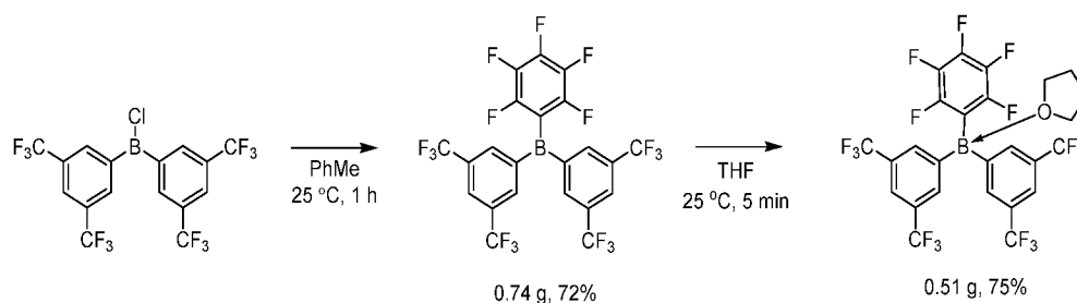
Schematic 7
