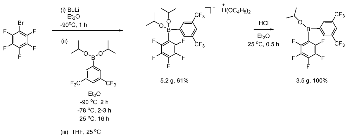
Schematic 4
