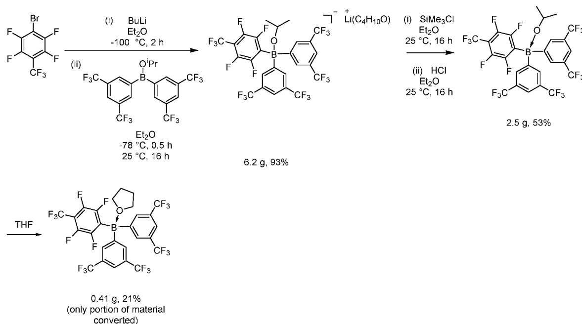
Schematic 18
