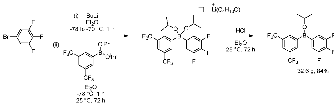
Schematic 5
