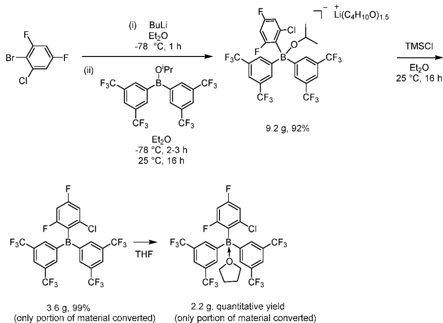
Schematic 11
