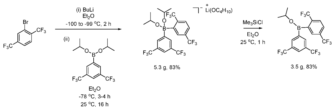
Schematic 6
