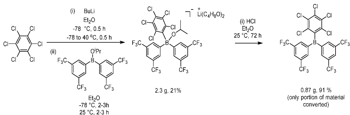
Schematic 15
