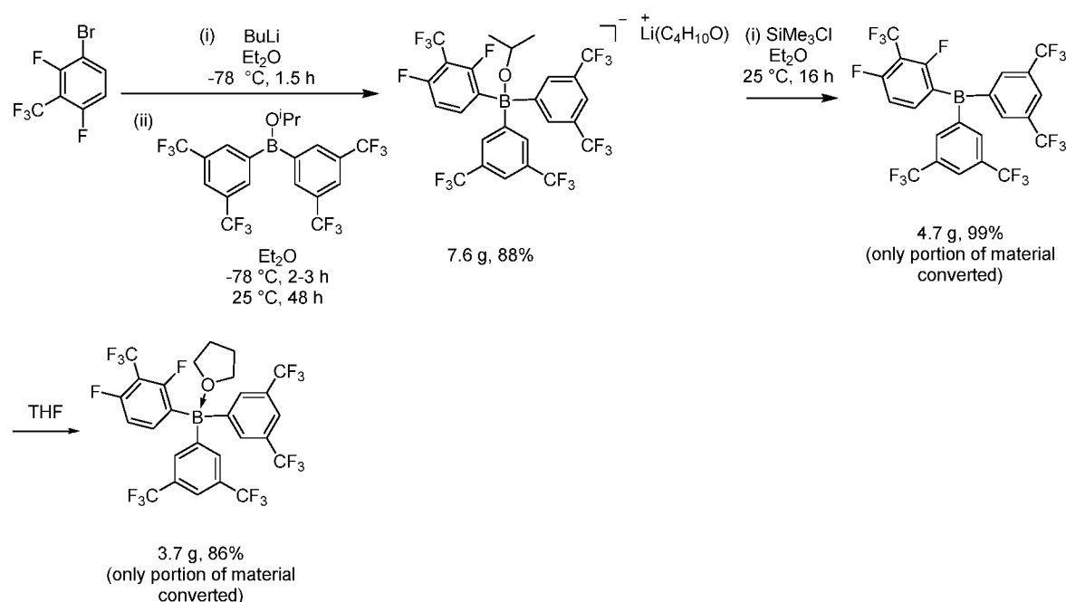
Schematic 19
