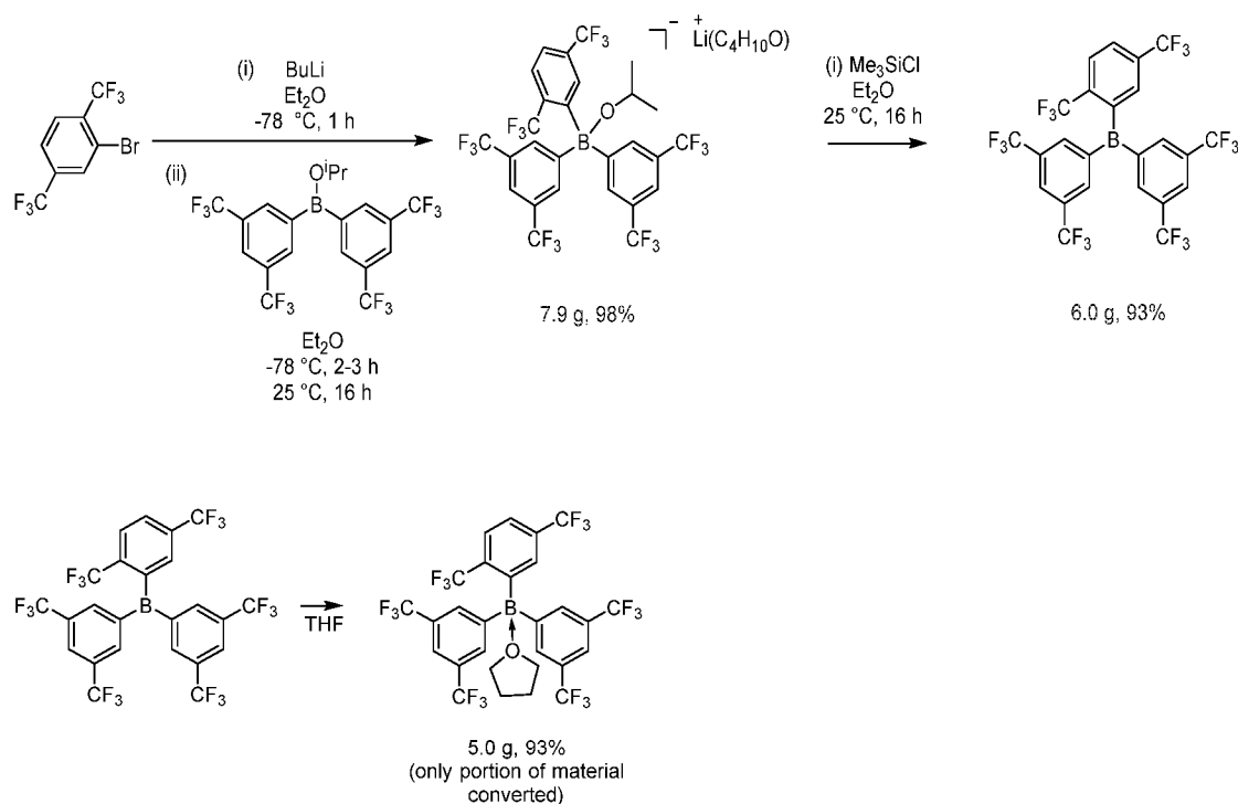
Schematic 16
