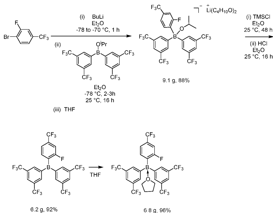
Schematic 14
