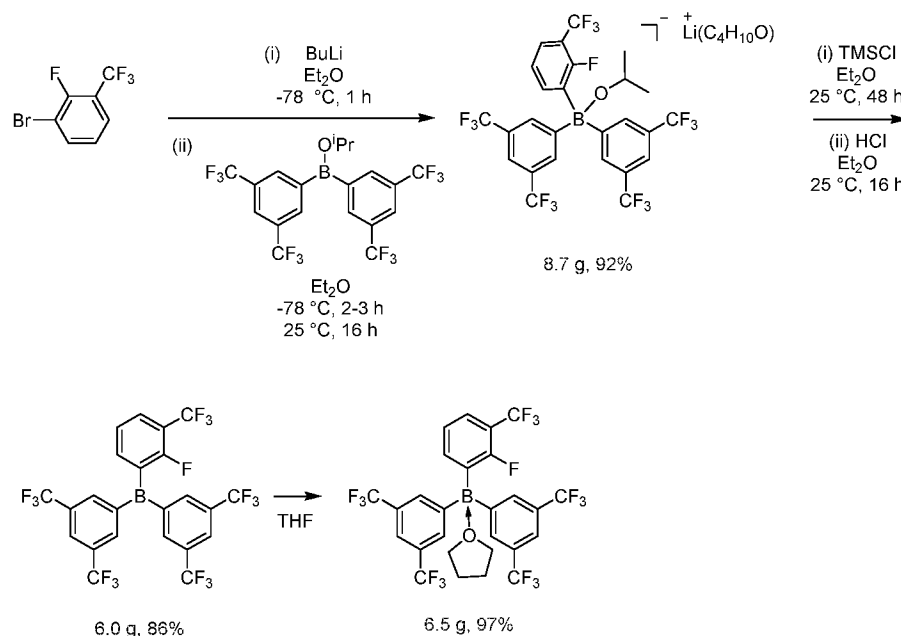
Schematic 13
