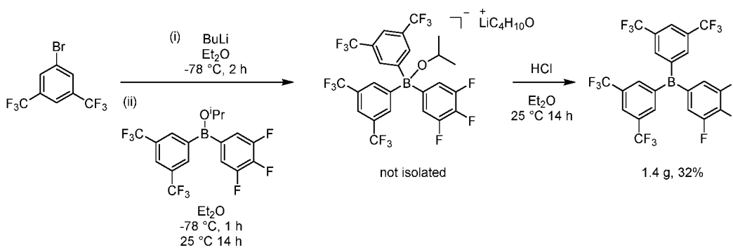
Schematic 9
