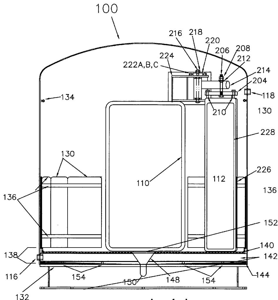
cross-sectional view with door open
