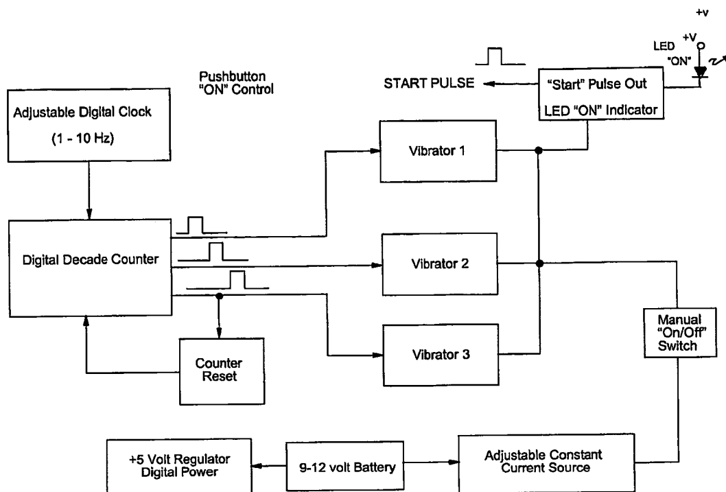
BLOCK DIAGRAM VIBRO-TACTILE STIMULATOR
