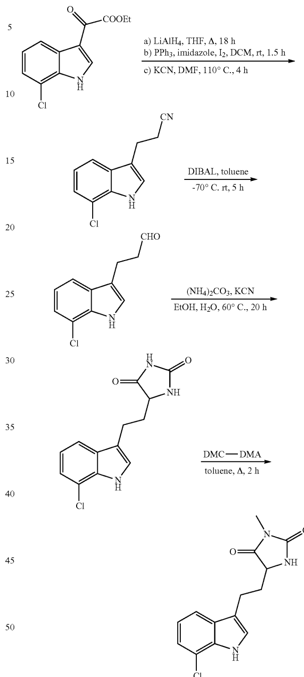
Comparative Reaction Scheme 2
