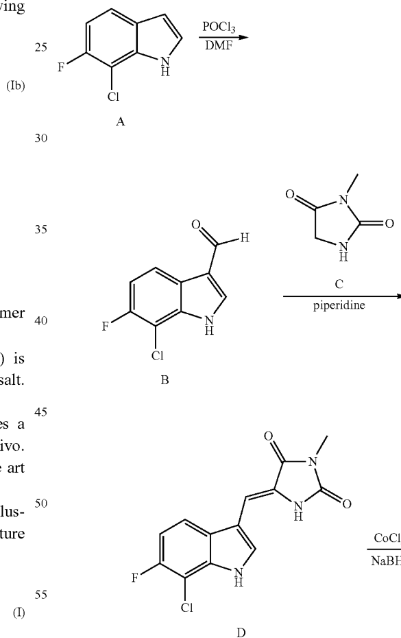
General Reaction Scheme I
