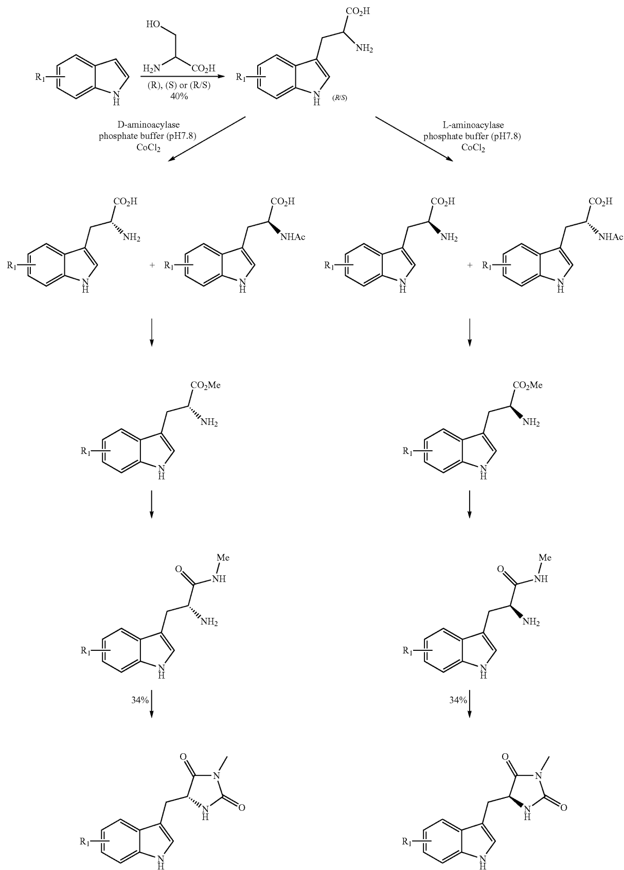
Comparative Reaction Scheme 3
