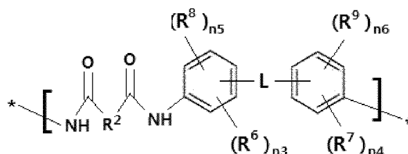
Chemical Formula 2
