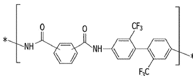
Chemical Formula 2b
