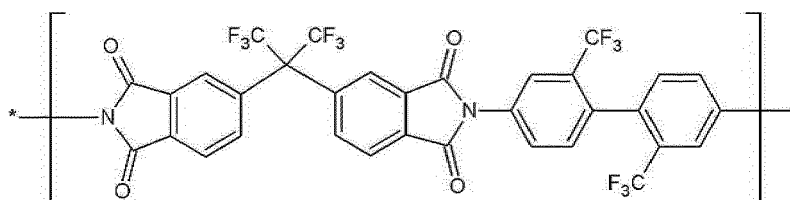
Chemical Formula 3a
