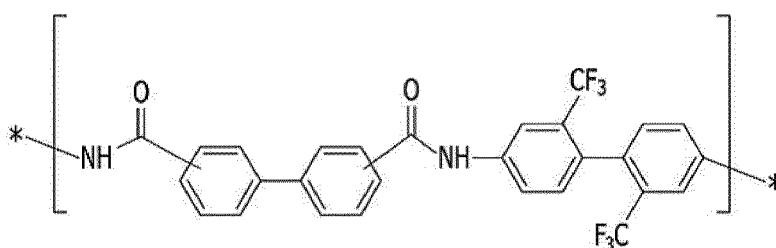
Chemical Formula 2b
