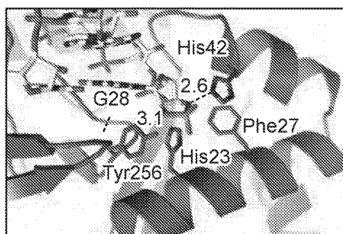
TtCas6B + repeat R3 RNA product
