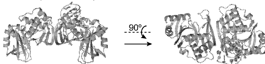
B TtCas6A + repeat R1 RNA product
