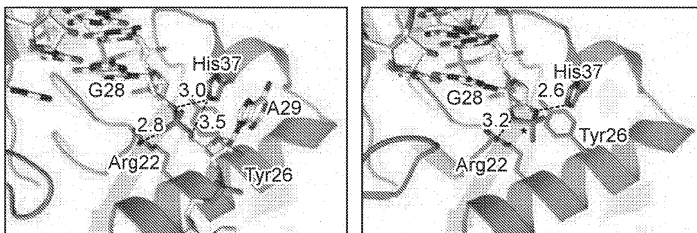
TtCas6A + repeat R1 RNA Substrate mimic
