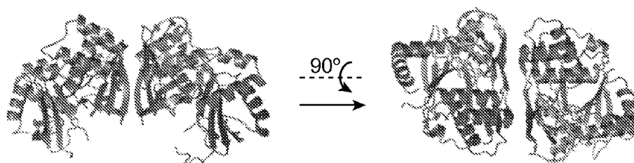
C TtCas6B + repeat R3 RNA product
