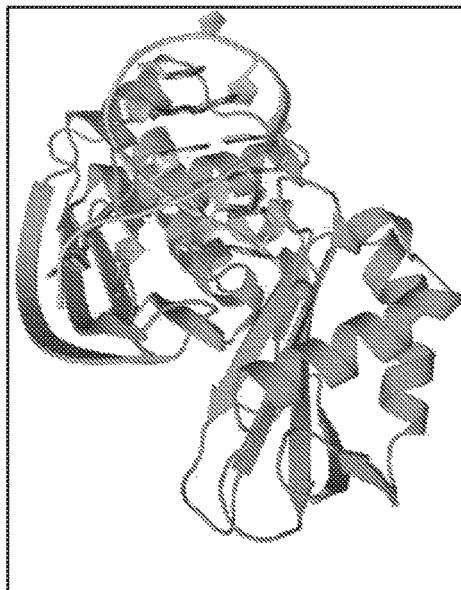
TtCas6A + repeat R1 RNA product
