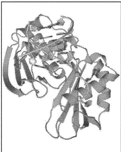
TtCas6A + repeat R1 RNA substrate mimic
