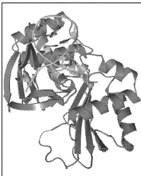
TtCas6B + repeat R3 RNA product
