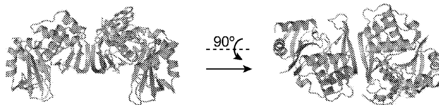
A TtCas6A + repeat R1 RNA substrate mimic
