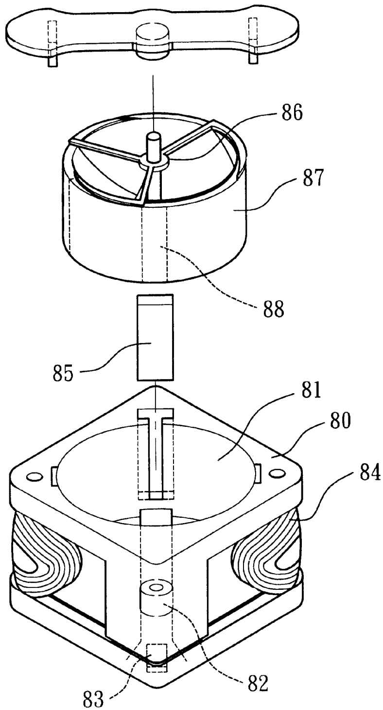
FIG. 6 PRIOR ART
