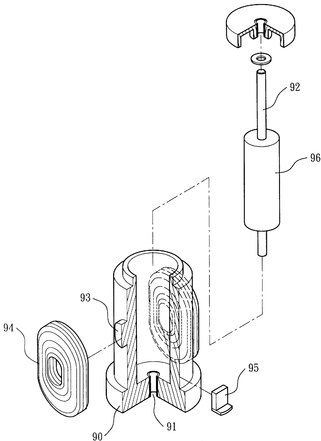
FIG. 5 PRIOR ART
