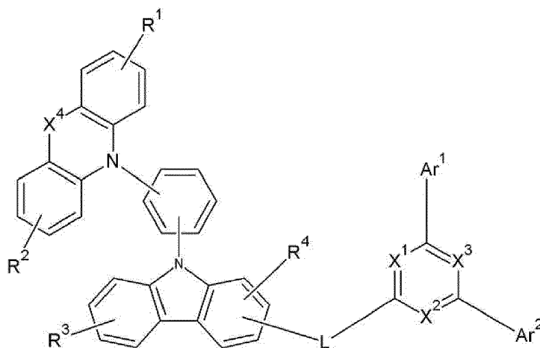
Chemical Formula 1
