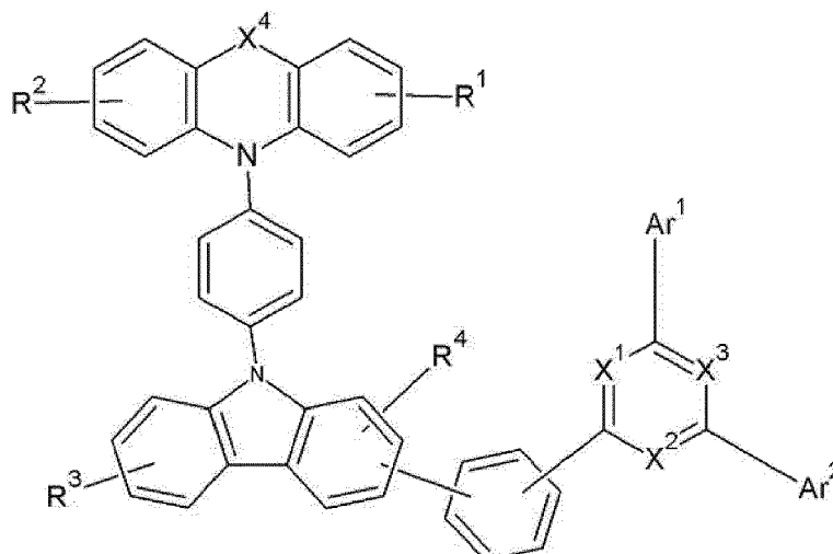
Chemical Formula 3
