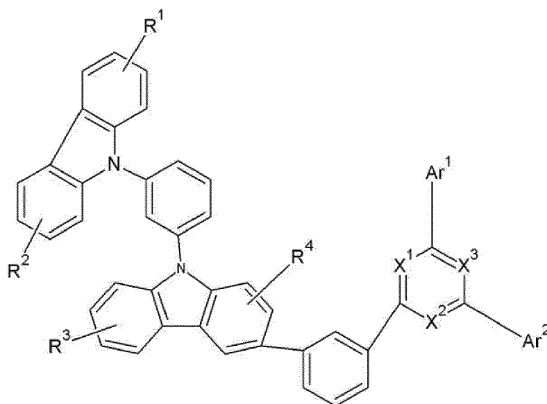
Chemical Formula 6
