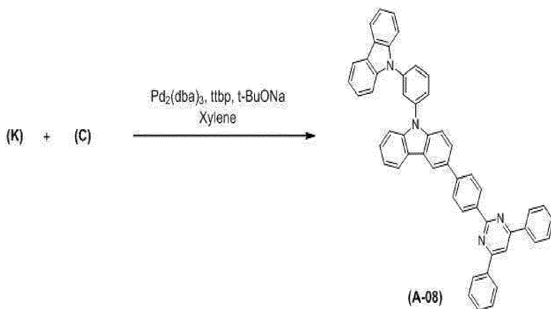
Reaction Scheme 8
