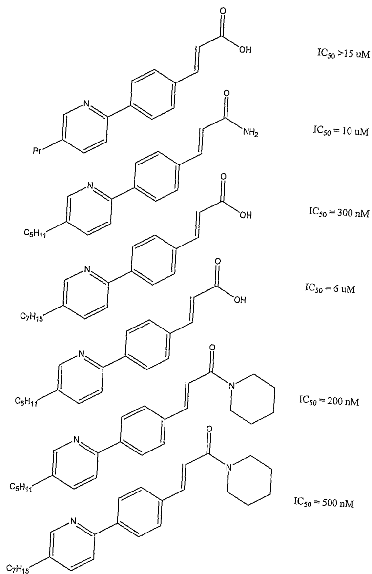
Scheme 4
