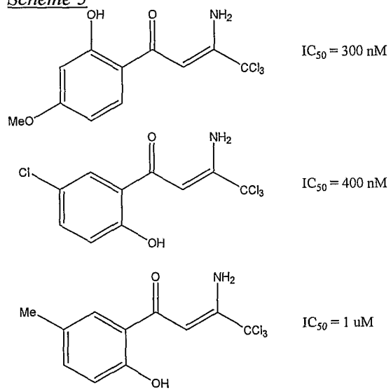
Scheme 5
