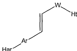
Formula IV
