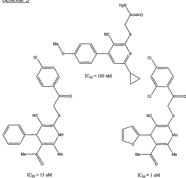
Scheme 3
