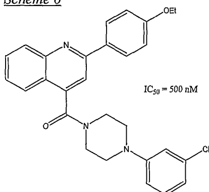
Scheme 6
