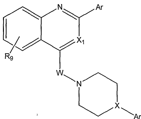
Formula VI
