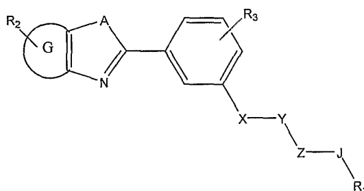
Formula VIIa
