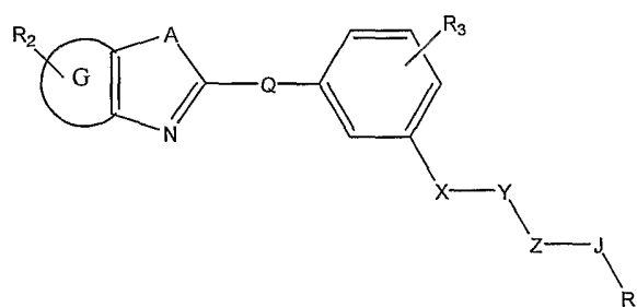
Formula VIIc
