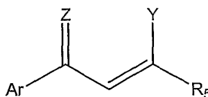
Formula V
