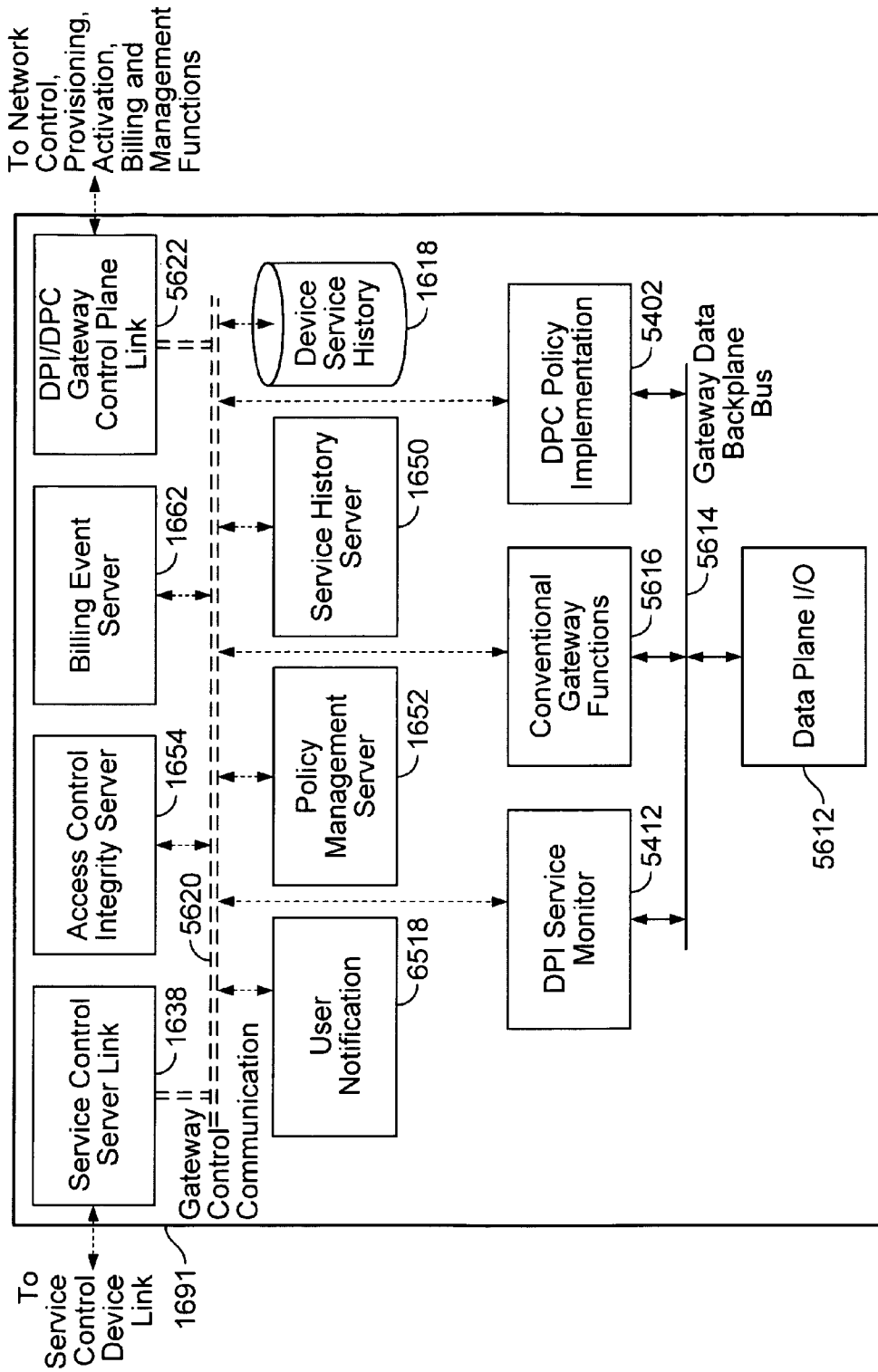
4G/3G/2G DPI/DPC Gateway 5610 FIG. 56
