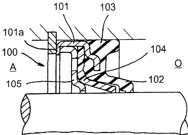
FIG. 23 (PRIOR ART)
