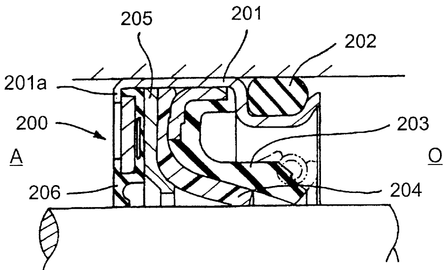
FIG. 24 (PRIOR ART)
