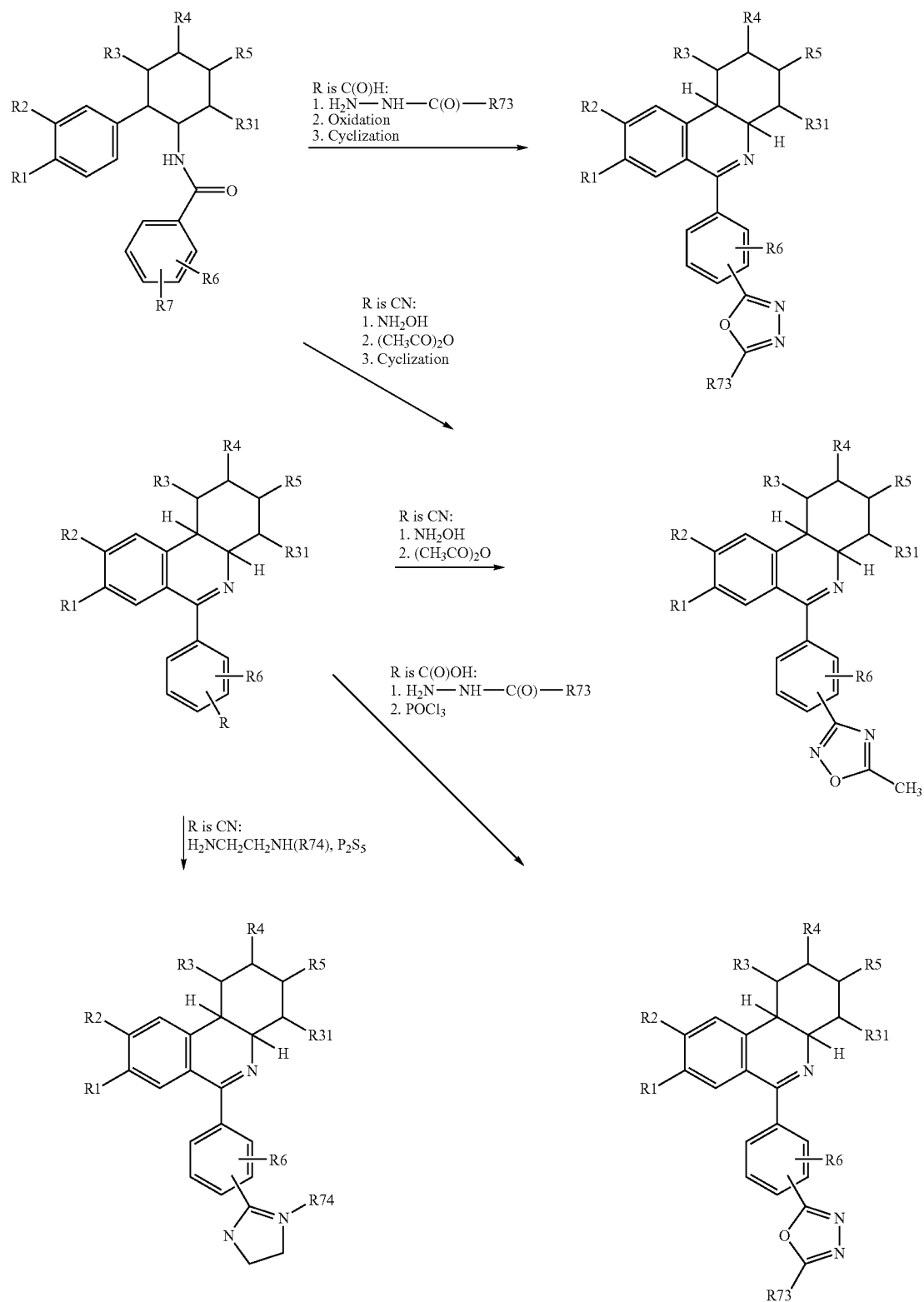
Reaction scheme 7:
