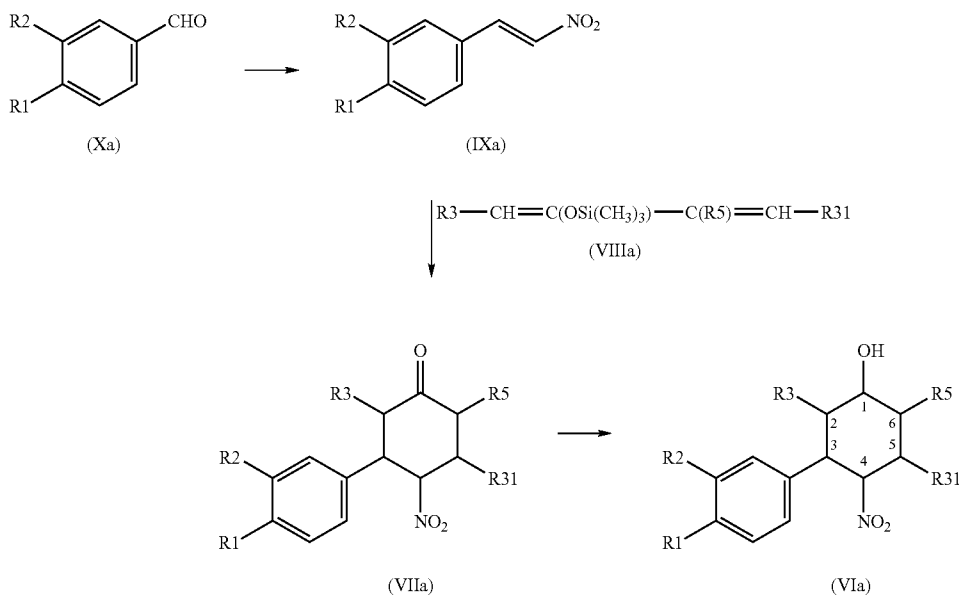
Reaction scheme 2:
