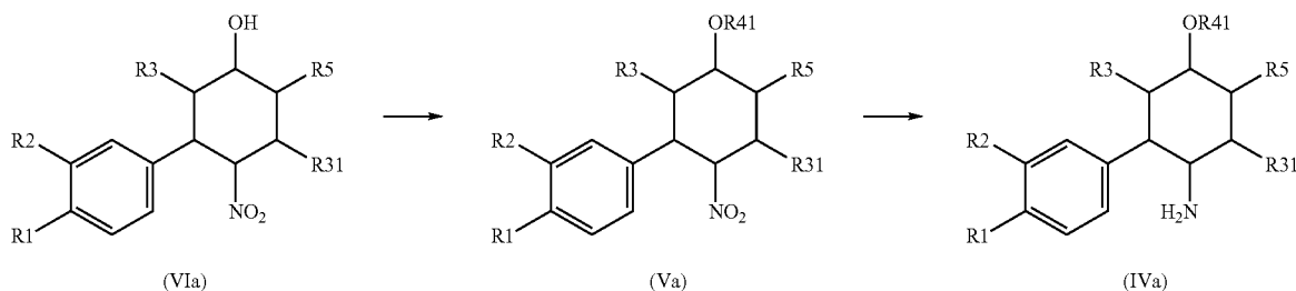
Reaction scheme 1:
