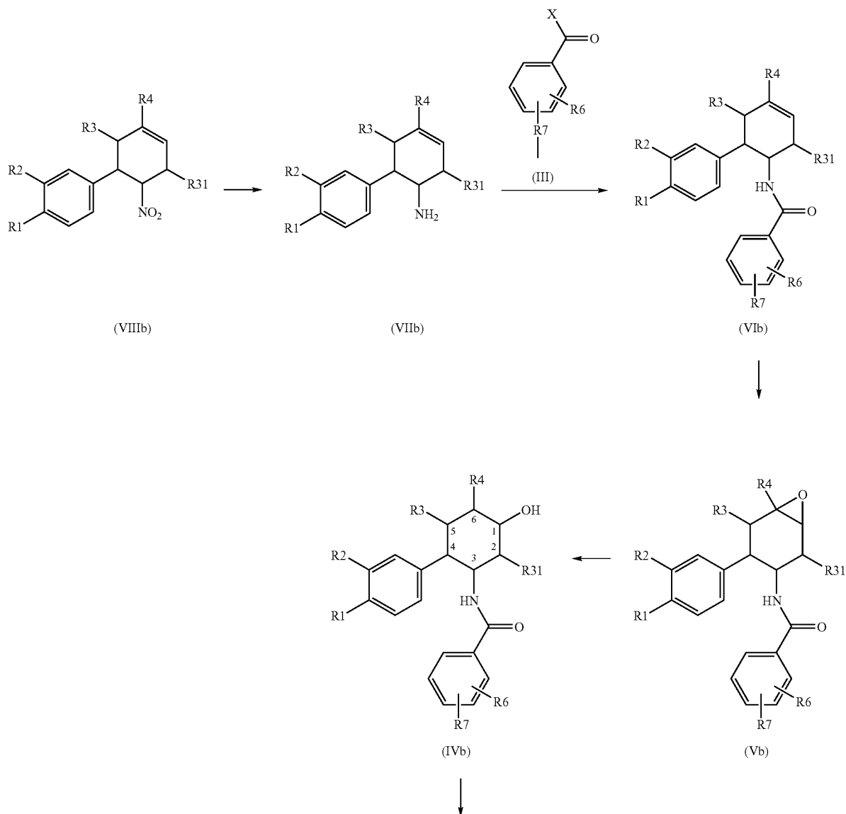
Reaction scheme 3:
