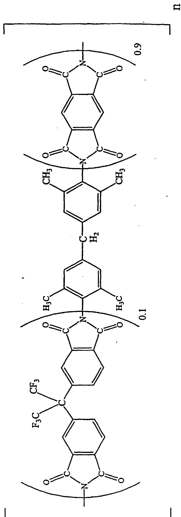
poly(PMDA/6FDA+TMMDA)imide
