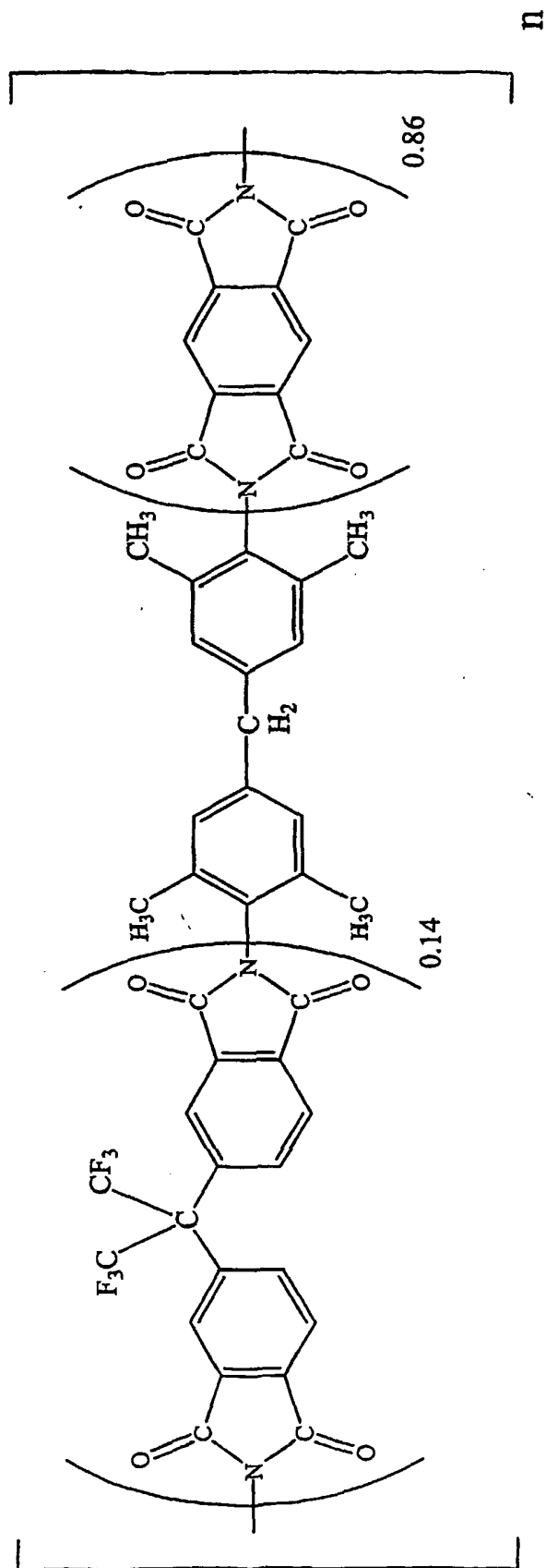
poly(PMDA/6FDA+TMMDA)imide
