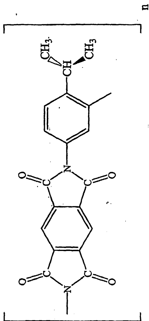
poly(PMDA+4-isopropyl-m-phenylenediamine)imide
