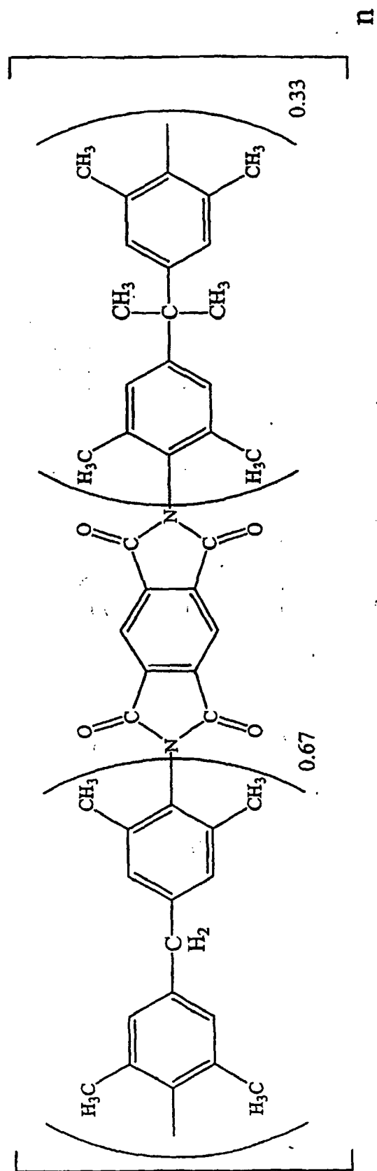
poly(PMDA+TMMDA/TMPDA)imide
