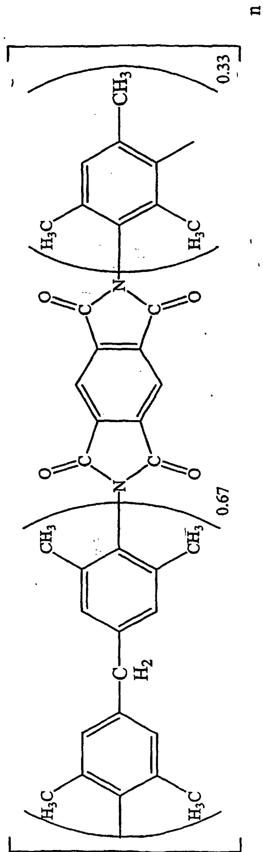
poly(PMDA+TMMDA/DAMs)imide
