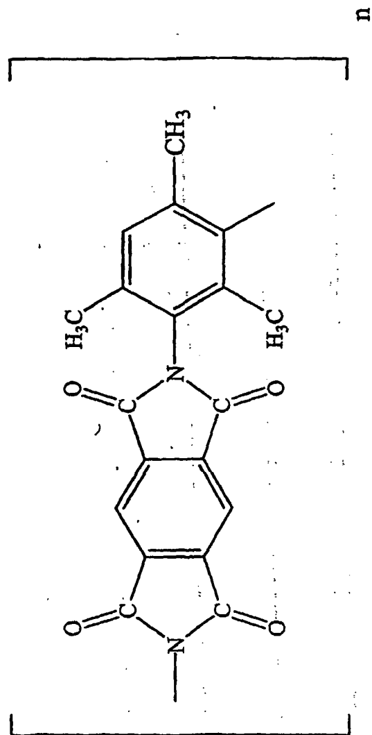
poly(PMDA+DAMs)imide
