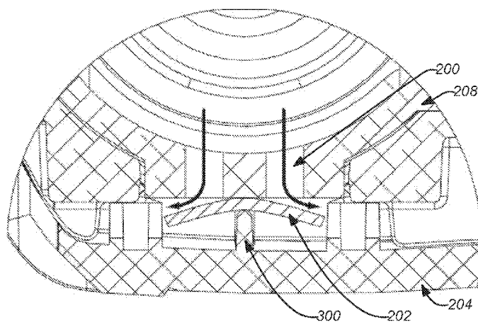
DETAIL C
