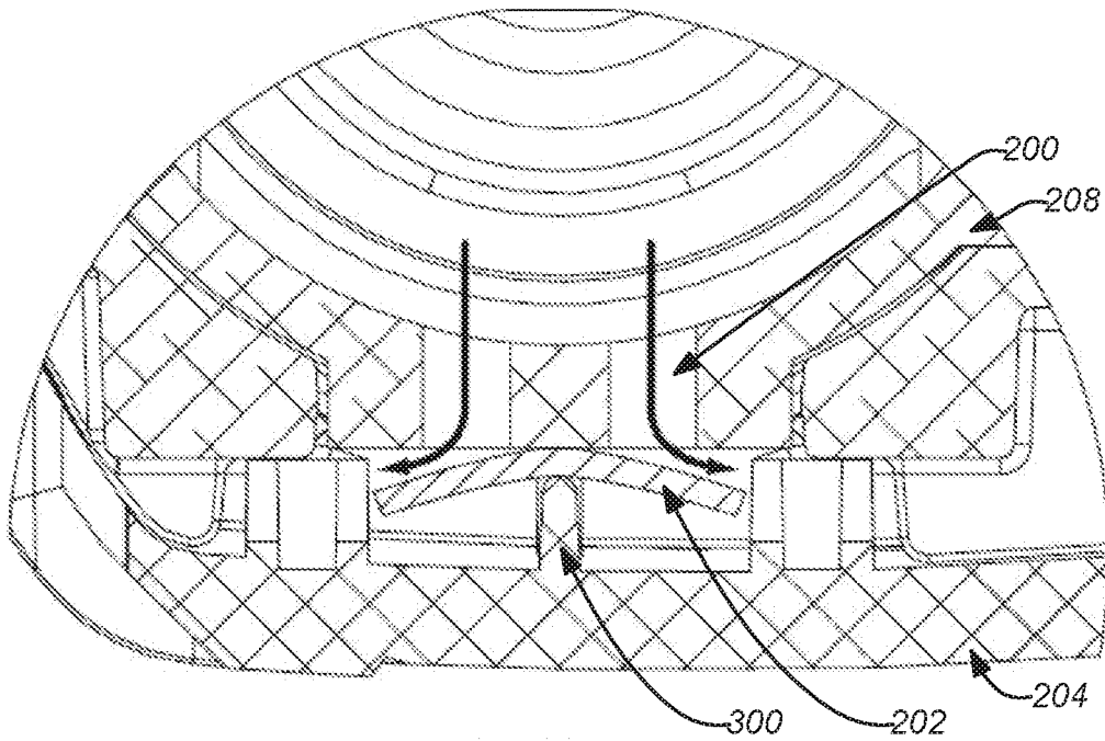
DETAIL C
