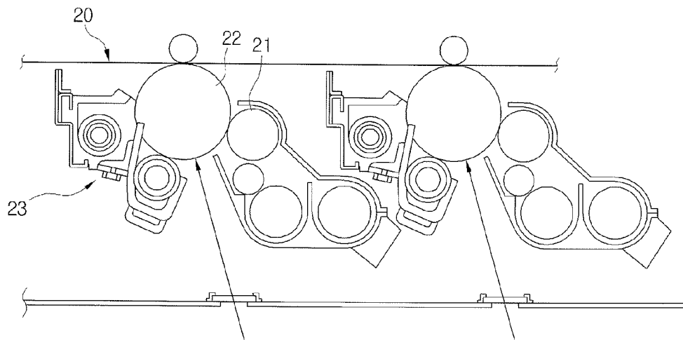
FIG. 2 (PRIOR ART)
