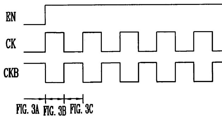
FIG. 2 (PRIOR ART)
