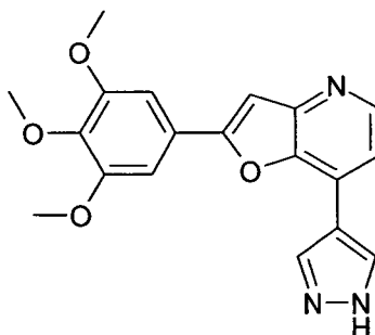
7-(1H-Pyrazol-4-yl)-2-(3,4,5-trimethoxy-phenyl)-furo[3,2-b]pyridine
