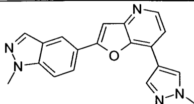
2-(1-Methyl-1H-indazol-5-yl)-7-(1-methyl-1H-pyrazol-4-yl)- furo[3,2-b]pyridine
