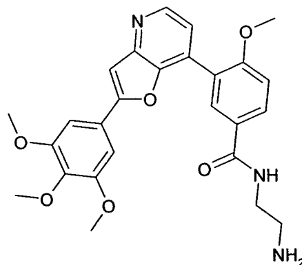
N-(2-Amino-ethyl)-4-methoxy-3-[2-(3,4,5-trimethoxy-phenyl)-furo[3,2-b]pyridin-7-yl]-benzamide
