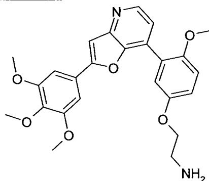
2-{4-Methoxy-3-[2-(3,4,5-trimethoxy-phenyl)-furo[3,2-b]pyridin-7-yl]-phenoxy}-ethylamine
