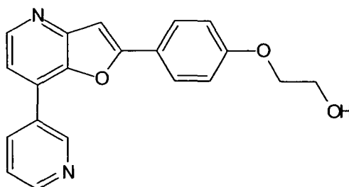
2-[4-(7-Pyridin-3-yl-furo[3,2-b]pyridin-2-yl)-phenoxy]-ethanol
