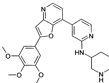
Piperidin-3-yl-{4-[2-(3,4,5-trimethoxy-phenyl)-furo[3,2-b]pyridin- 7-yl]-pyridin-2-yl}-amine
