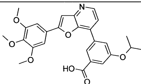
3-Isopropoxy-5-[2-(3,4,5-trimethoxy-phenyl)-furo[3,2-b]pyridin-7-yl]-benzoic acid
