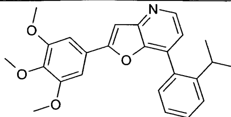
7-(2-Isopropyl-phenyl)-2-(3,4,5-trimethoxy-phenyl)-furo[3,2-b]pyridine
