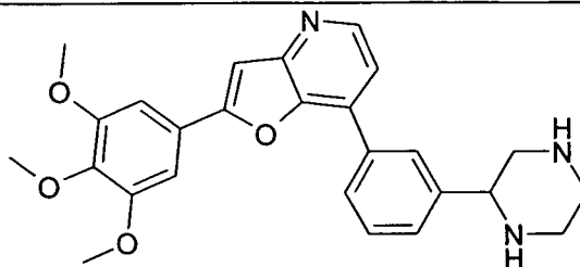
7-(3-Piperazin-2-yl-phenyl)-2-(3,4,5-trimethoxy-phenyl)- furo[3,2-b]pyridine
