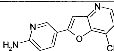
5-(7-Chloro-furo[3,2-b]pyridin-2-yl)-pyridin-2-ylamine
