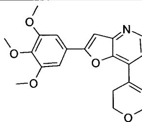
7-(3,6-Dihydro-2H-pyran-4-yl)-2-(3,4,5-trimethoxy-phenyl)- furo[3,2-b]pyridine
