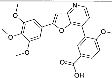
4-Methoxy-3-[2-(3,4,5-trimethoxy-phenyl)-furo[3,2-b]pyridin-7-yl]-benzoic acid
