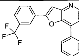
7-Phenyl-2-(3-trifluoromethyl-phenyl)-furo[3,2-b]pyridine
