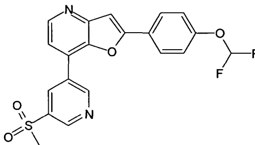
2-(4-Difluoromethoxy-phenyl)-7-(5-methanesulfonyl-pyridin-3- yl)-furo[3,2-b]pyridine
