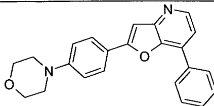
2-(4-Morpholin-4-yl-phenyl)-7-phenyl-furo[3,2-b]pyridine
