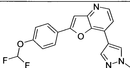
2-(4-Difluoromethoxy-phenyl)-7-(1-methyl-1H-pyrazol-4-yl)-furo[3,2-b]pyridine
