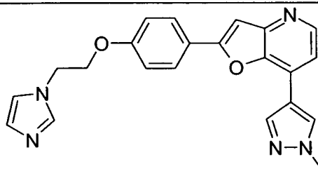
2-[4-(2-Imidazol-1-yl-ethoxy)-phenyl]-7-(1-methyl-1H-pyrazol-4-yl)-furo[3,2-b]pyridine
