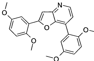
2,7-Bis-(2,5-dimethoxy-phenyl)-furo[3,2-b]pyridine
