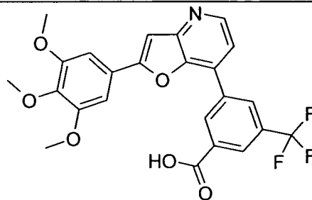
3-Trifluoromethyl-5-[2-(3,4,5-trimethoxy-phenyl)-furo[3,2-b]pyridin-7-yl]-benzoic acid
