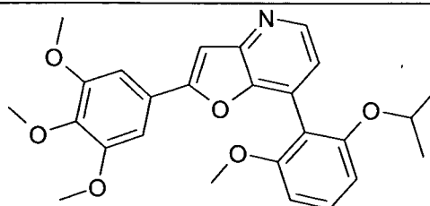
7-(2-Isopropoxy-6-methoxy-phenyl)-2-(3,4,5-trimethoxy-phenyl)-furo[3,2-b]pyridine
