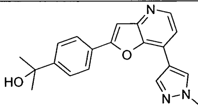
2-{4-[7-(1-Methyl-1H-pyrazol-4-yl)-furo[3,2-b]pyridin-2-yl]- phenyl}-propan-2-ol
