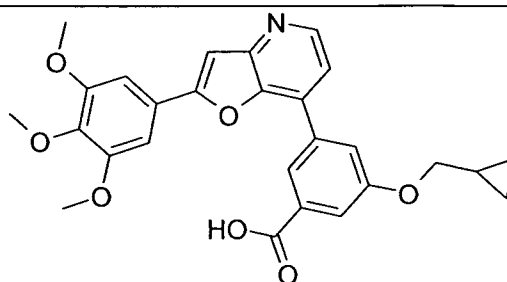
3-Cyclopropylmethoxy-5-[2-(3,4,5-trimethoxy-phenyl)-furo[3,2-b]pyridin-7-yl]-benzoic acid
