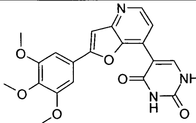
5-[2-(3,4,5-Trimethoxy-phenyl)-furo[3,2-b]pyridin-7-yl]-1H- pyrimidine-2,4-dione
