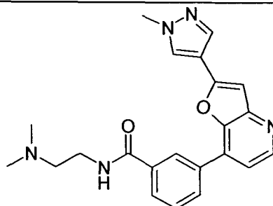
N-(2-Dimethylamino-ethyl)-3-[2-(1-methyl-1H-pyrazol-4-yl)- furo[3,2-b]pyridin-7-yl]-benzamide
