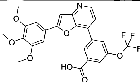
3-Trifluoromethoxy-5-[2-(3,4,5-trimethoxy-phenyl)-furo[3,2-b]pyridin-7-yl]-benzoic acid
