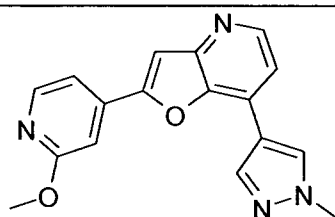
2-(2-Methoxy-pyridin-4-yl)-7-(1-methyl-1H-pyrazol-4-yl)- furo[3,2-b]pyridine
