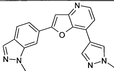
2-(1-Methyl-1H-indazol-6-yl)-7-(1-methyl-1H-pyrazol-4-yl)- furo[3,2-b]pyridine
