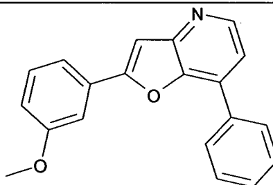
2-(3-Methoxy-phenyl)-7-phenyl-furo[3,2-b]pyridine
