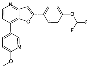
2-(4-Difluoromethoxy-phenyl)-7-(6-methoxy-pyridin-3-yl)- furo[3,2-b]pyridine
