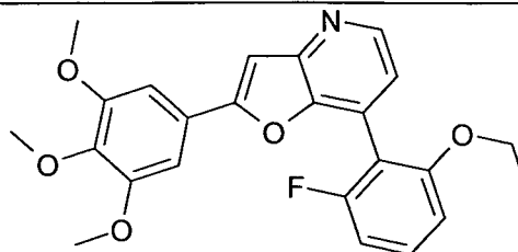
7-(2-Ethoxy-6-fluoro-phenyl)-2-(3,4,5-trimethoxy-phenyl)- furo[3,2-b]pyridine
