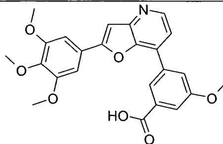
3-Methoxy-5-[2-(3,4,5-trimethoxy-phenyl)-furo[3,2-b]pyridin-7-yl]-benzoic acid
