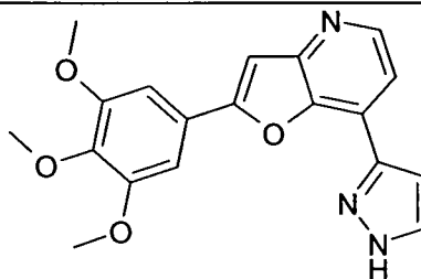
7-(1H-Pyrazol-3-yl)-2-(3,4,5-trimethoxy-phenyl)-furo[3,2-b]pyridine
