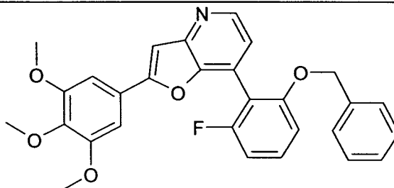
7-(2-Benzyloxy-6-fluoro-phenyl)-2-(3,4,5-trimethoxy-phenyl)- furo[3,2-b]pyridine
