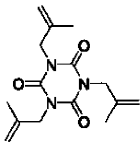
trimethallyl isocyanurate (TMAIC)
