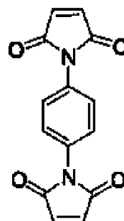
N,N'-phenylene bismaleimide
