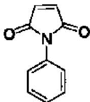
N-phenylene maleimide
