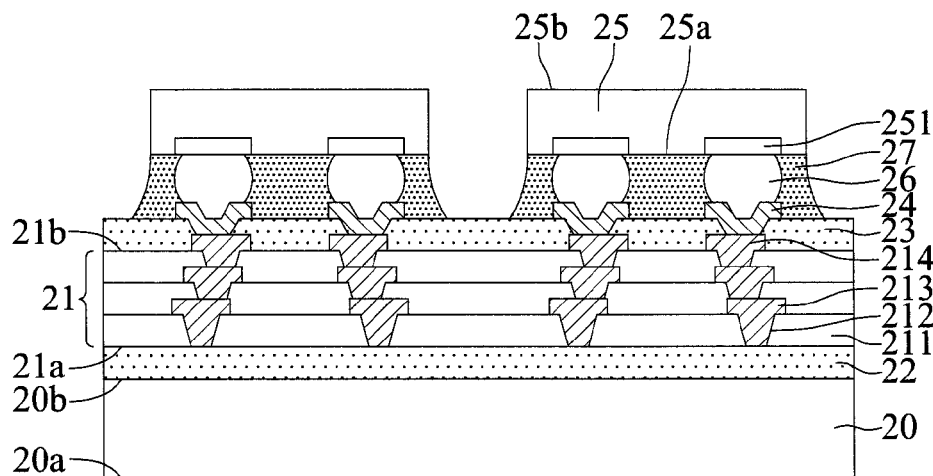
FIG. 2C (PRIOR ART)
