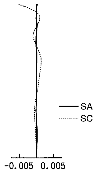
SPHERICAL ABERRATION, SINE CONDITION
