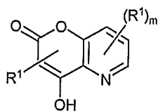
4-hydroxy-4a,8a-dihydro-pyrano[3,2,b]pyridin-2-one
