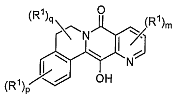
dibenzo[a,g]quinolizin-8-one
