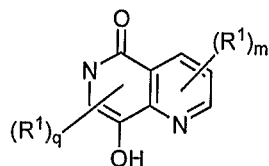
8-hydroxy-6H-[1,6]naphthyridin-5-one
