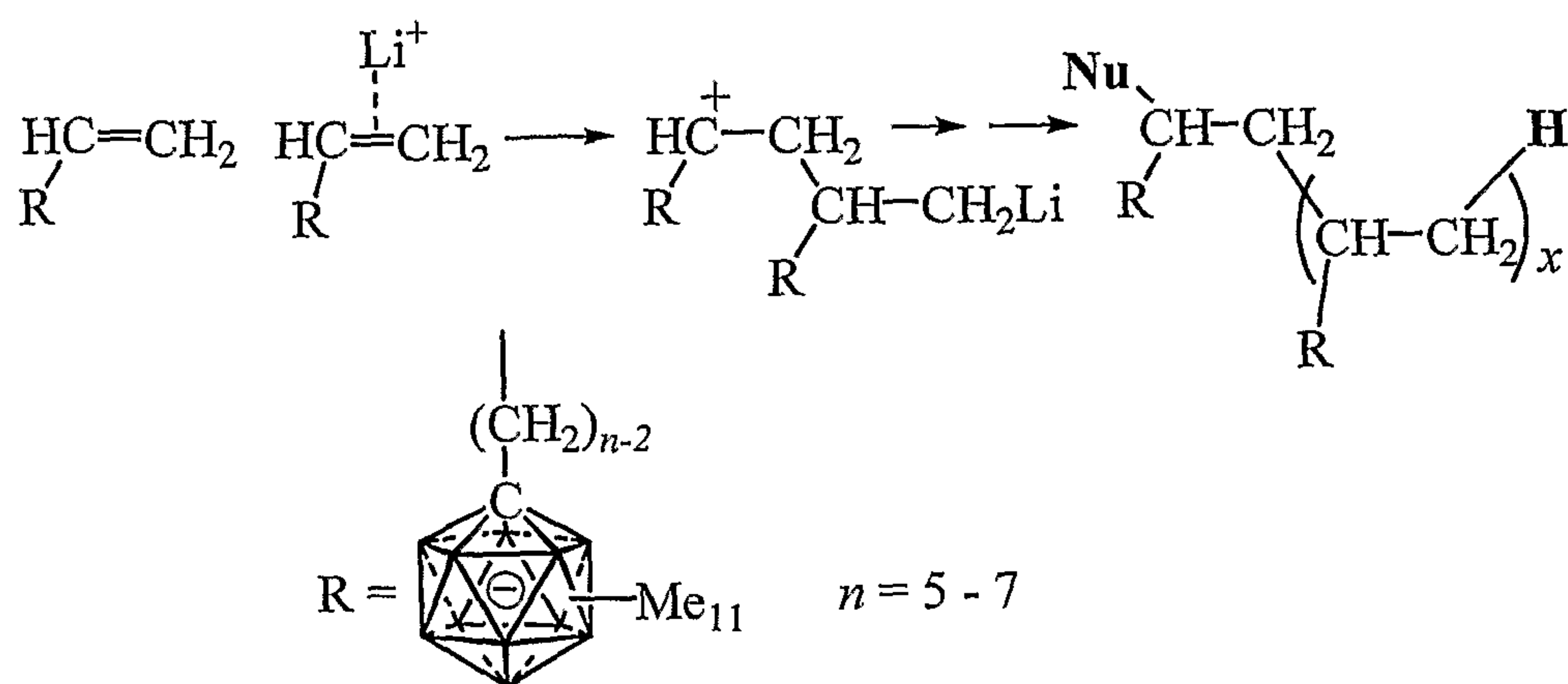
Scheme 4: A hypothetical mechanism for cationic polymerization of [n]2 , n = 5 - 7 .
