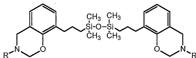
13 (R = t-Bu) and 14 (R = Ph)
