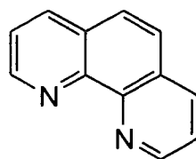
1,10-o-phenanthroline (4,5-diazaphenanthrene)
