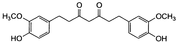
Tetrahydrocurcumin
