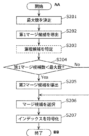
FIG. 19: S201 Determine the maximum number S202 Derive first merge candidates S203 Specify overlapping candidates S204 Number of first merge candidates < maximum number? S205 Derive second merge candidates S206 Select merge candidates S207 Encode index AA Start BB End
