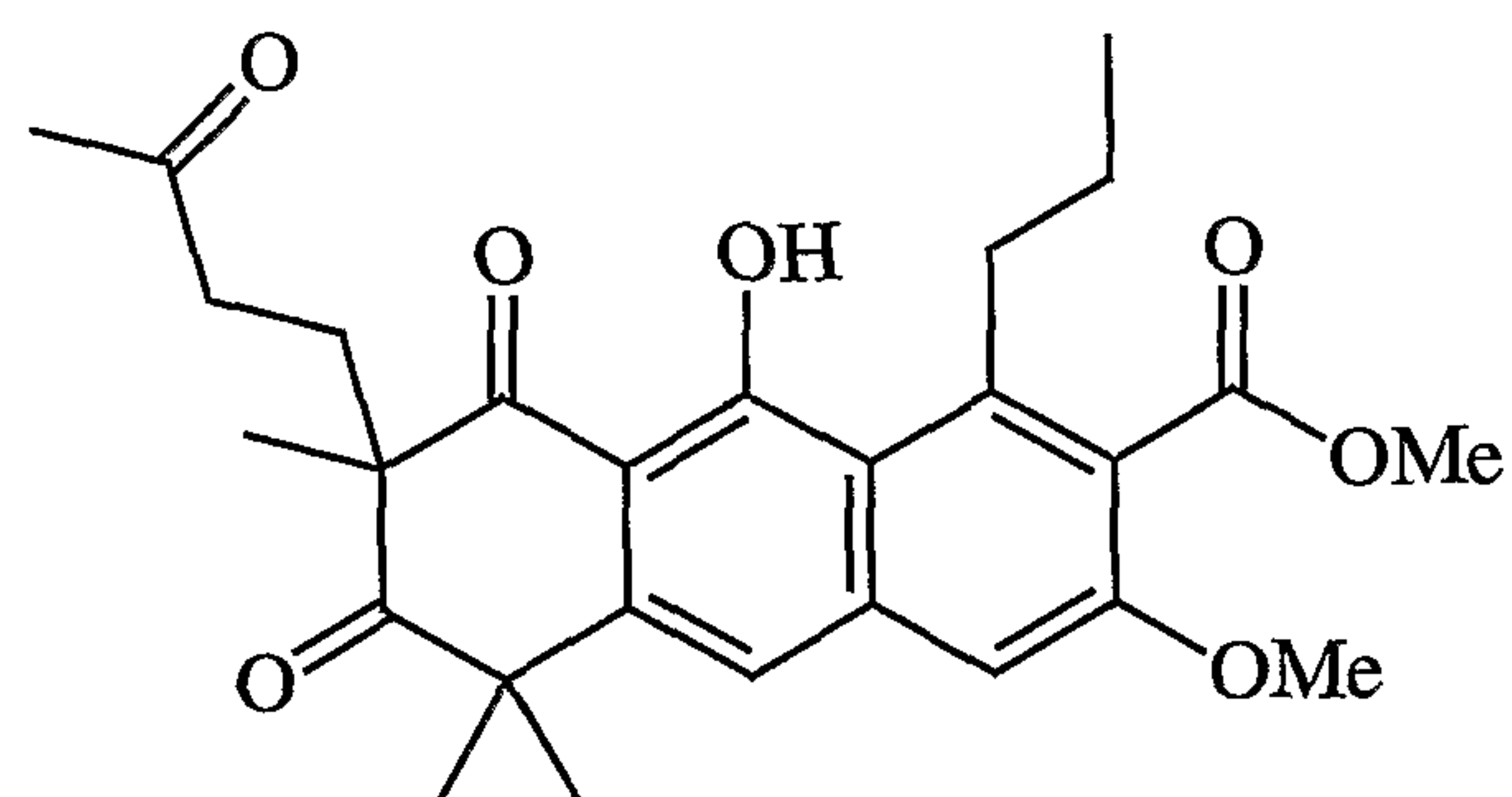
Garvalone B
