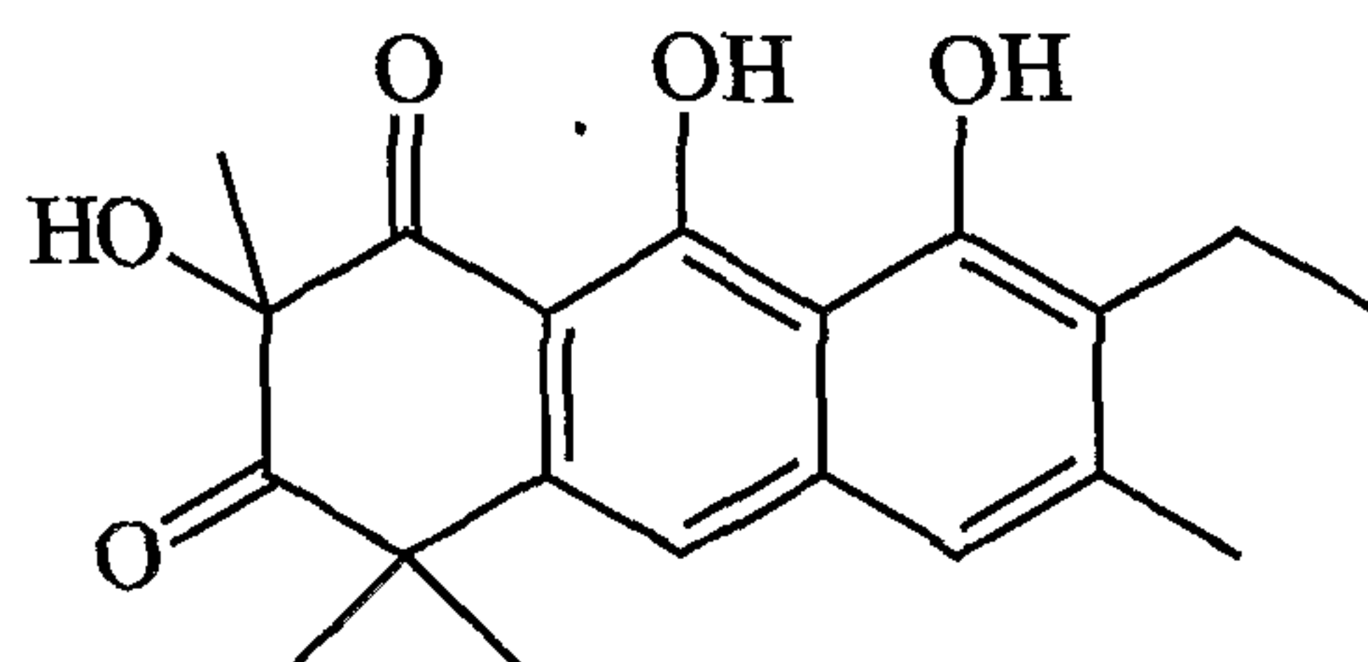
Garveatin F
