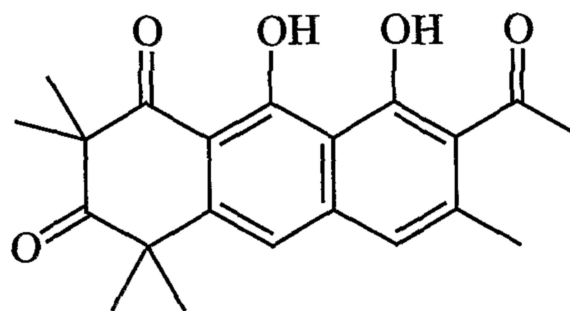
Garveatin D
