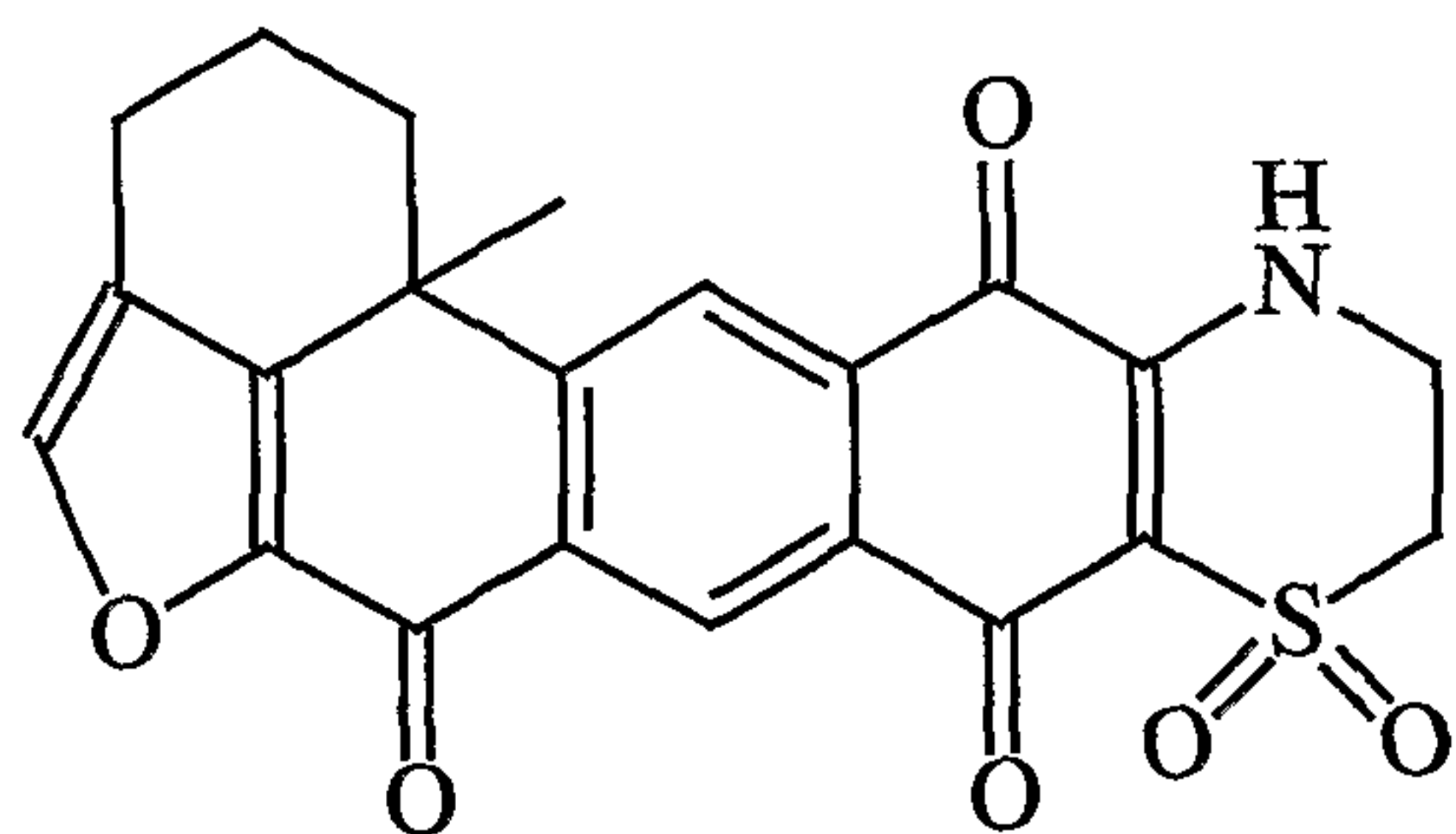
Adociaquinone A
