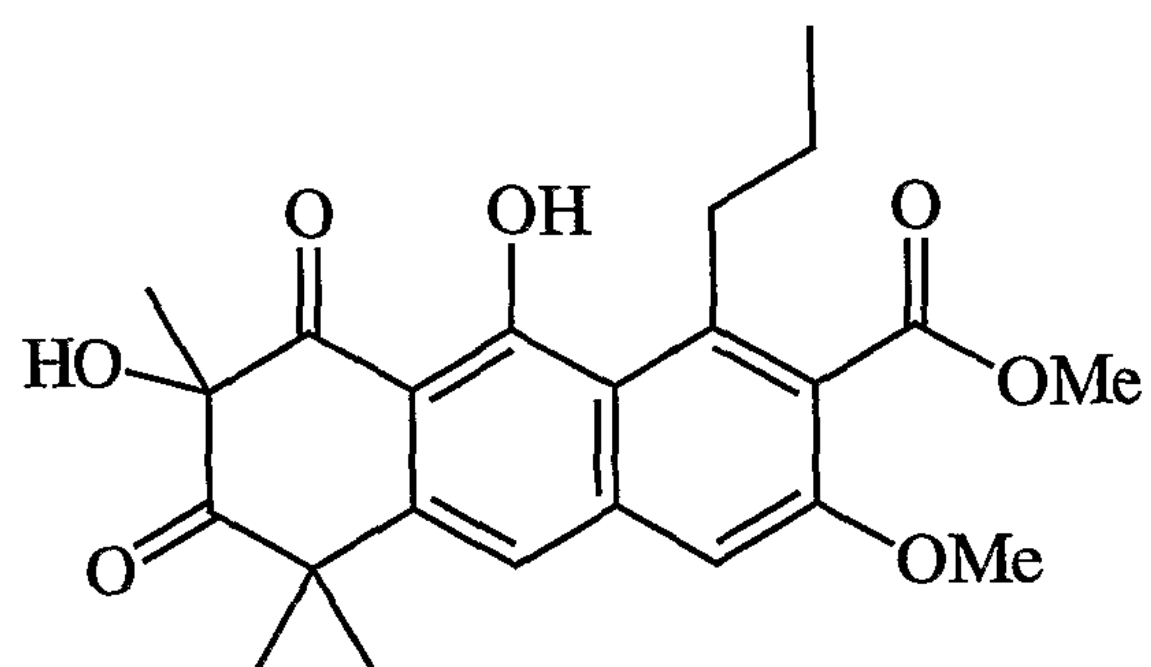
2-hydroxygarvin A
