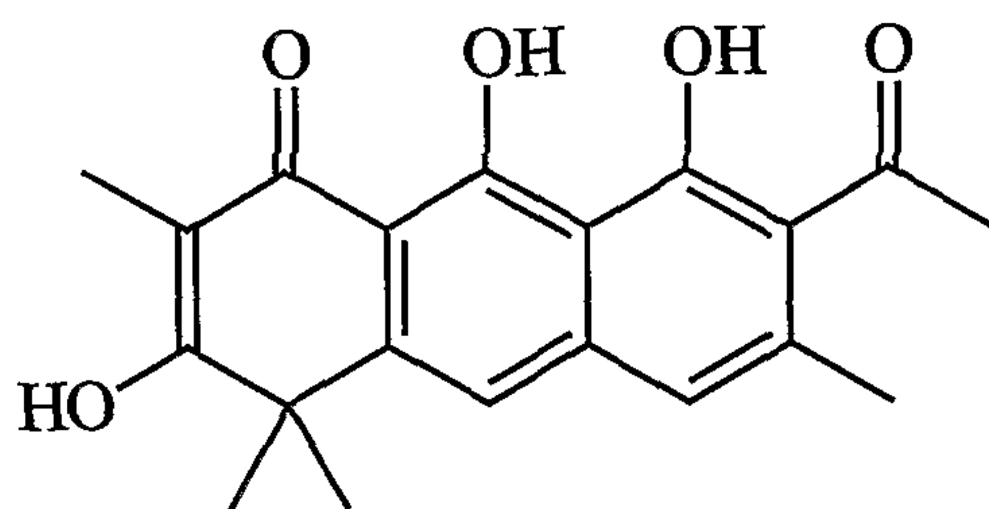
Garveatin A
