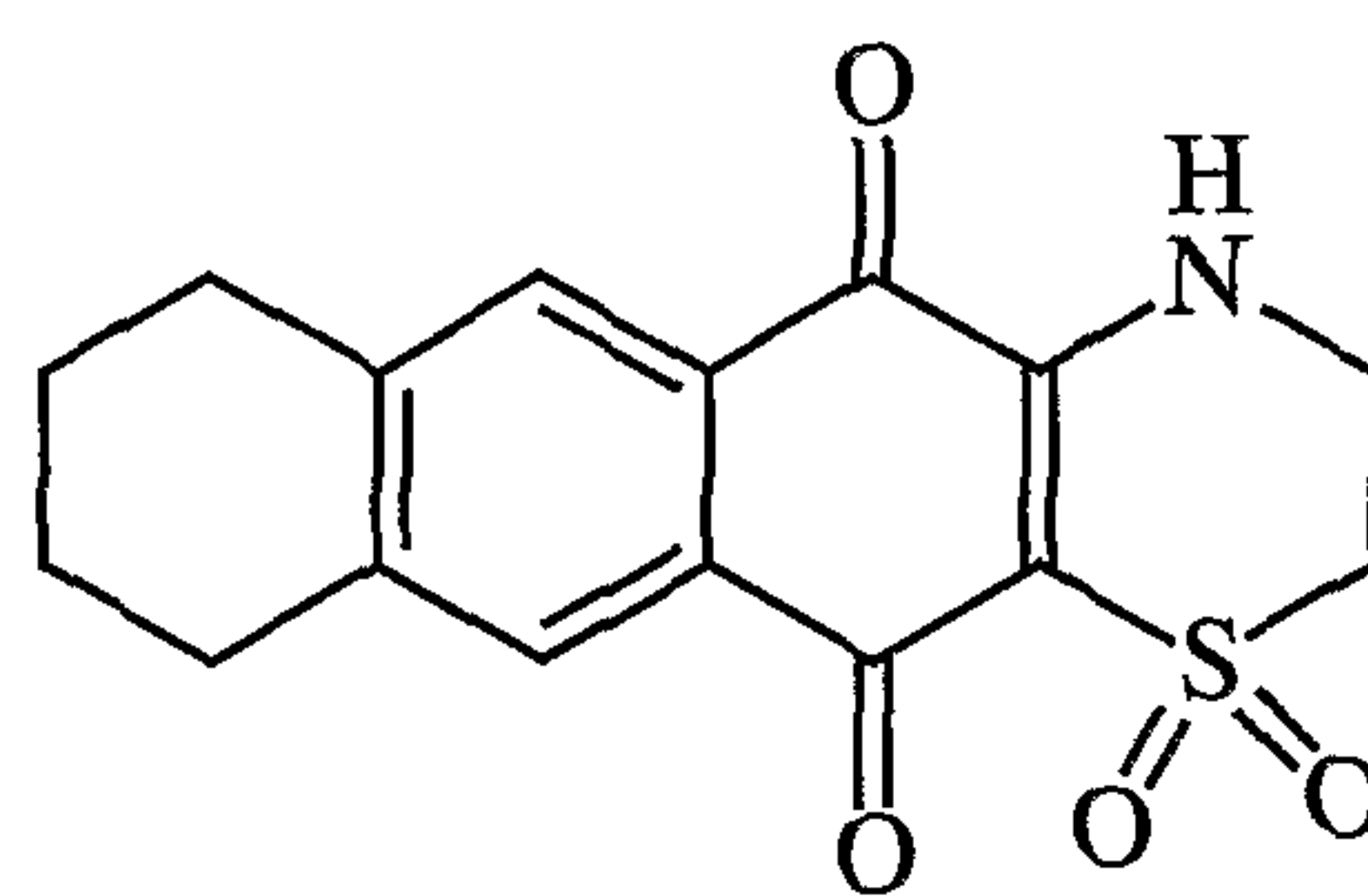
Garveatin F
