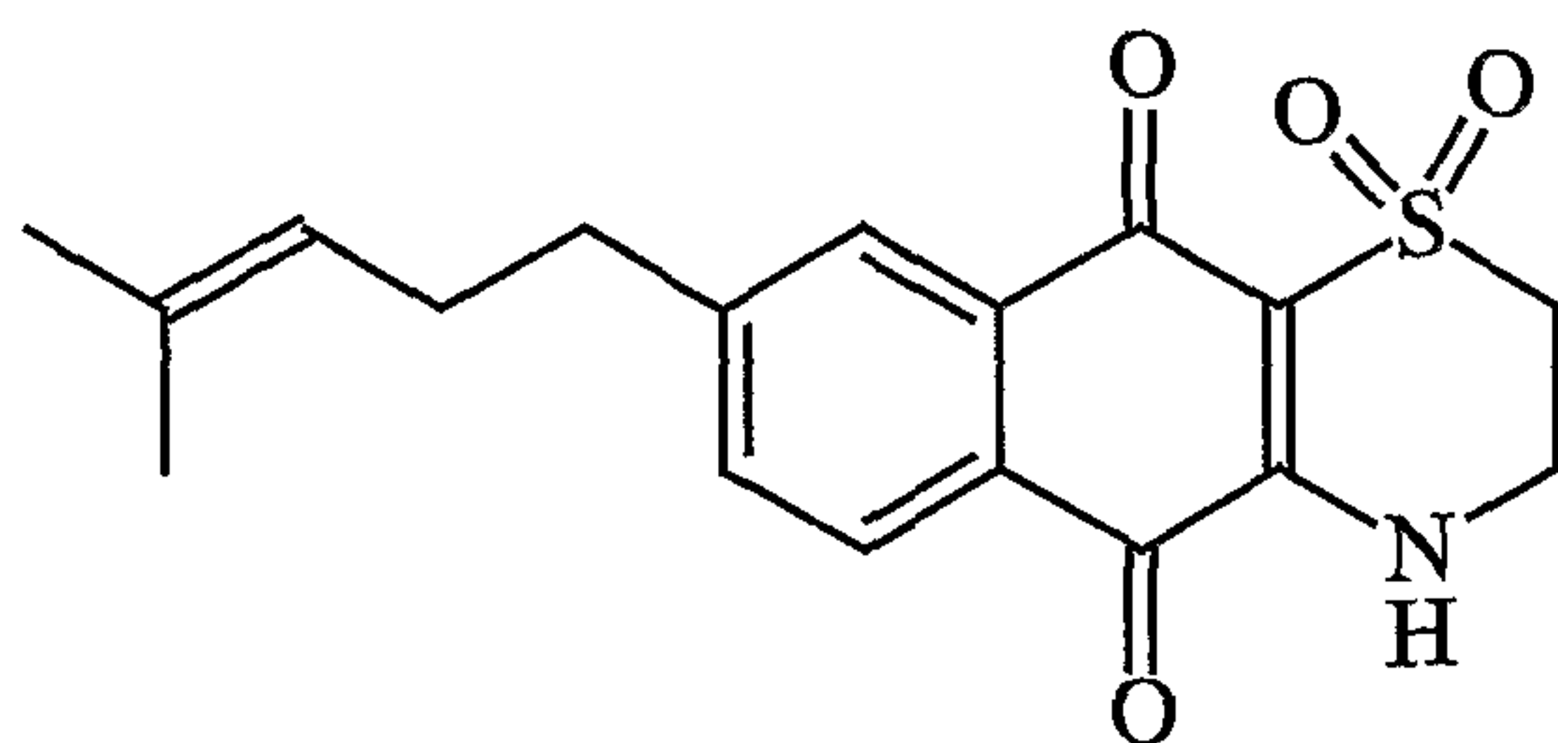
Conicaquinone A
