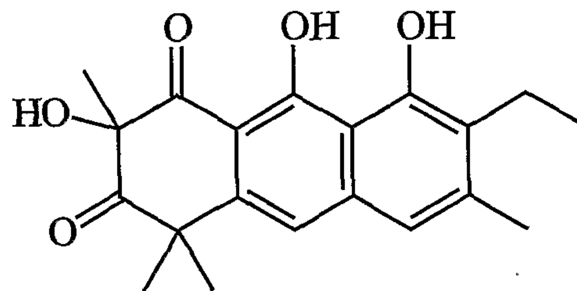
2-hydroxyGarveatin B
