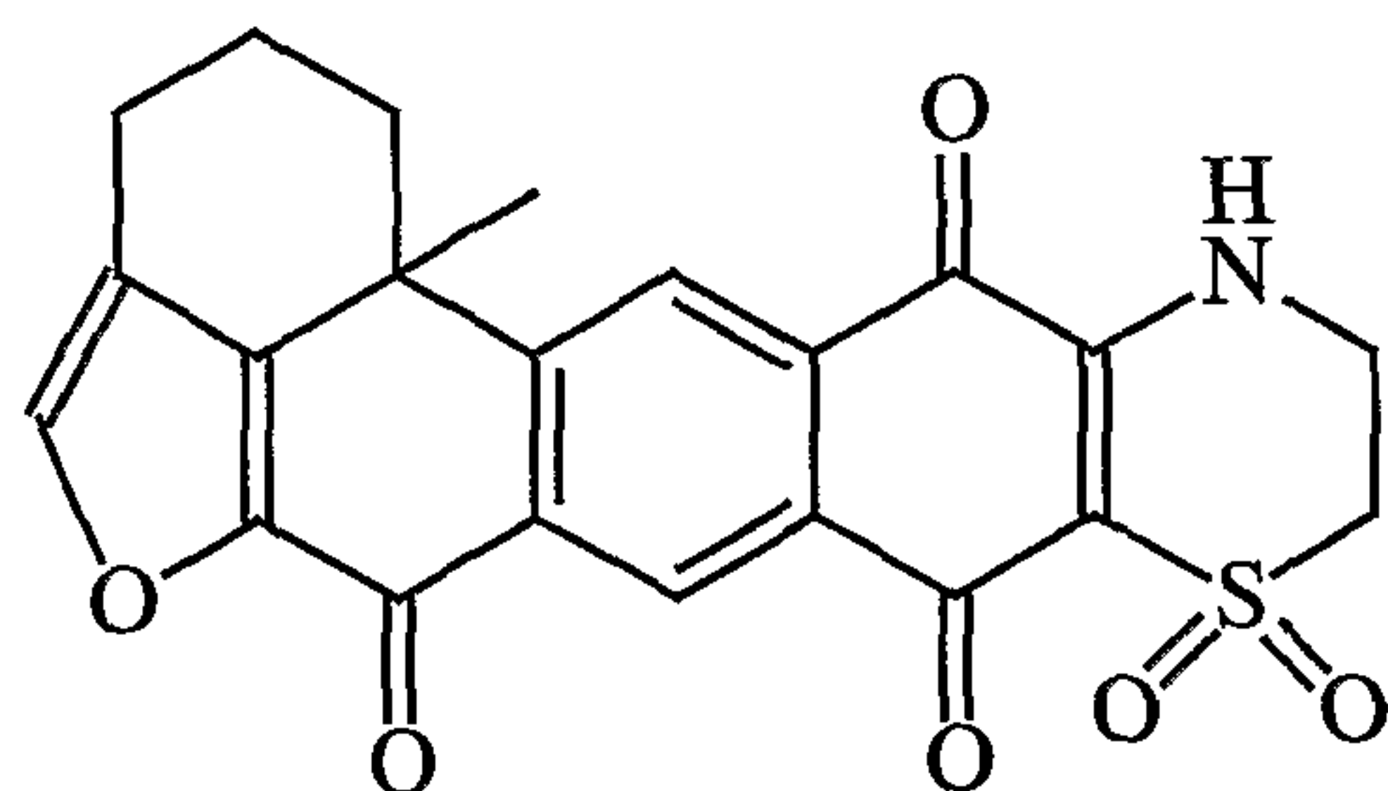
Adociaquinone A
