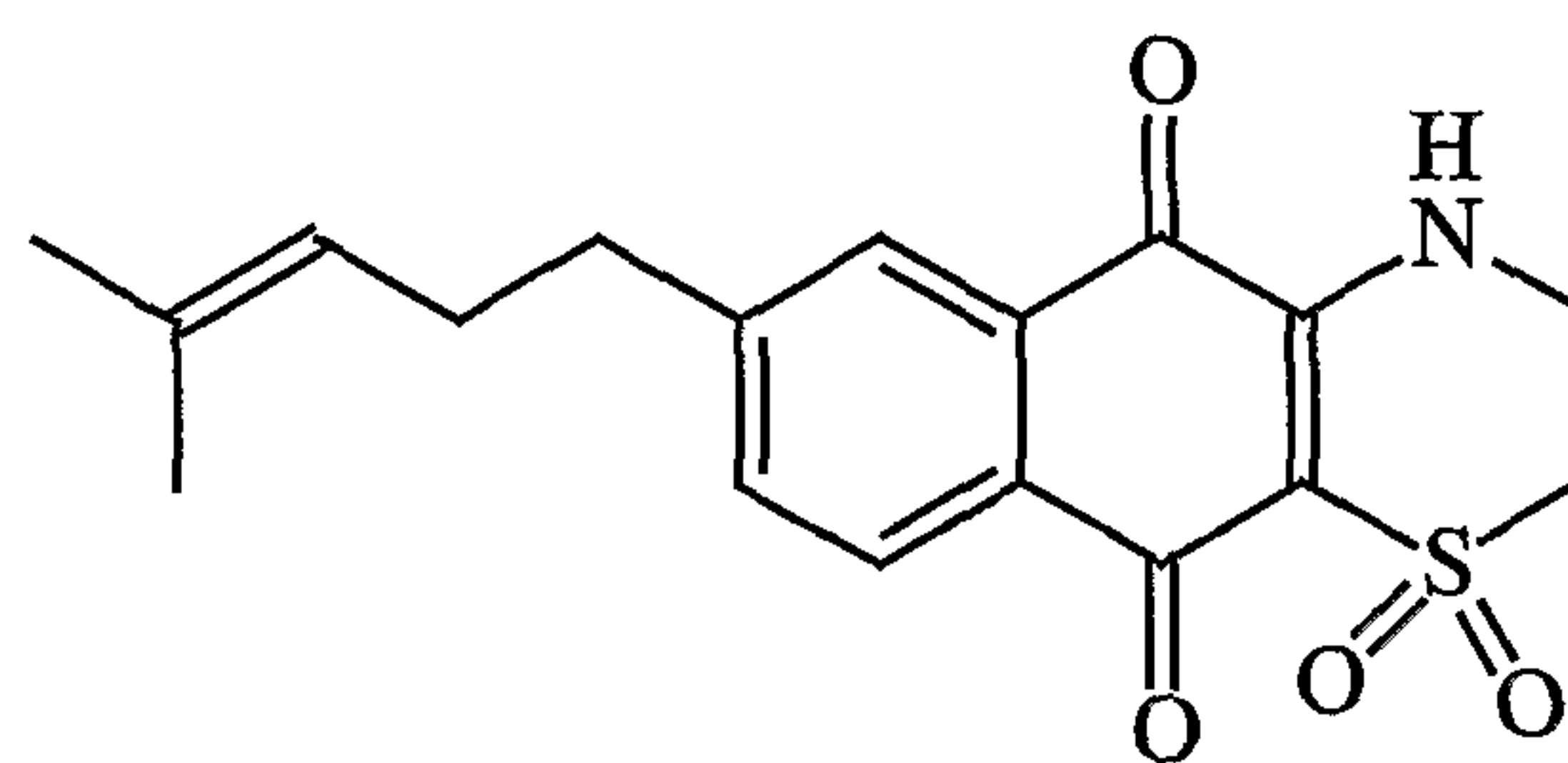
Conicaquinone B
