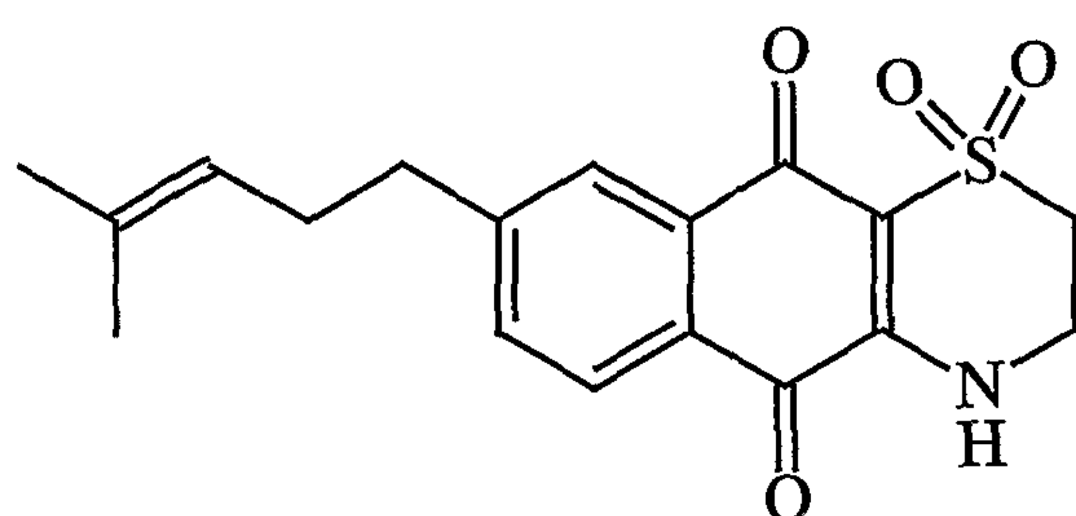
Conicaquinone A
