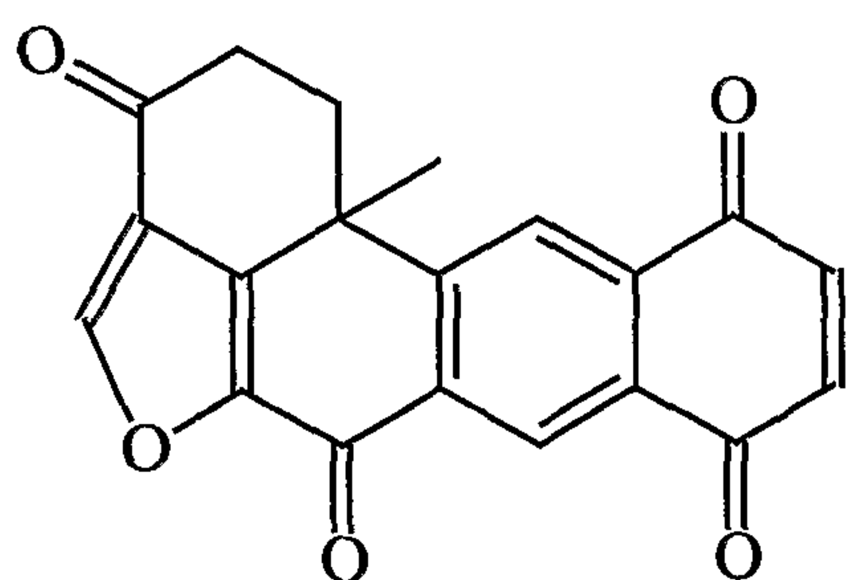
Helenaquinone
