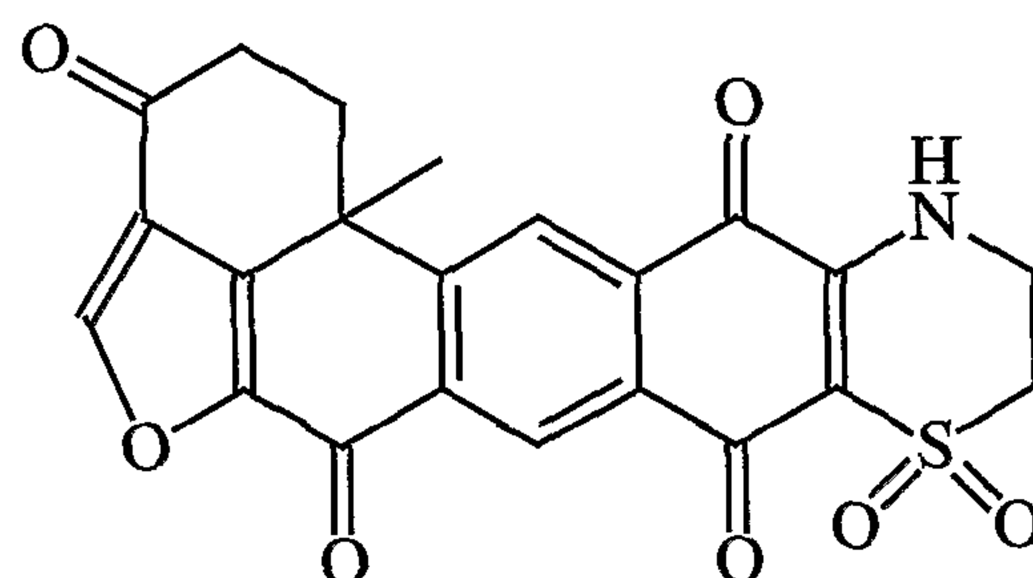
3-Ketoadociaquinone A
