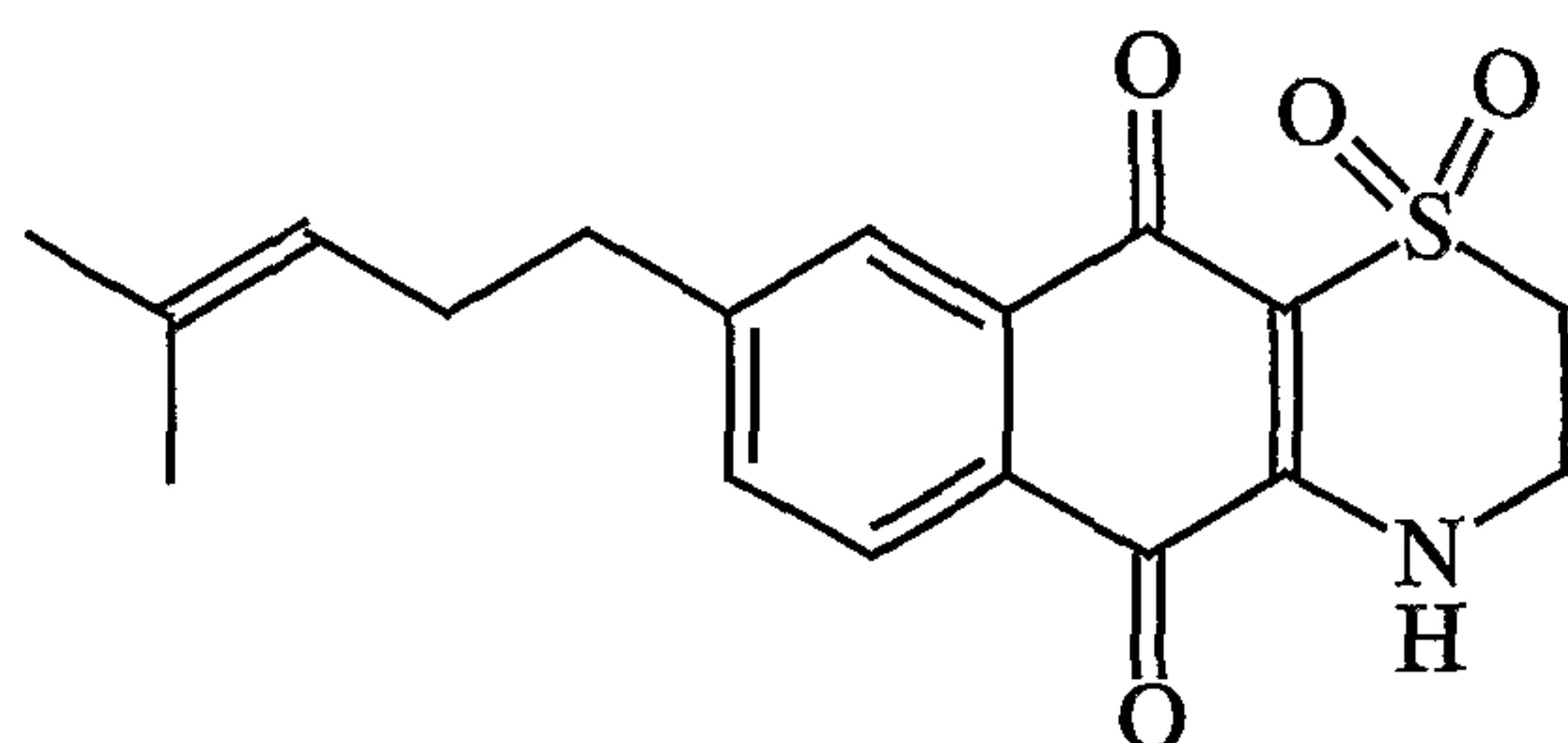
Conicaquinone A
