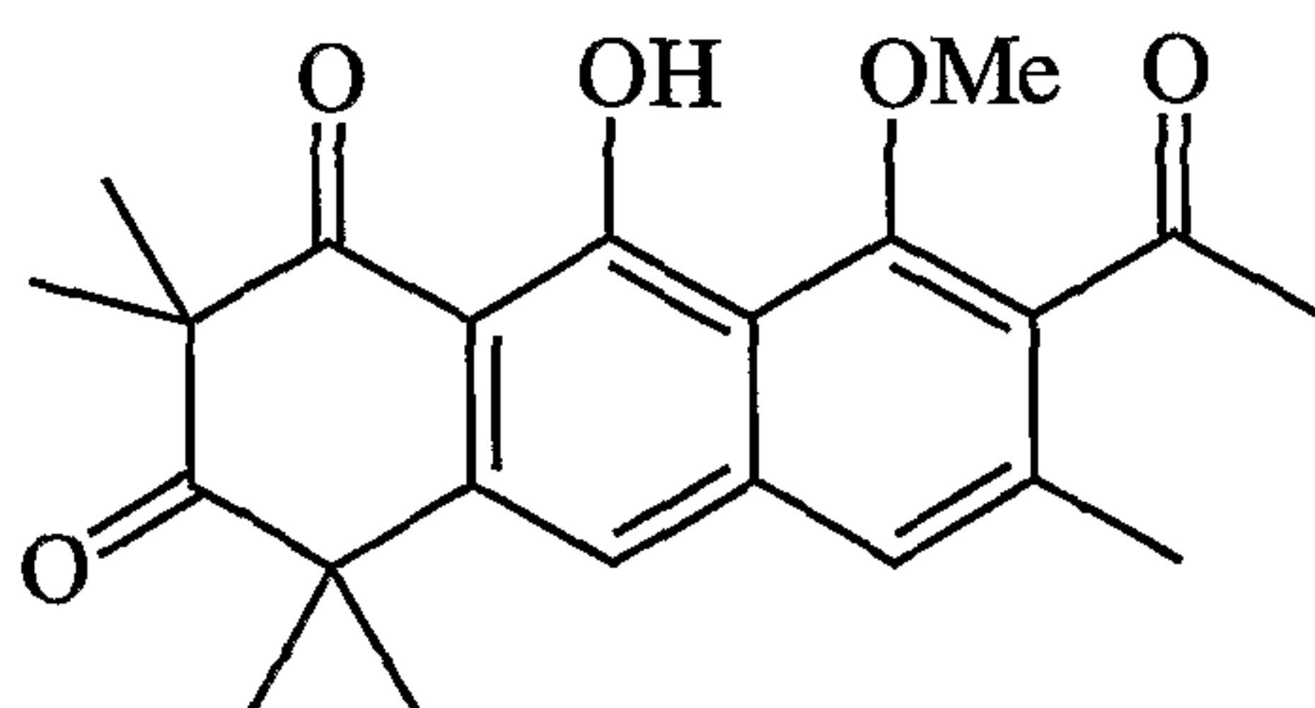
Garveatin C
