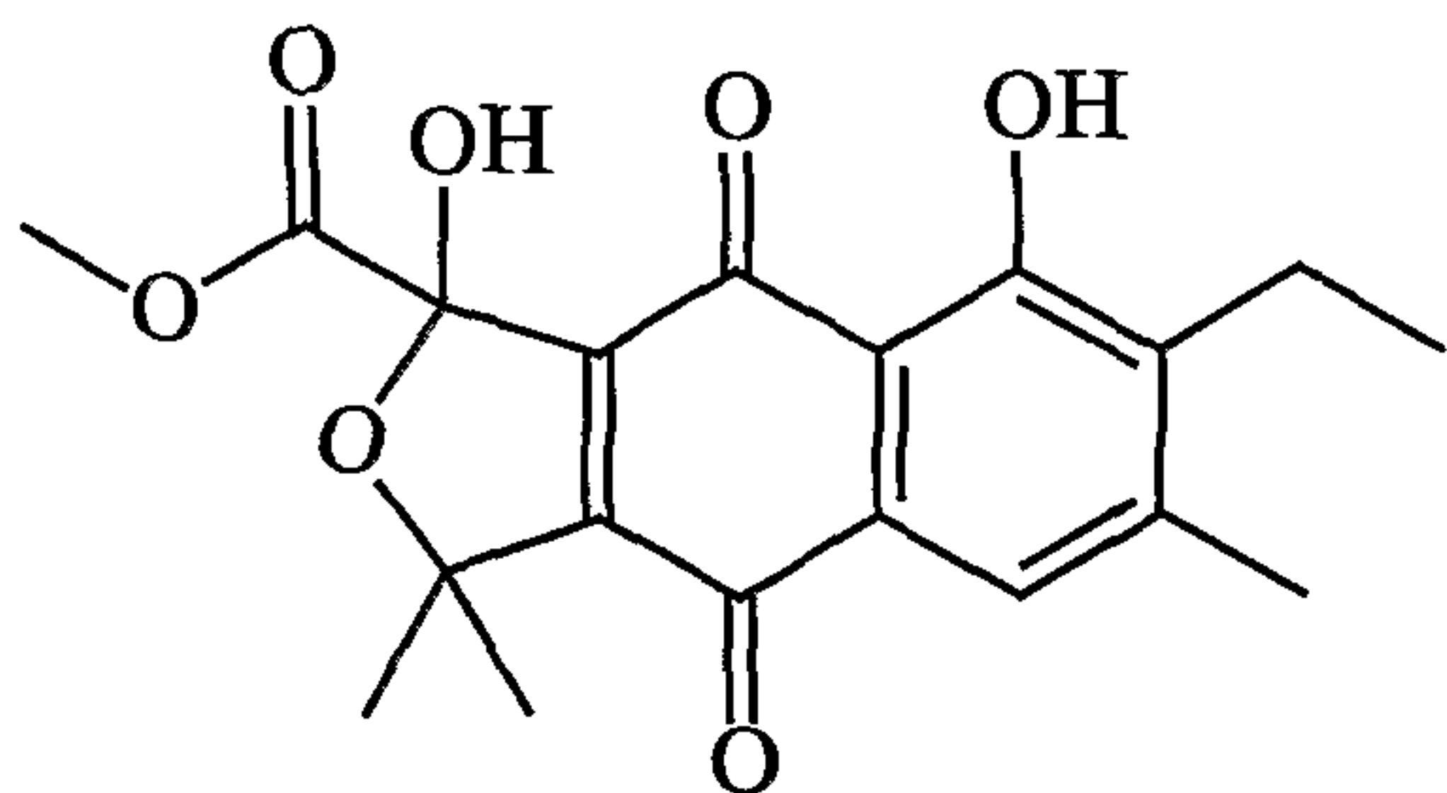
Annulin A
