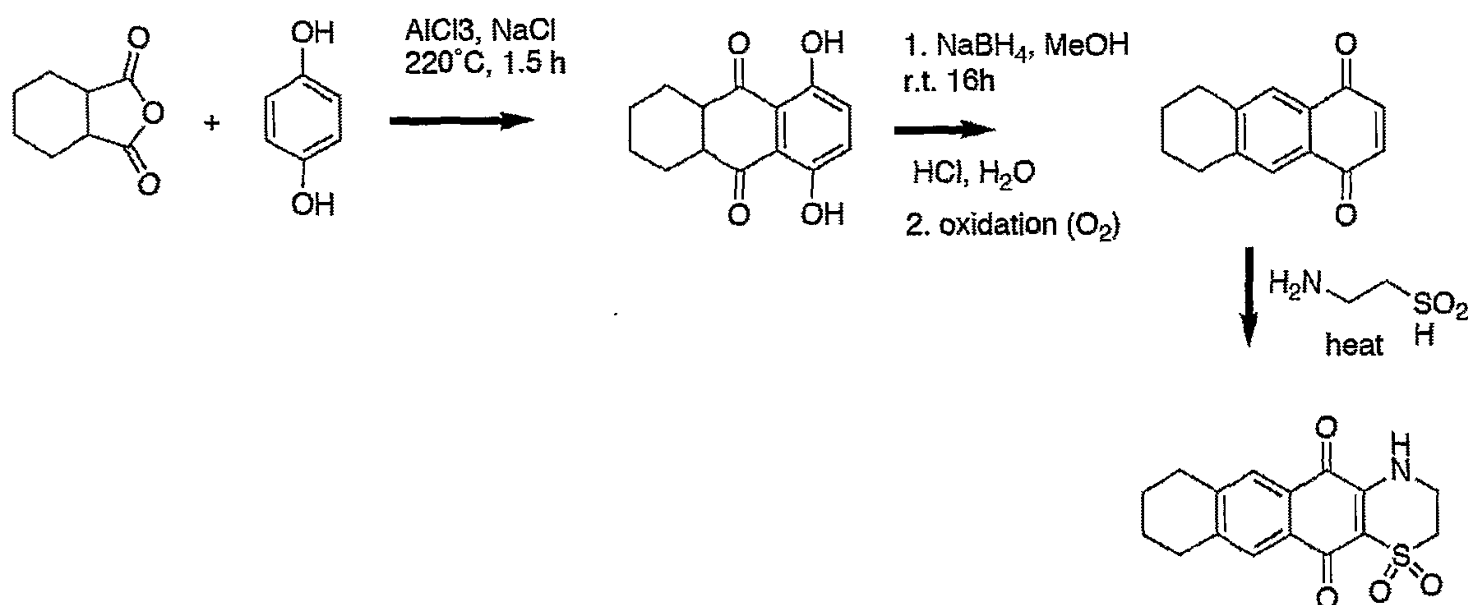
Scheme IV
