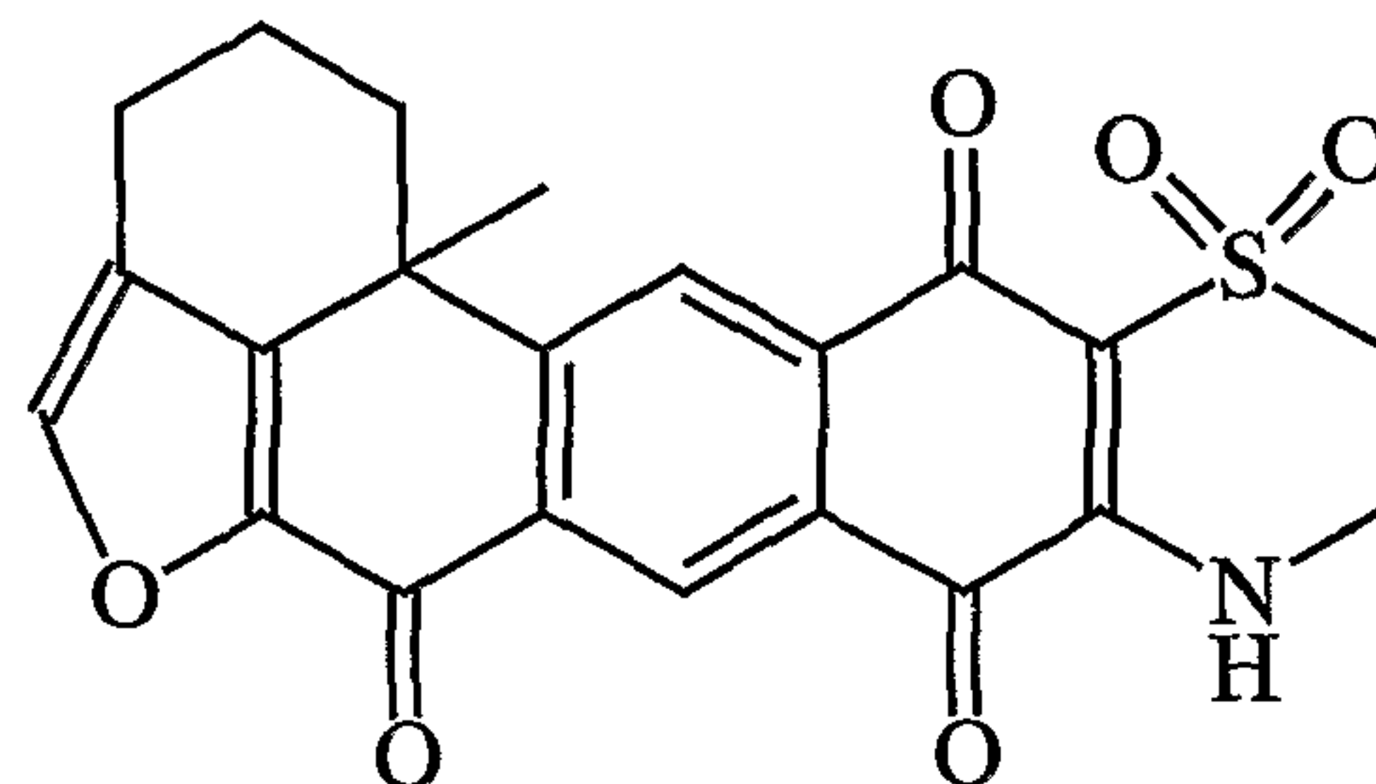
Adociaquinone B
