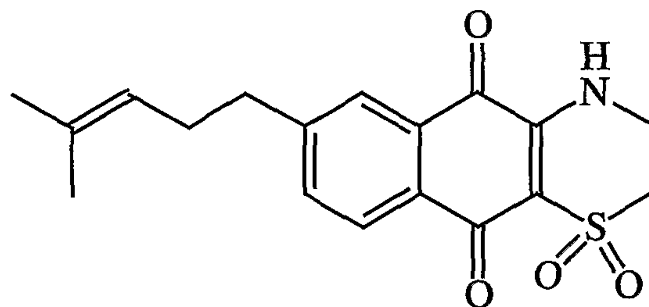
Conicaquinone B
