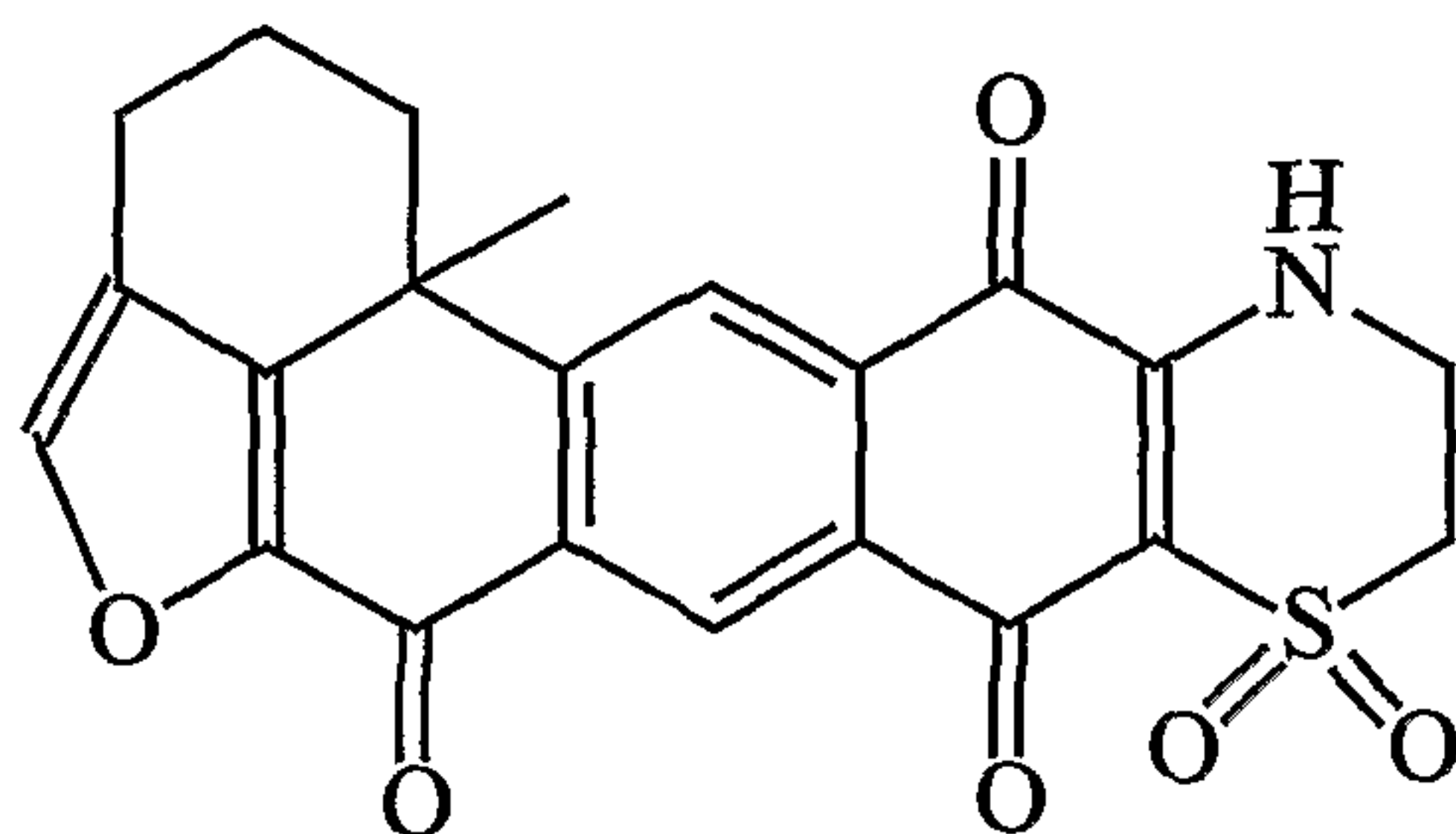
Adociaquinone A
