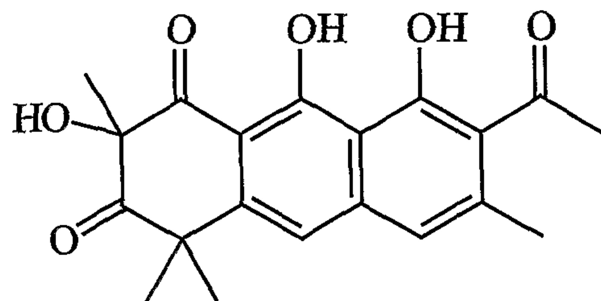
2-hydroxyGarveatin A
