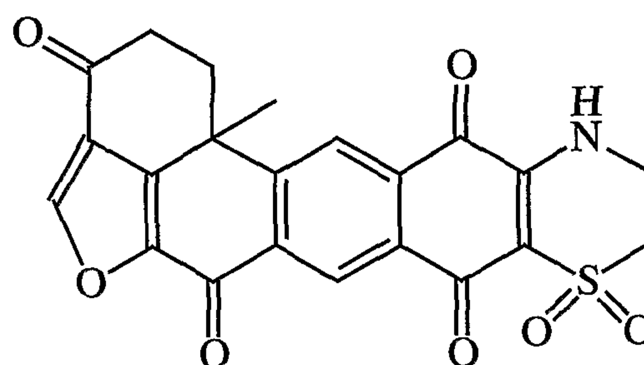
3-Ketoadociaquinone A
