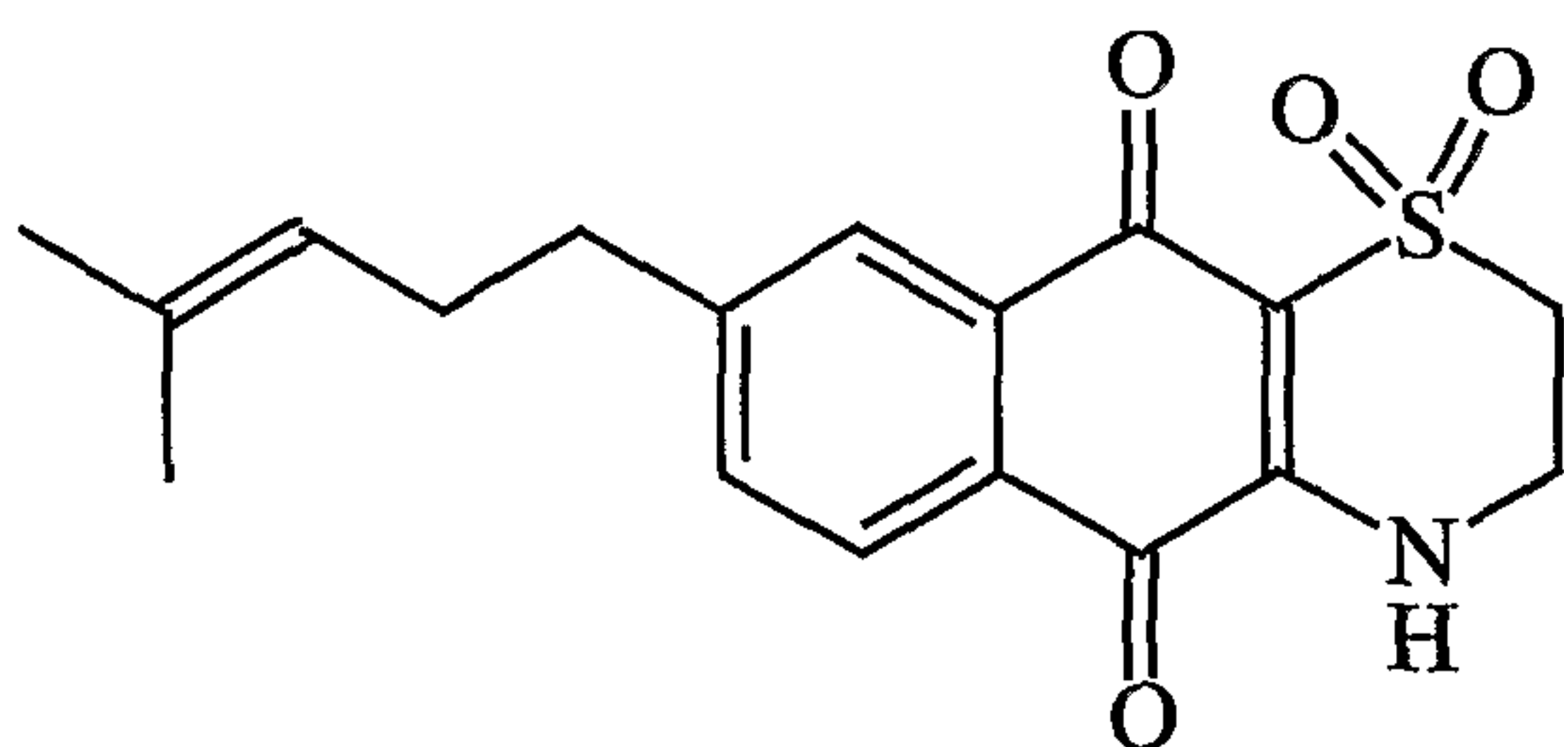
Conicaquinone A
