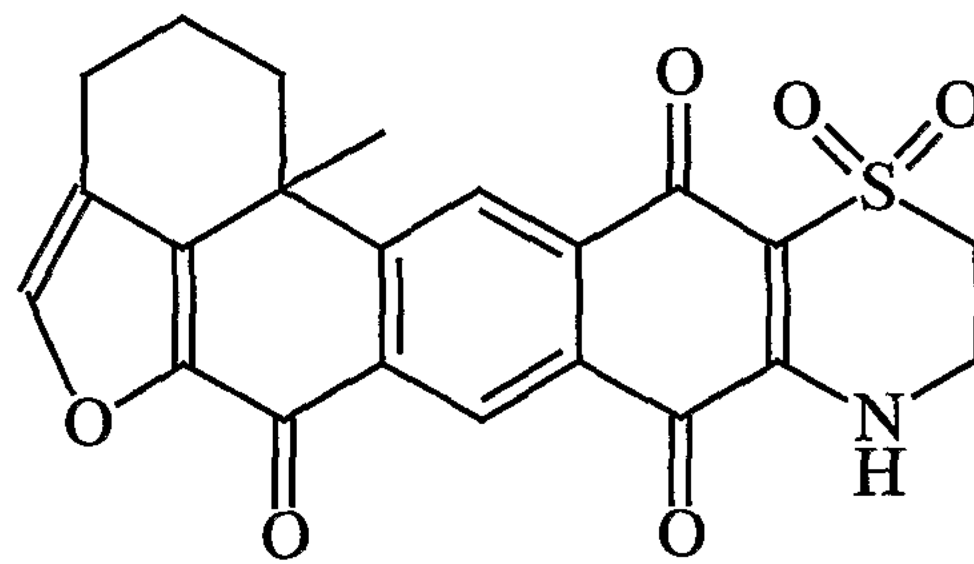
Adociaquinone B
