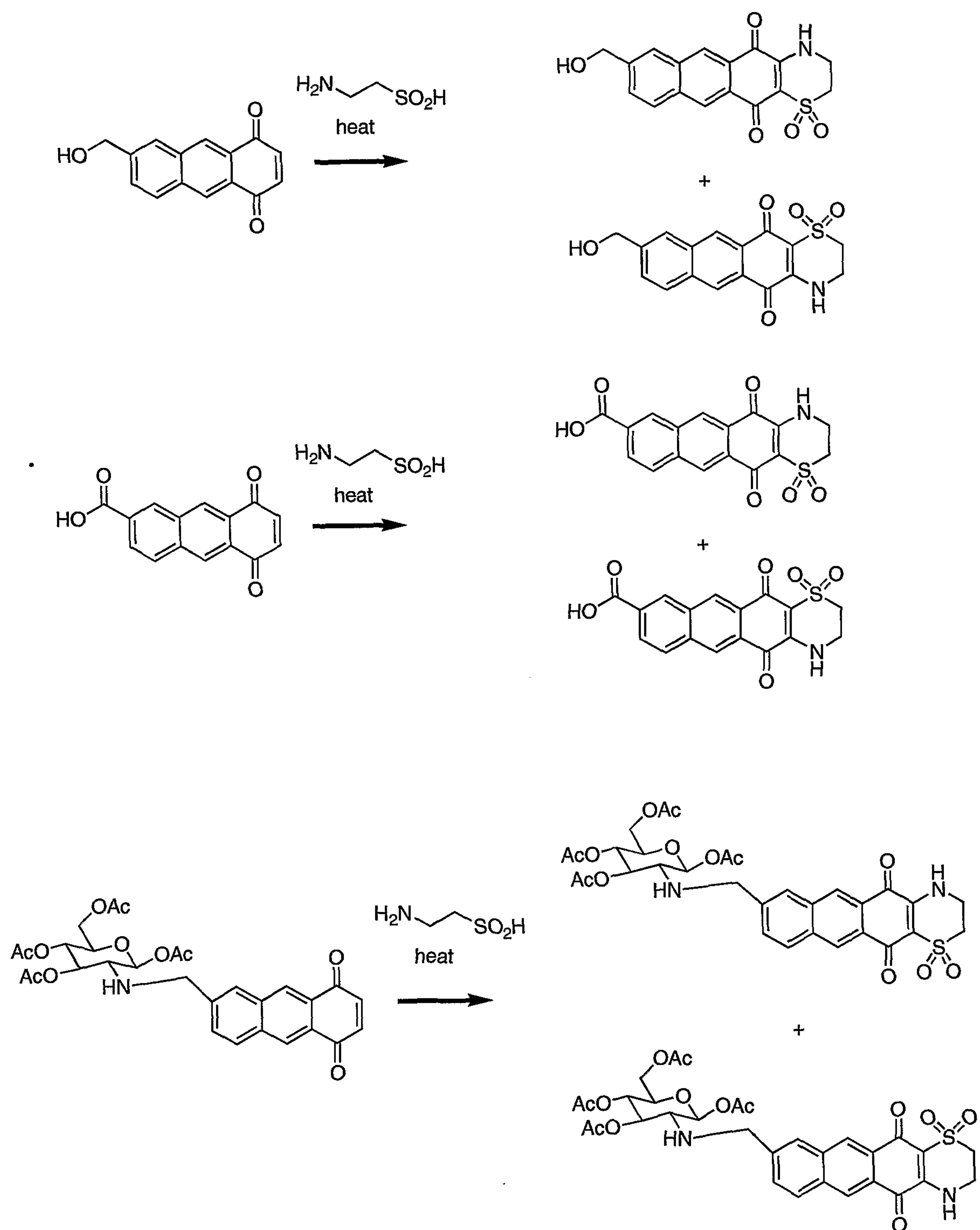
Scheme III
