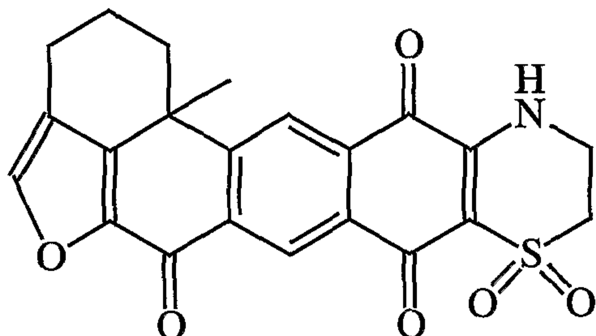
Adociaquinone A
