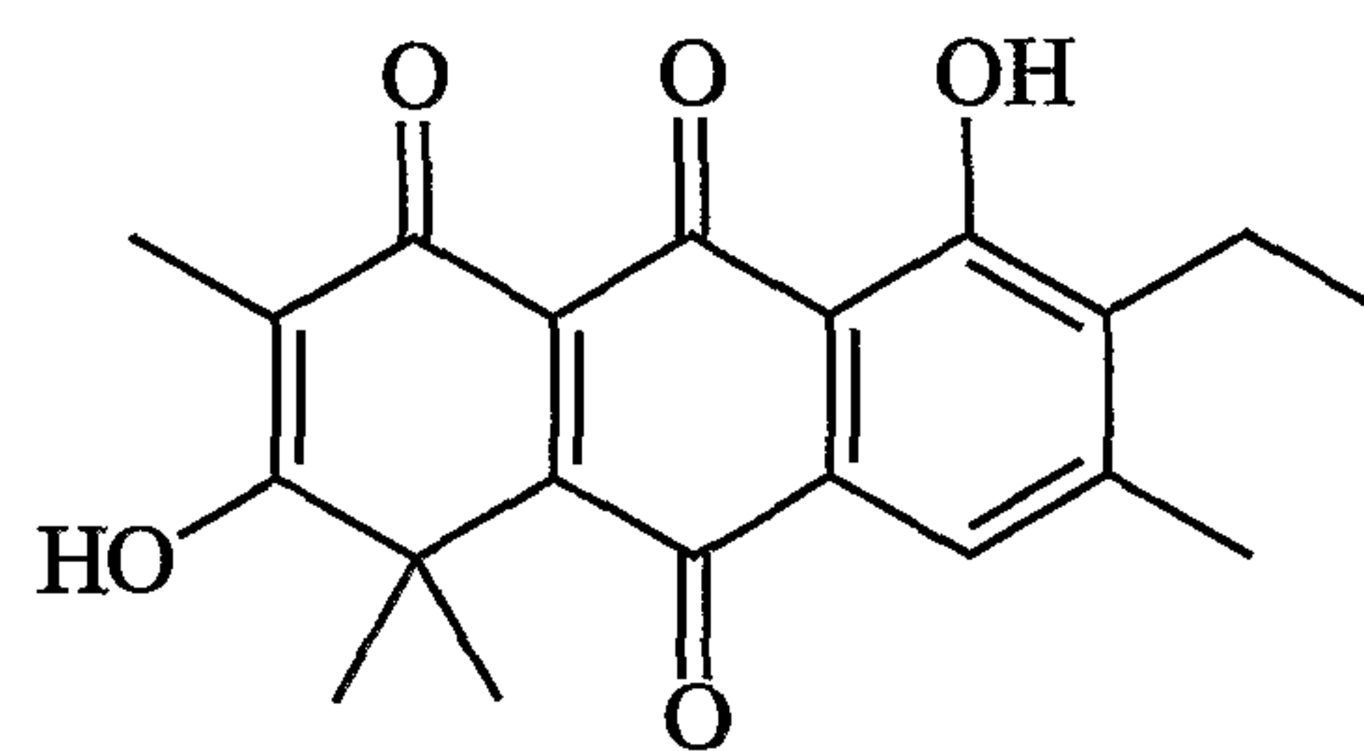
Conicaquinone B
