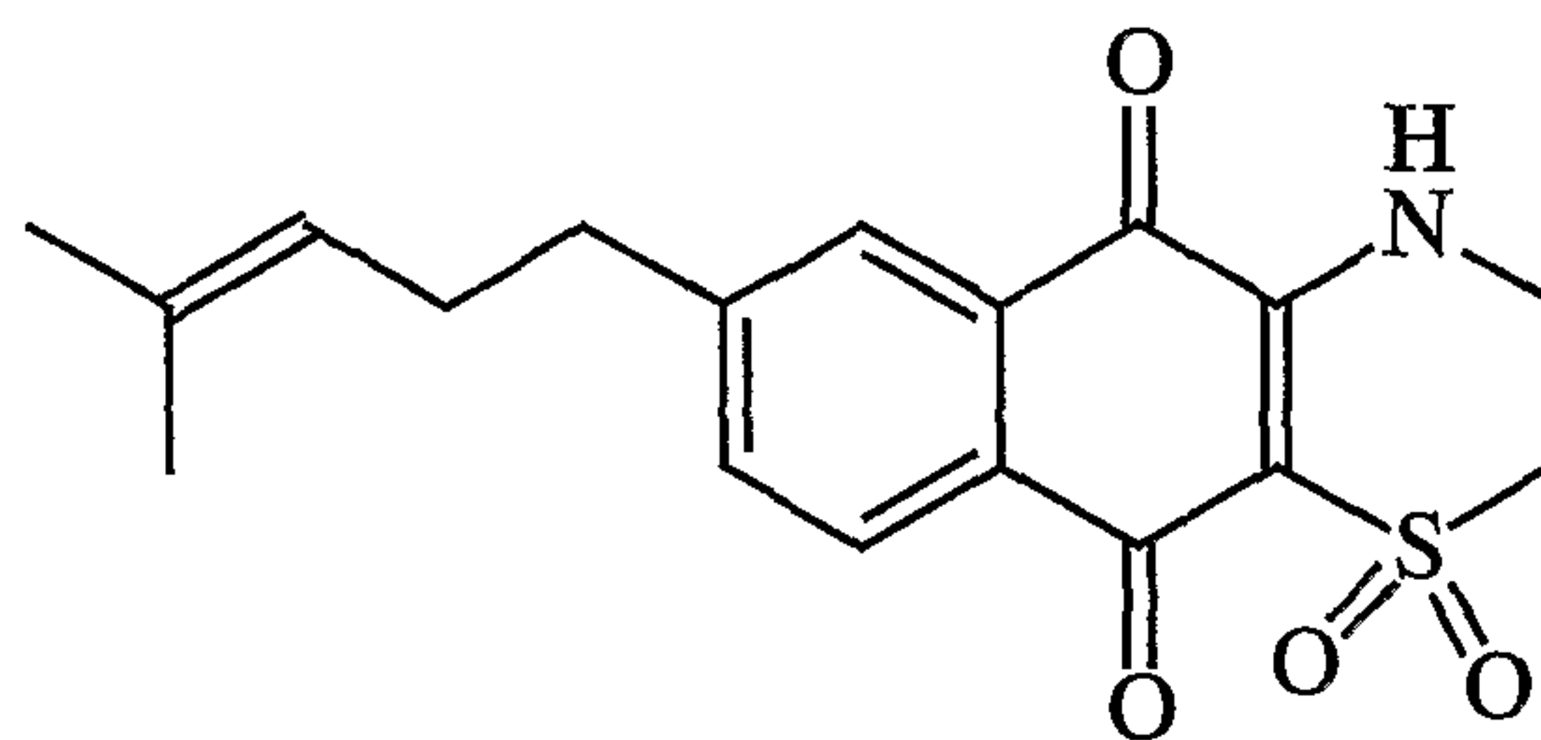
Conicaquinone B
