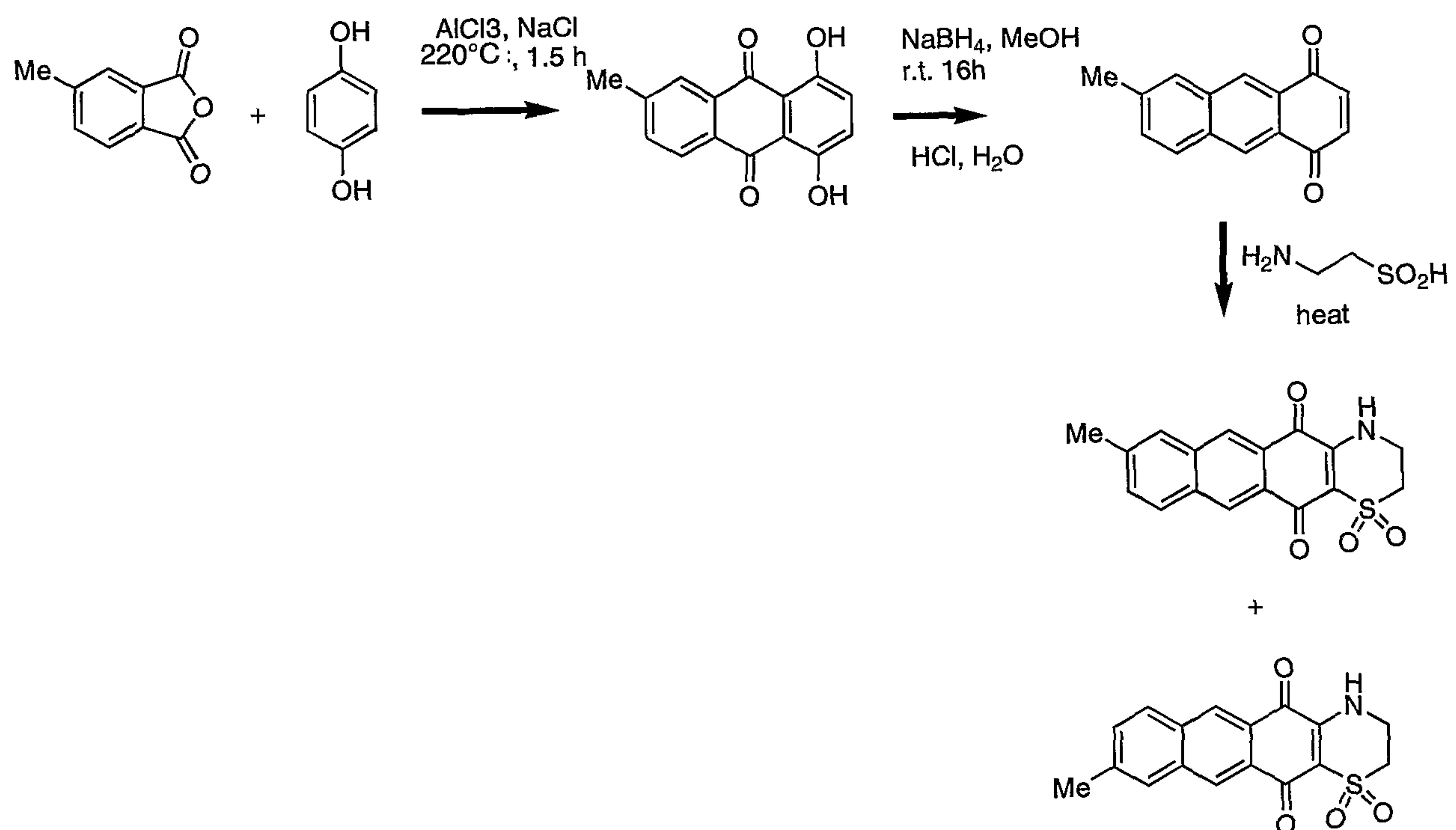
Scheme I
