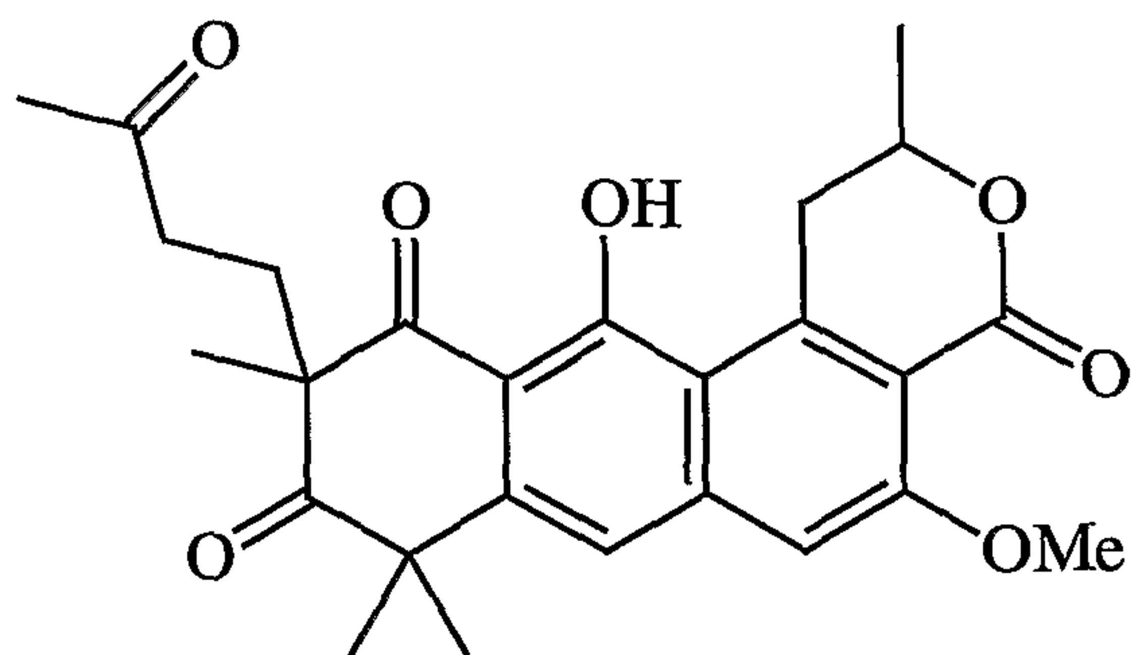
Garvalone B
