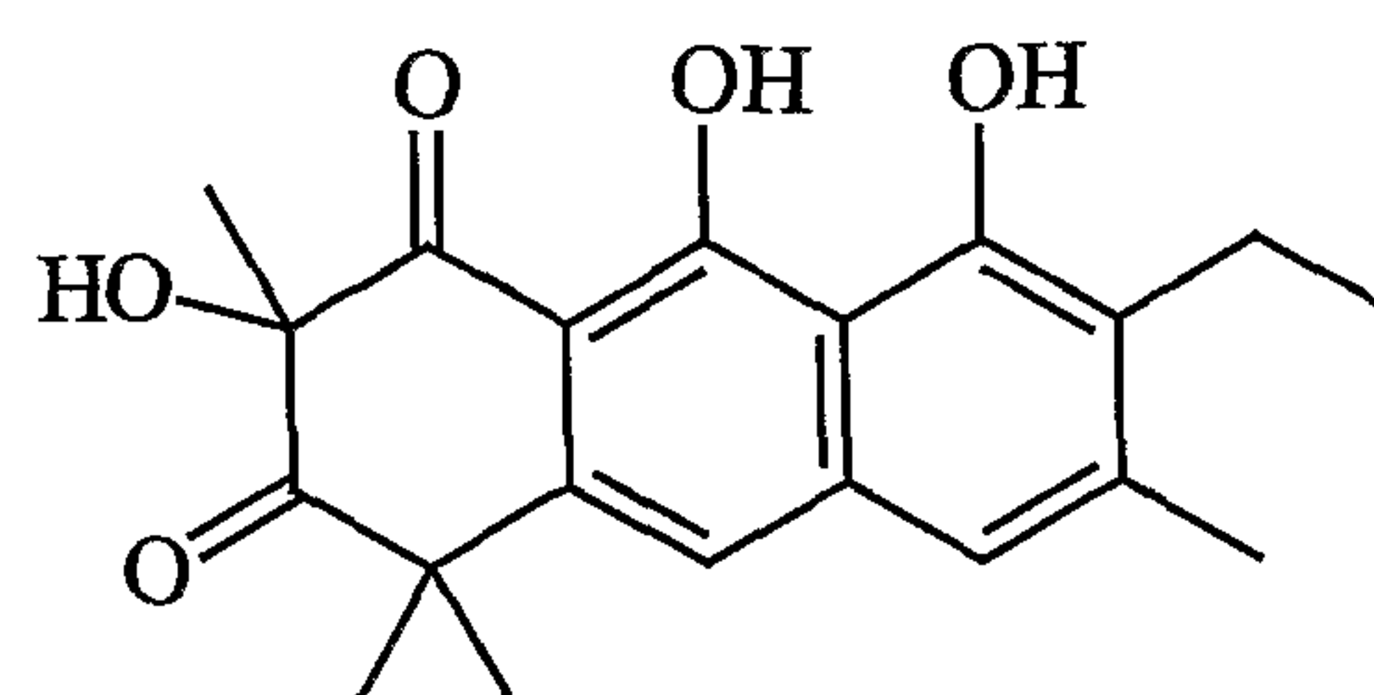
2-hydroxyGarveatin B
