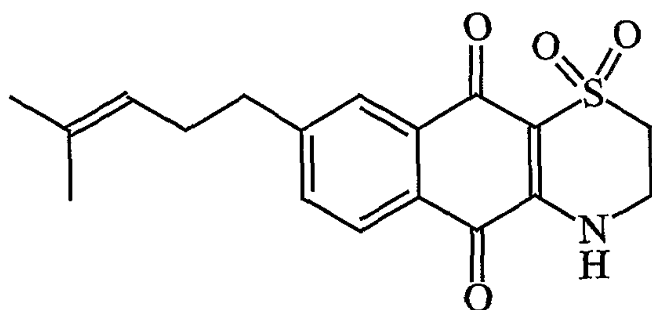
Conicaquinone A
