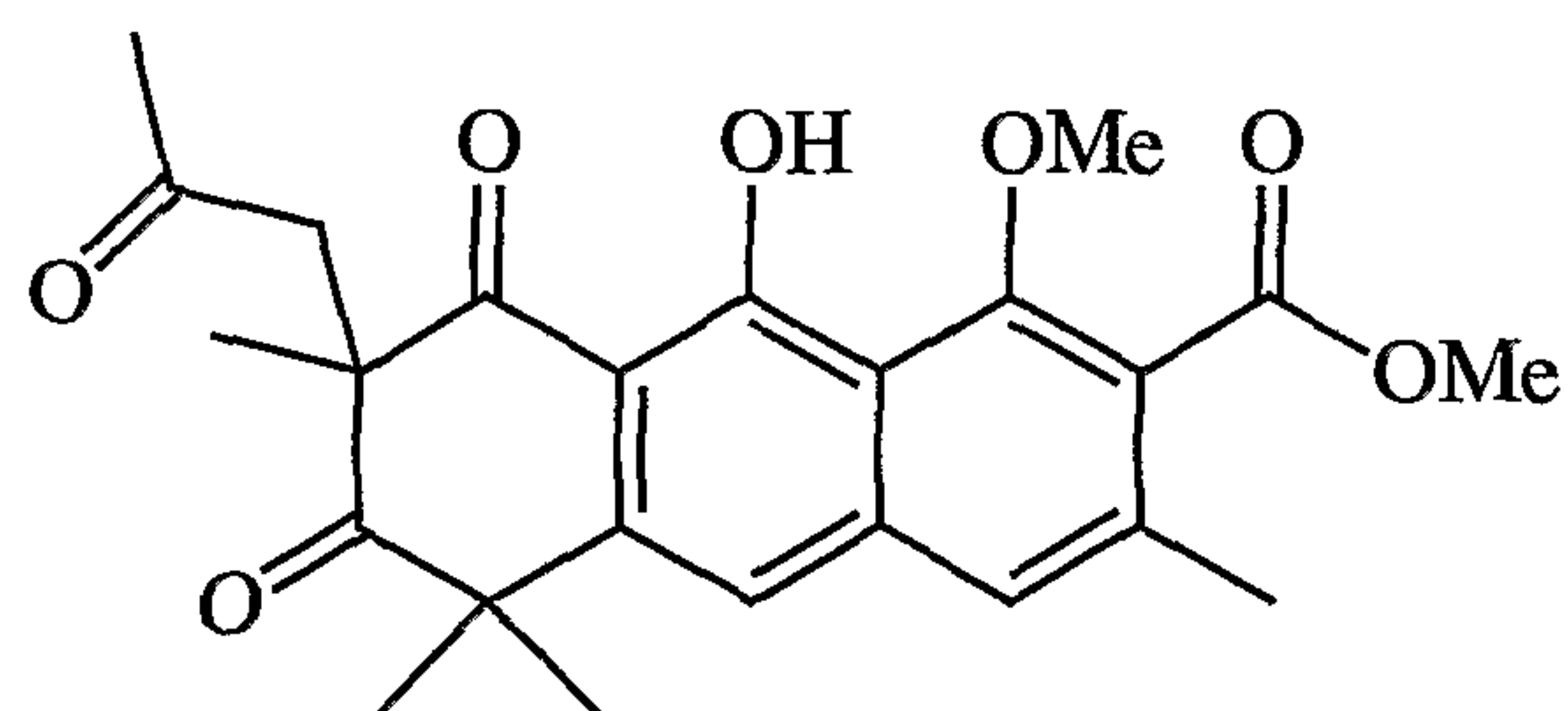
Garvalone C
