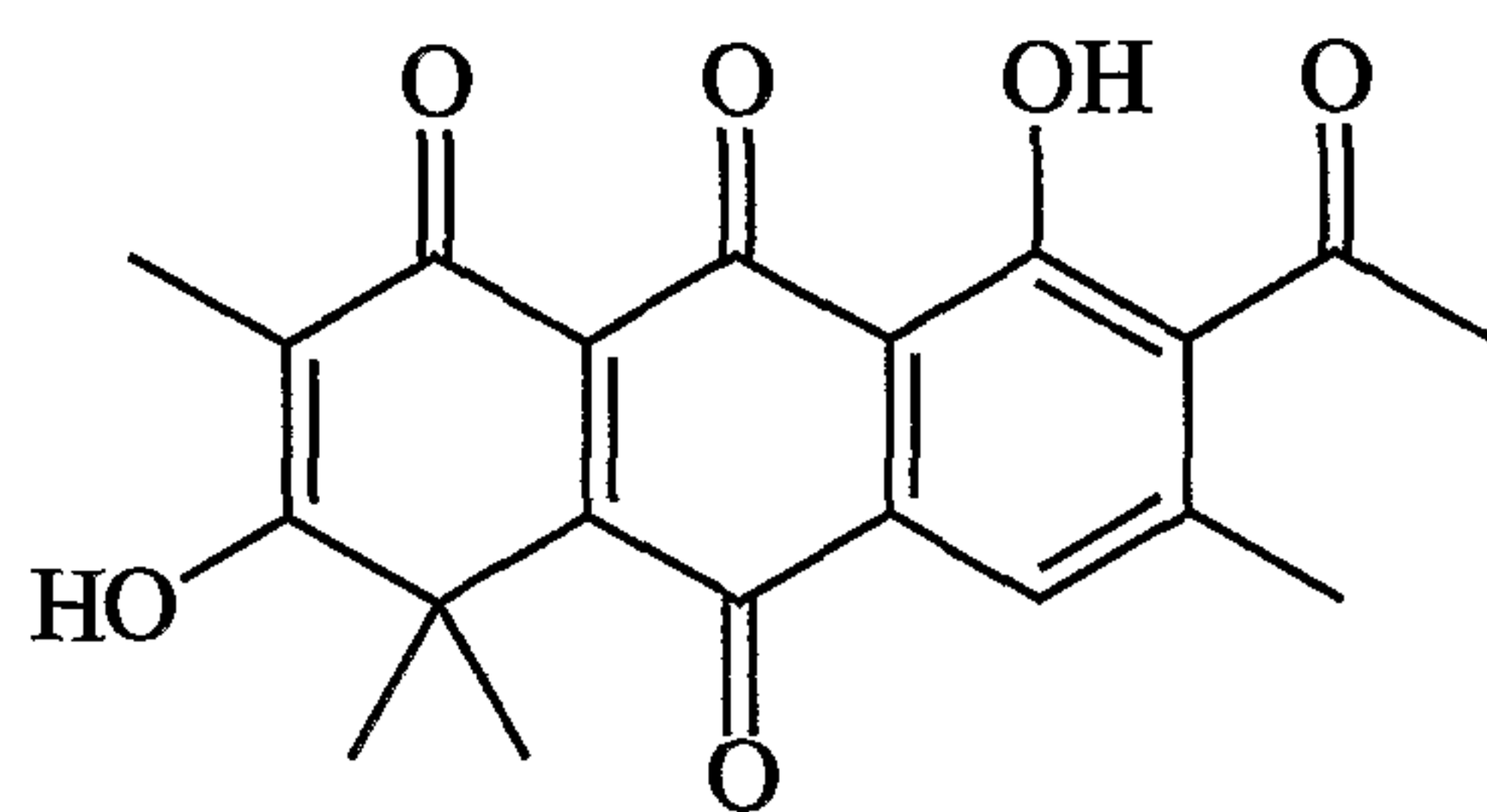
Conicaquinone A
