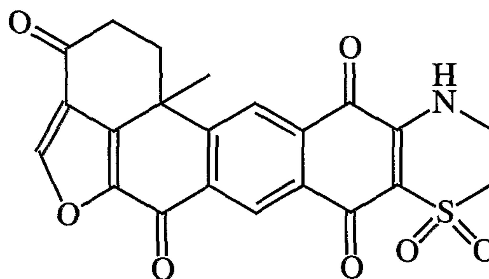
3-Ketoadociaquinone A
