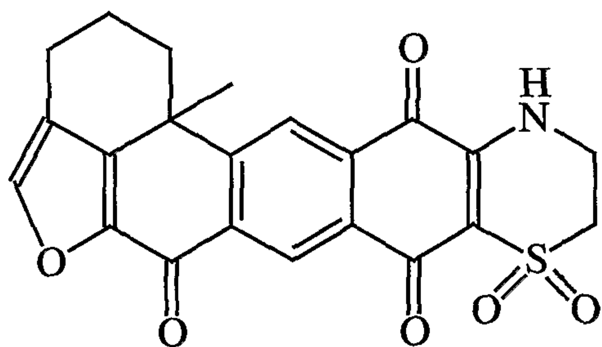
Adociaquinone A
