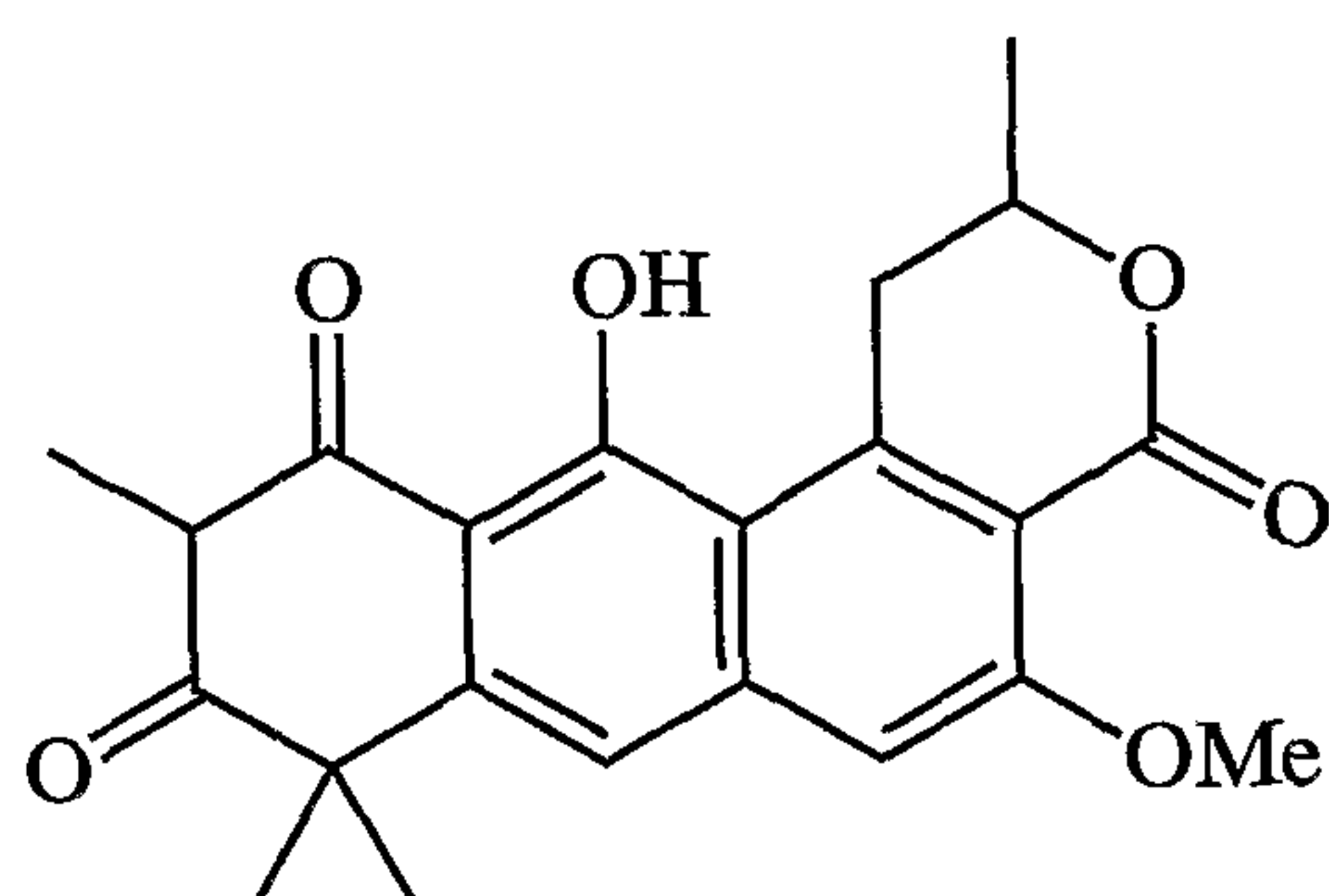
Garvin B
