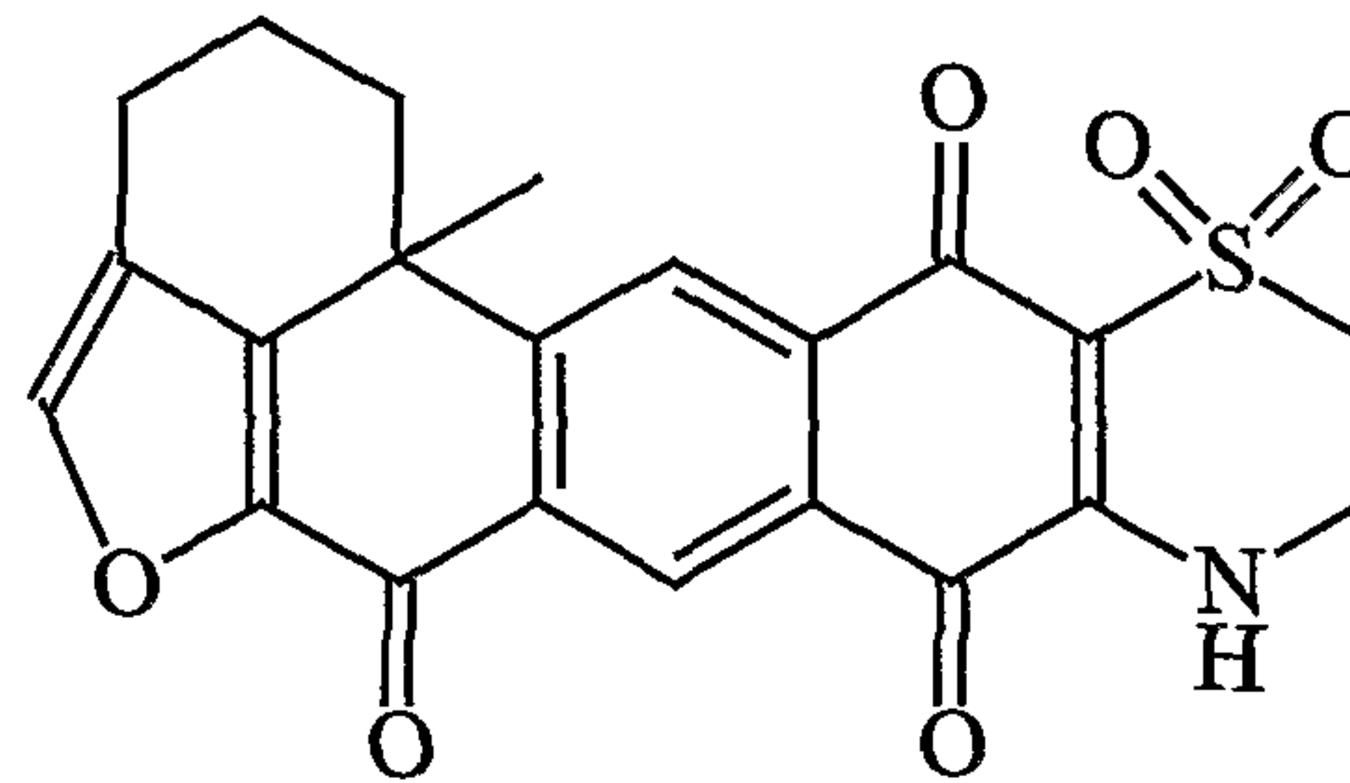
Adociaquinone B
