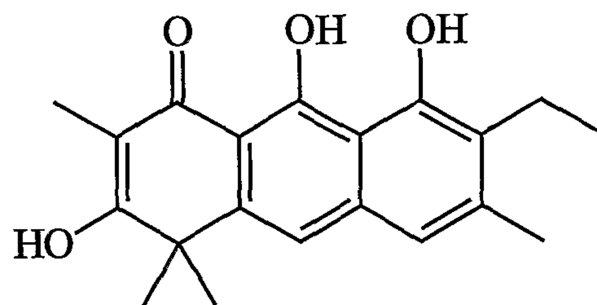
Garveatin B
