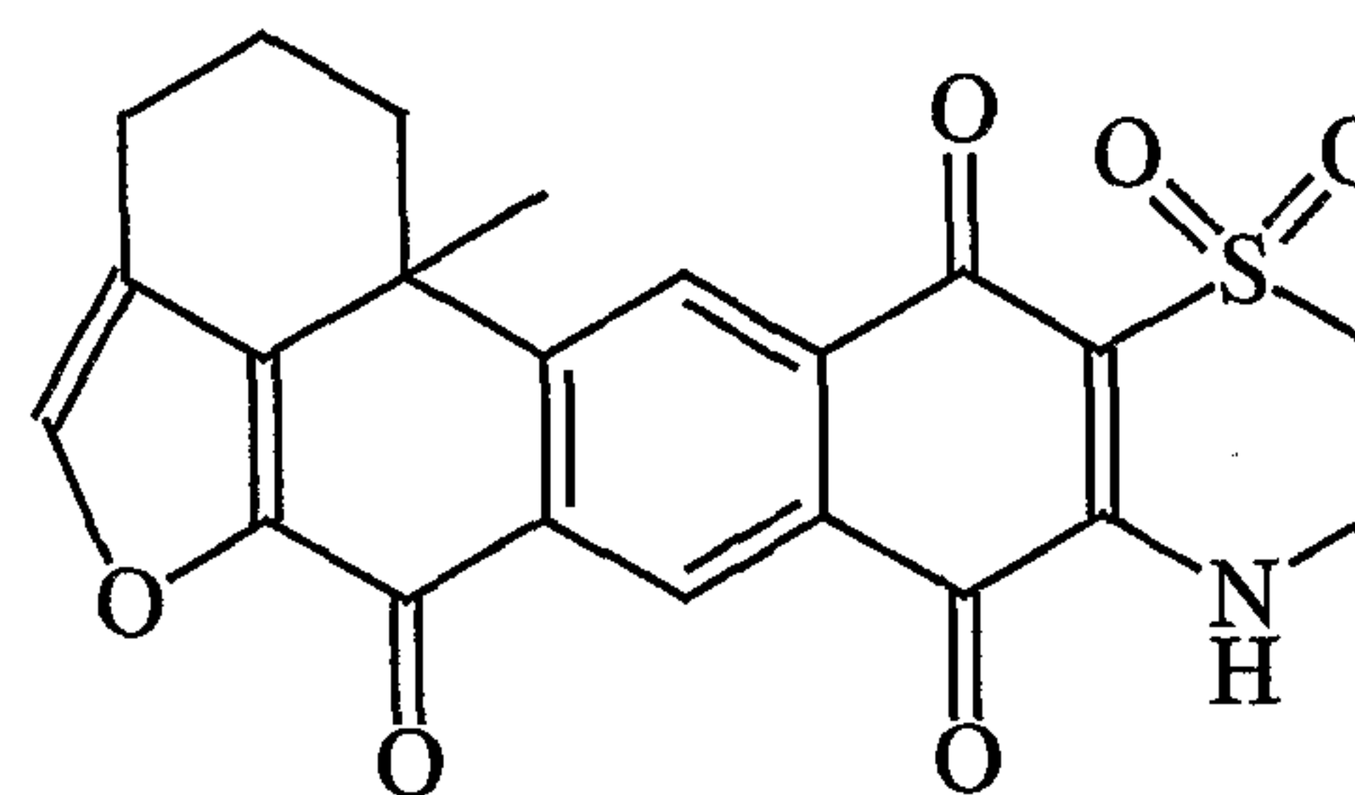
Adociaquinone B
