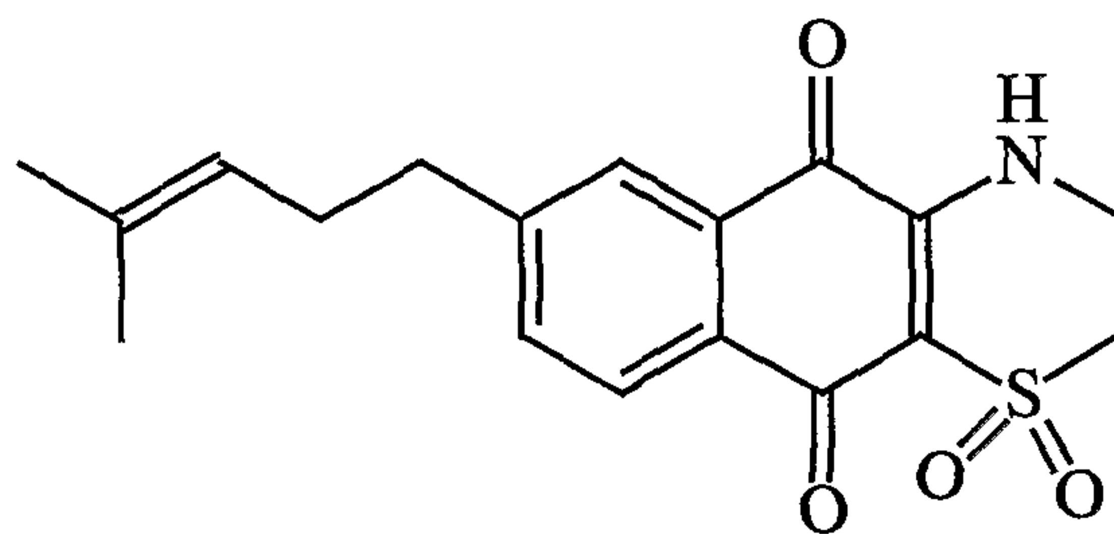
Conicaquinone B
