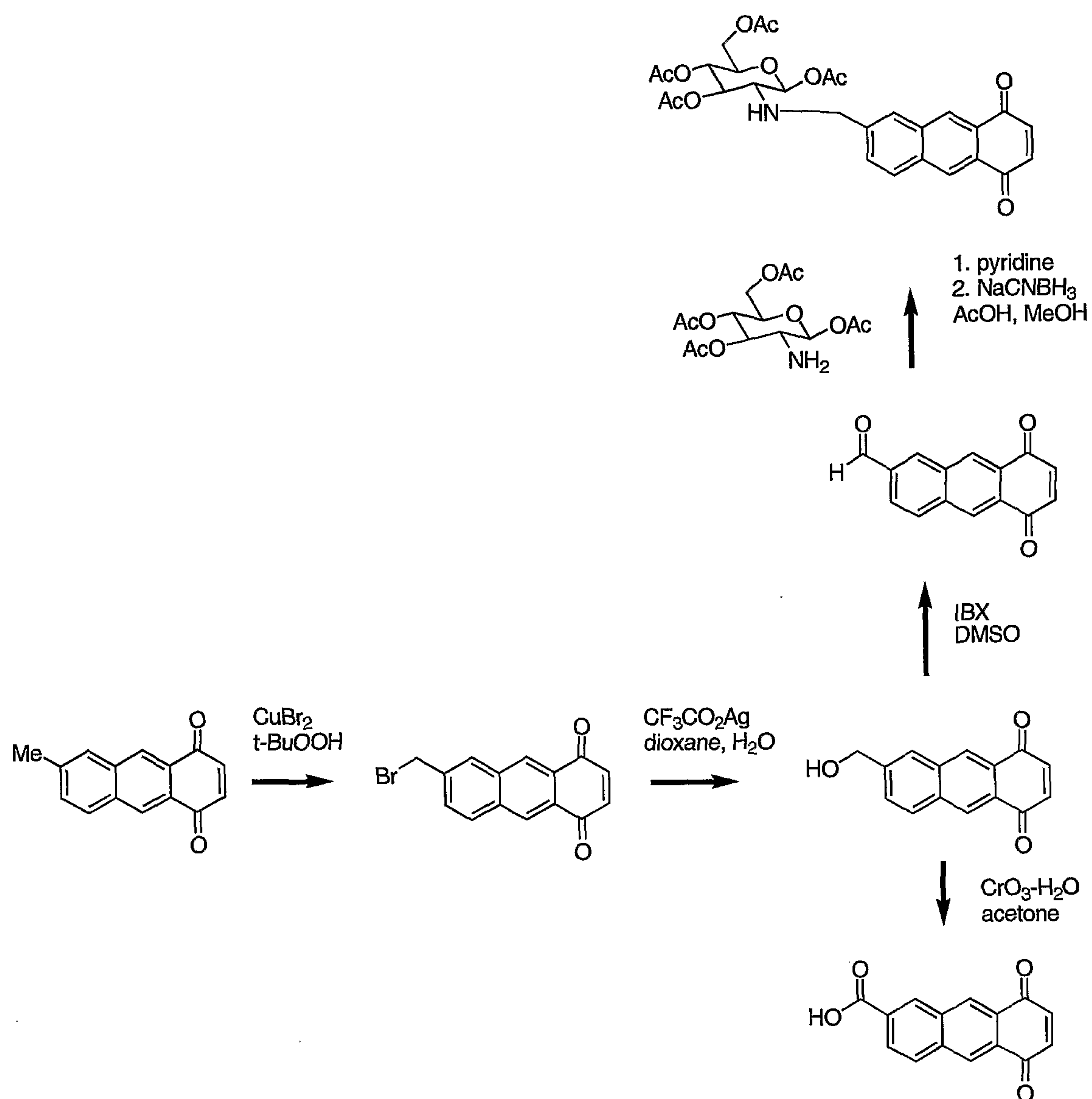
Scheme II
