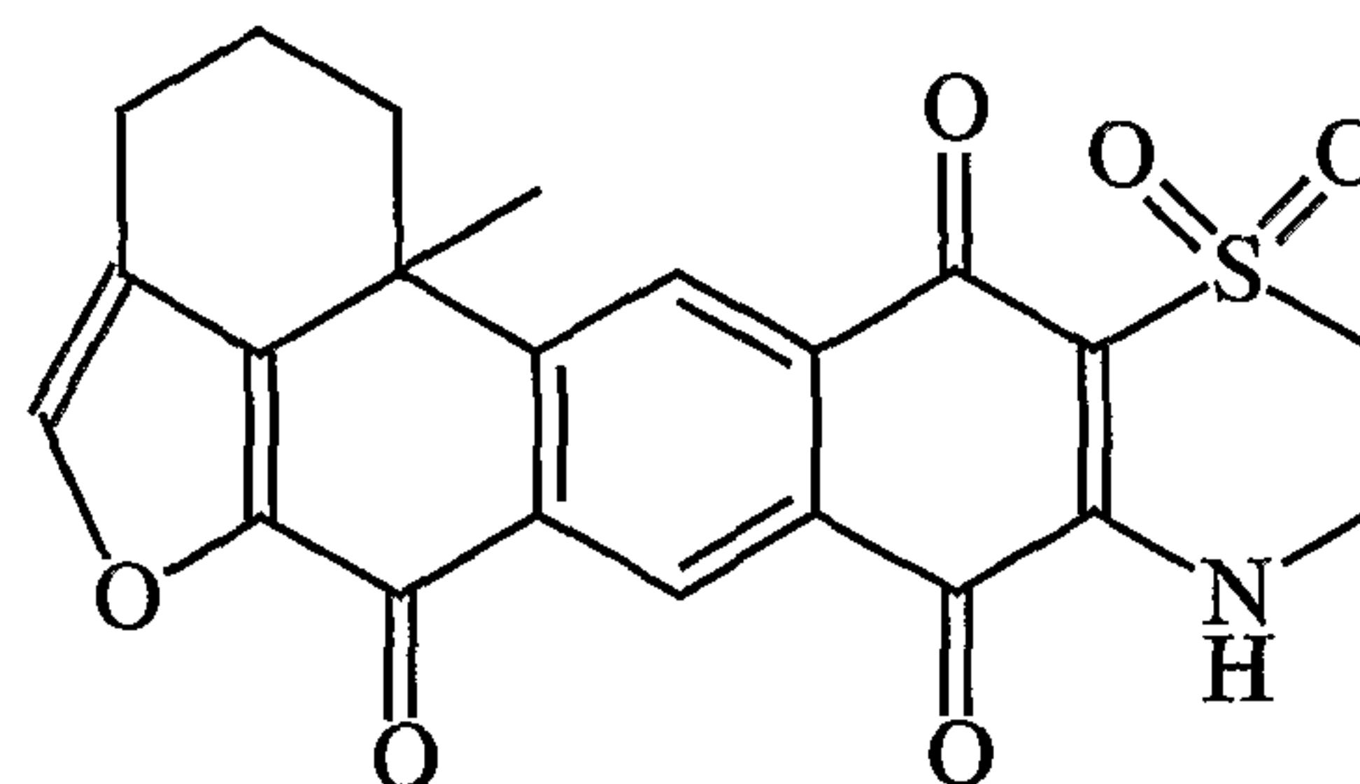
Adociaquinone B
