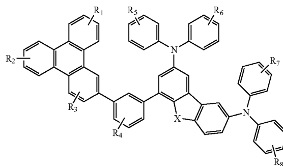
Compound 28G
