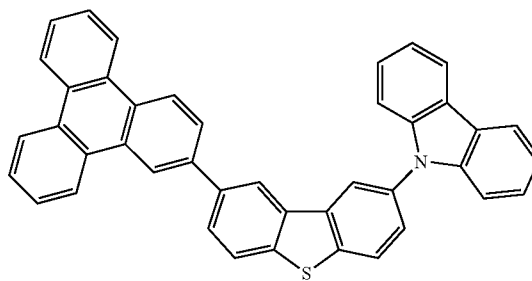
Compound 19
