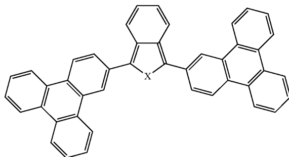
Compound 11
