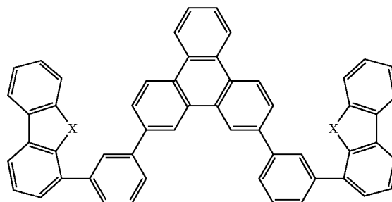
Compound 4
