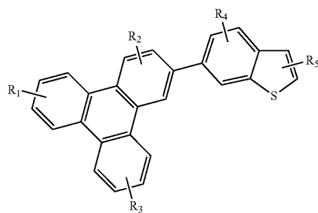
Compound 17'G
