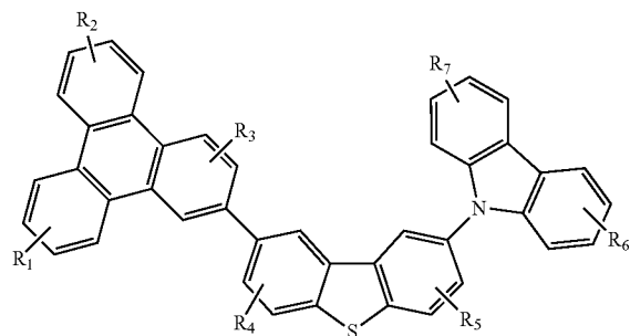
Compound 19 G
