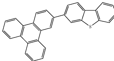
Compound 9'G
