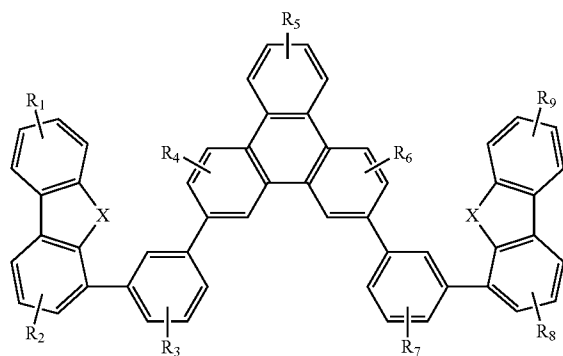
Compound 4G
