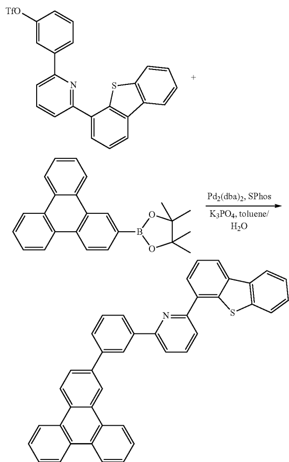
Compound 21S
