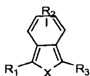
Formula (IV)
