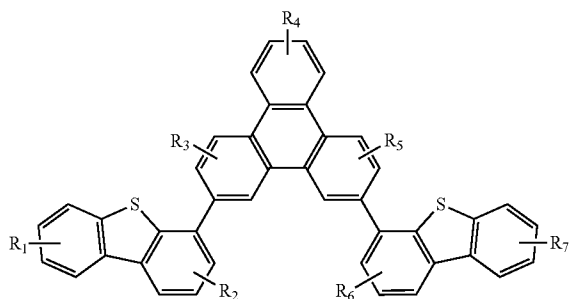
Compound 10'
