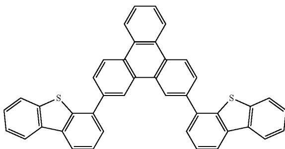
Compound 10'
