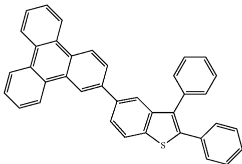
Compound 13'
