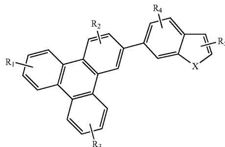
Compound 18G
