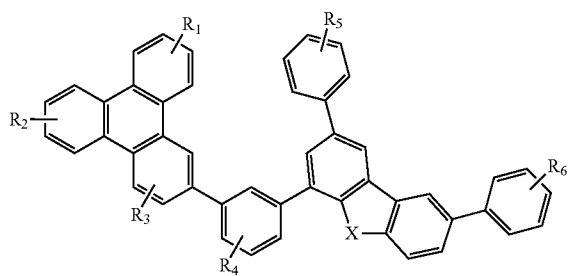
Compound 25 G
