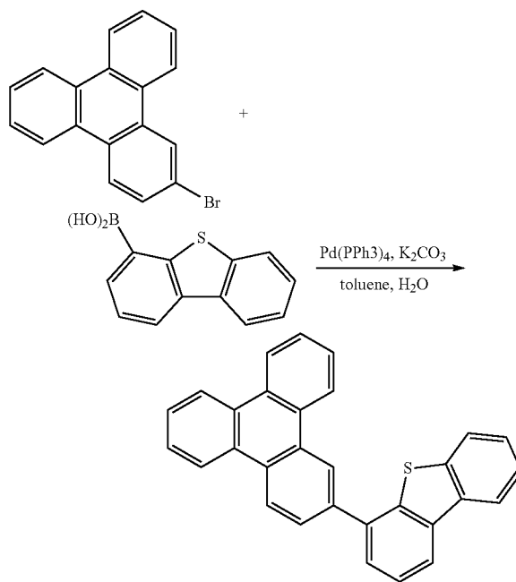
Compound 1S
