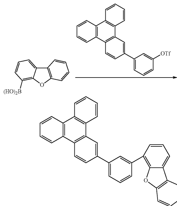
Compound 20
