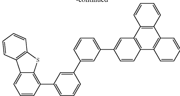
Compound 9S
