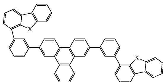
Compound 26
