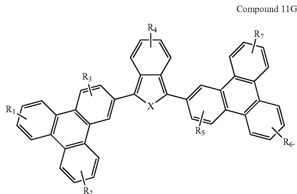
Compound 11G
