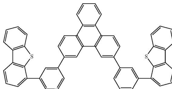
Compound 4'
