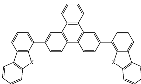
Compound 19
