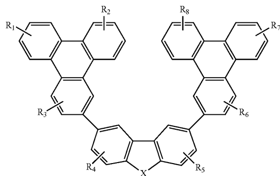
Compound 5G
