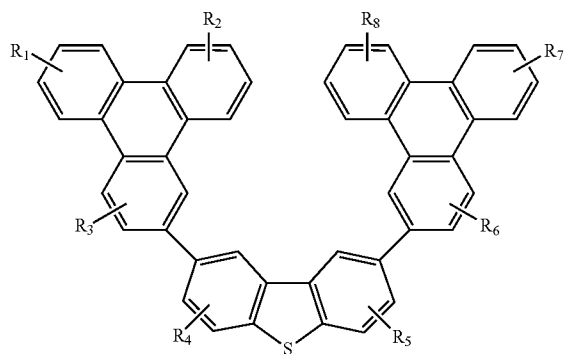
Compound 5'
