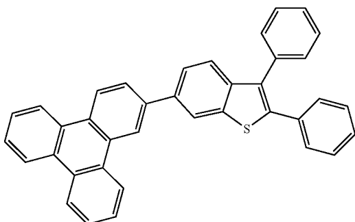
Compound 18'G
