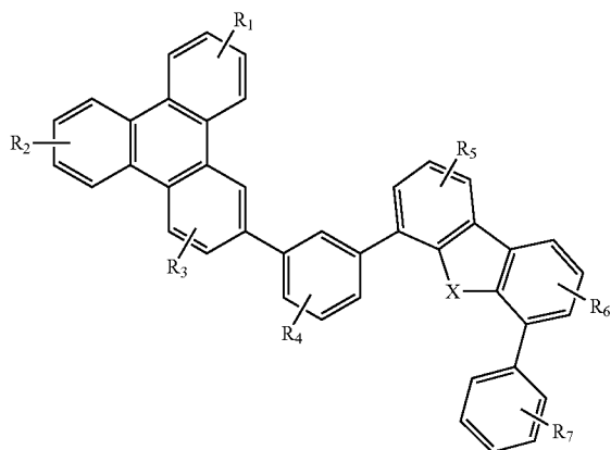
Compound 24 G
