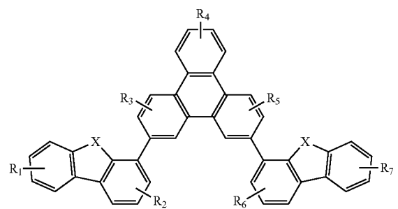
Compound 10G
