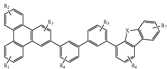
Compound 10G
