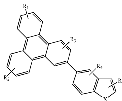
Compound 18'
