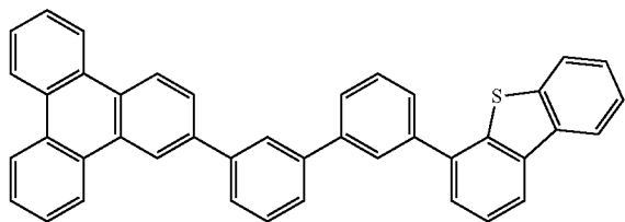
Compound 10'G
