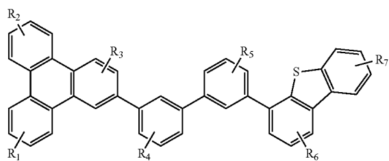
Compound 9'G
