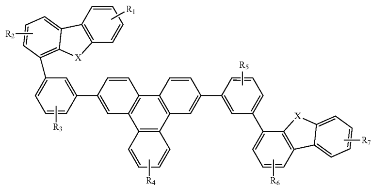
Compound 26
