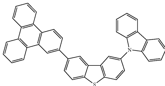
Compound 15'
