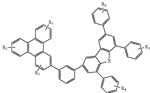
Compound 36G
