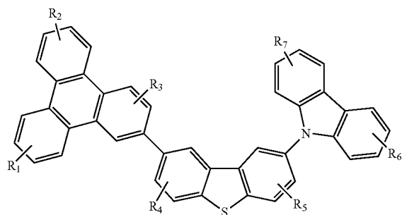
Compound 15'G
