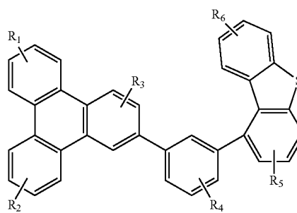
Compound 1'G
