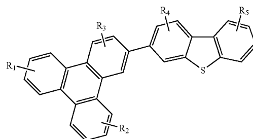
Compound 8'G
