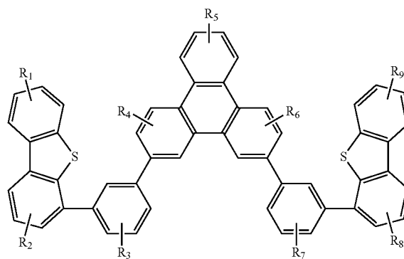
Compound 4'G
