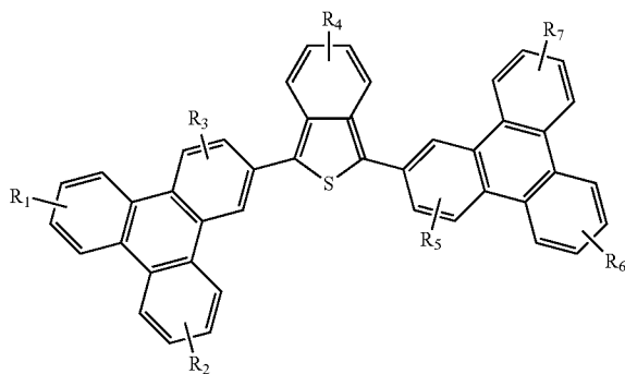
Compound 11'
