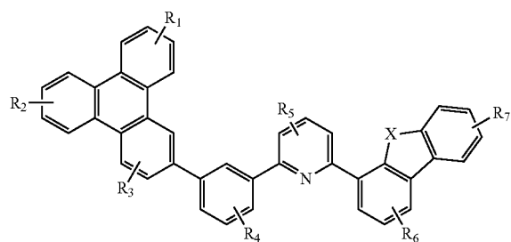
Compound 21 G
