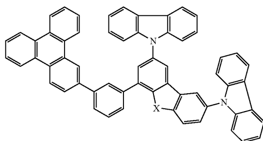
Compound 27
