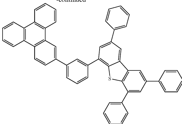
Compound 25S
