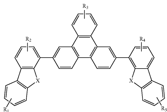
Compound 19 G
