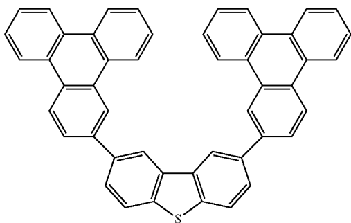
Compound 5'
