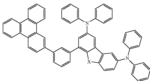
Compound 28
