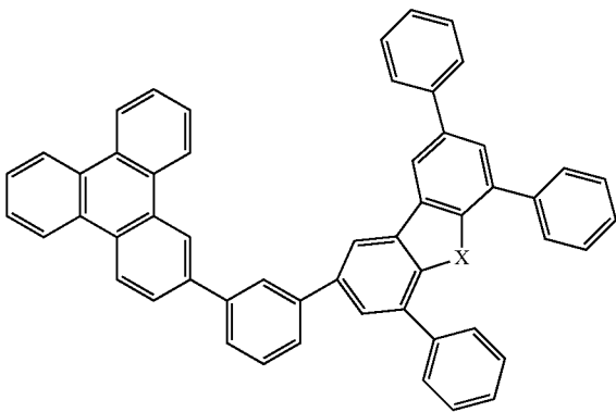
Compound 36
