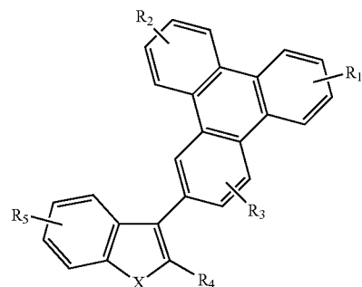
Compound 13G
