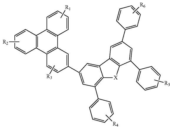
Compound 35G
