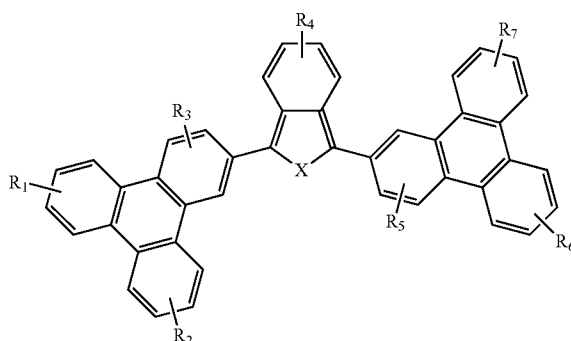
Compound 11
