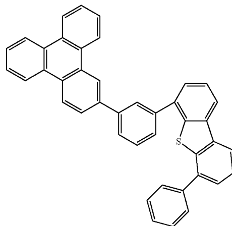
Compound 23S
