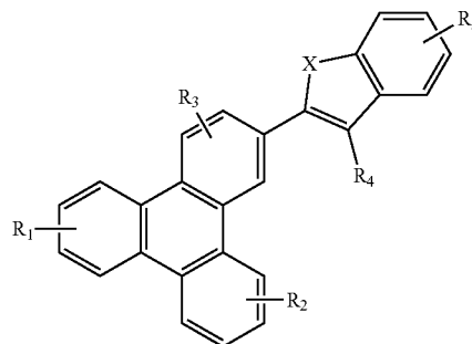
Compound 14G
