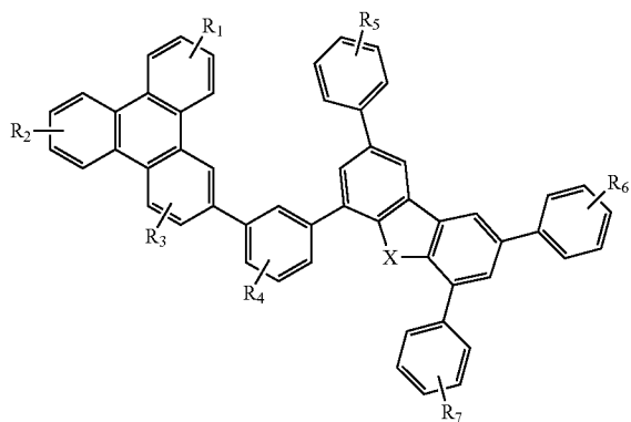
Compound 25 G
