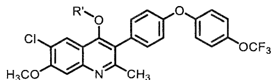
Formula (II)
