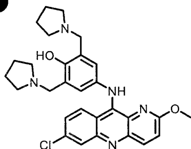
pyronaridine (4-[(7-chloro-2-methoxy-pyrido[3,2-b]quinolin-10-yl)amino]-
