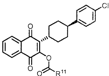
Formula (III)
