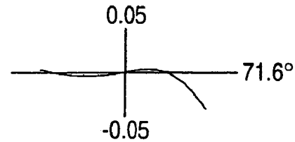
COMMA ABERRATION (mm)
