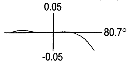
COMMA ABERRATION (mm)
