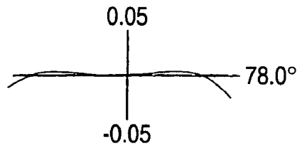
COMMA ABERRATION (mm)
