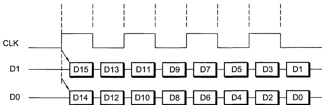
DETAILED VIEW OF THE READ DATA
