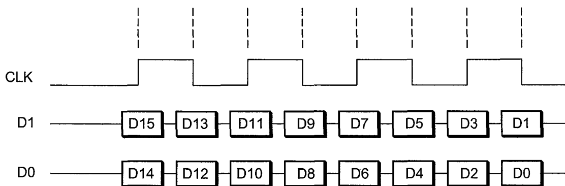
DETAILED VIEW OF THE WRITE DATA
