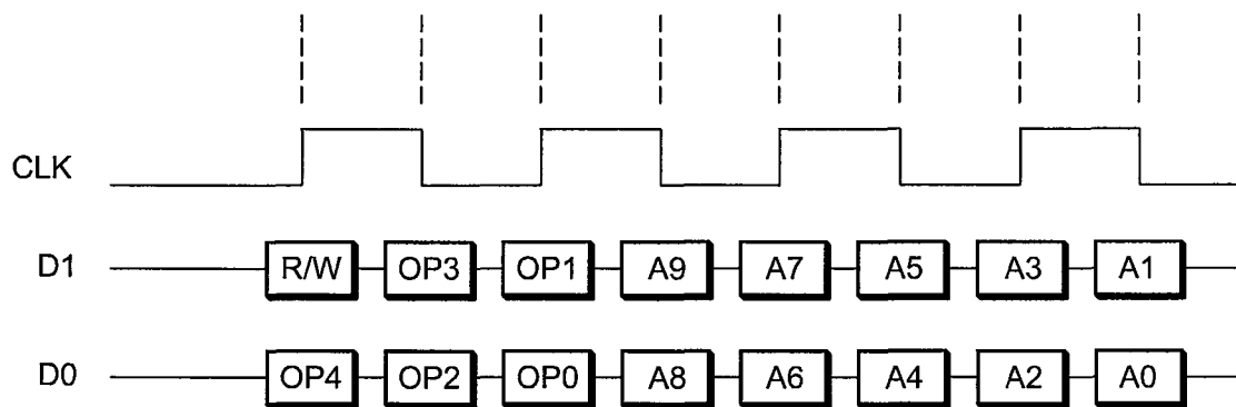
DETAILED VIEW OF THE FIRST 4 CLOCKS
