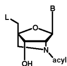
2'-(acylamino)-LNA
