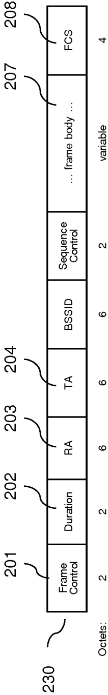
Figure 2g : MAC frame format
