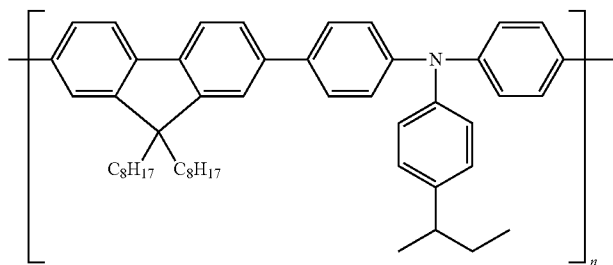
[Chemical formula 6]
