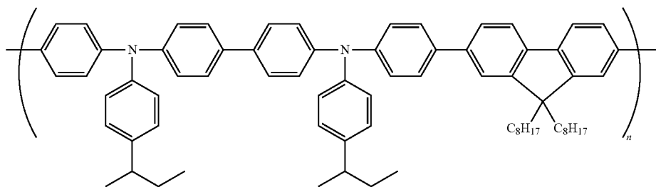
[Chemical formula 7]
