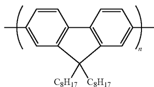
[Chemical formula 7]
