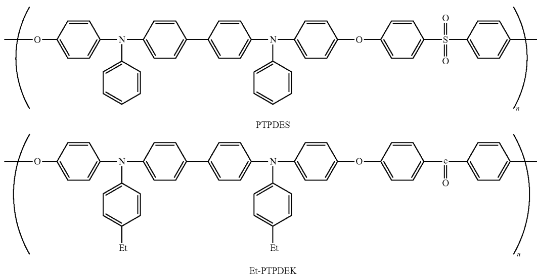
[Chemical formula 3]
