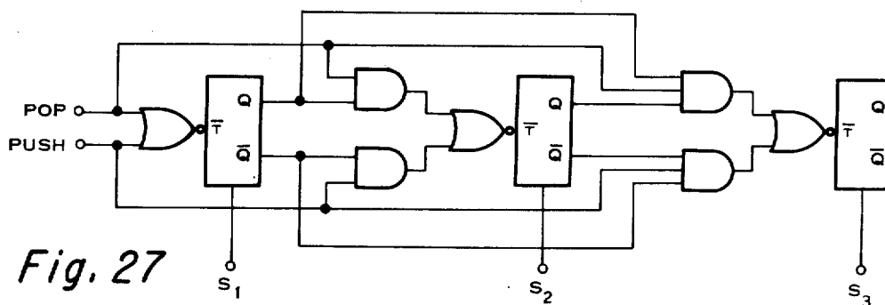
STACK POINTER
