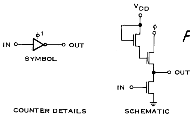
SCHEMATIC
