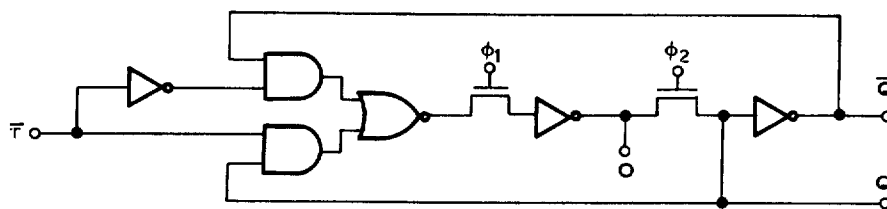
FLIP-FLOP LOGIC
