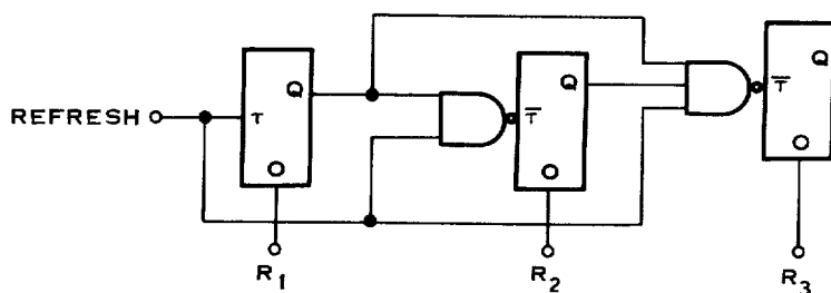
REFRESH COUNTER
