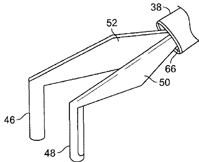
FIG. 6 (Prior Art)
