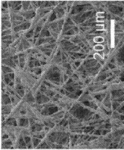
HSSN anode after 5 cycles
