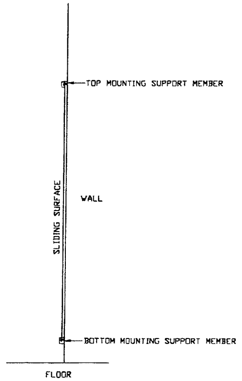
SIDE VIEW fig 5
