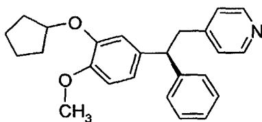
CT-1731
