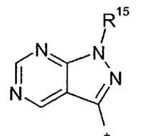
1H-pyrazolo[3,4-d]- pyrimidinyl (5.0.23)
