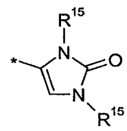
Imidazolidin-2-on-4-yl
