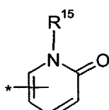
2-pyridonyl
