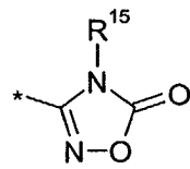
1,2,4-oxadiazol- 5-on-3-yl
