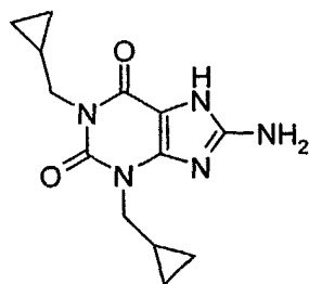
Cipamfylline (BRL-61,063)
