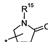
pyrrolidonyl (1.1.30)
