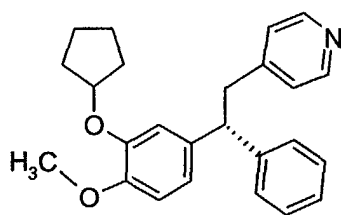
CDP840 (0.0.9)
