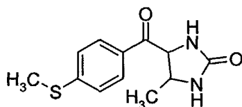
Enoximone (0.0.10)
