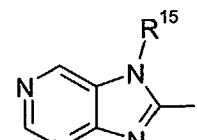
1H-purinyl (5.0.28)
