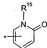
2-pyridonyl
