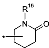
2-piperidonyl (1.1.31)
