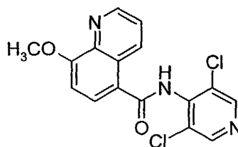
D4418
