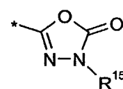
1,3,4-oxadiazol-2-on-5-yl (1.1.19)
