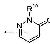
pyridazin-3-onyl
