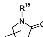
pyrrolidonyl
