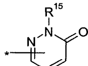
pyridazin-3-onyl
