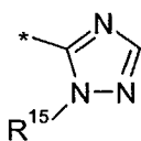
1,2,4-triazol-3-yl (1.1.12)
