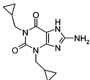
Cipamfylline
