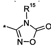
1,2,4-oxadiazol-5-on-3-yl
