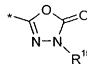
1,3,4-oxadiazol-2-on-5-yl (1.1.19)
