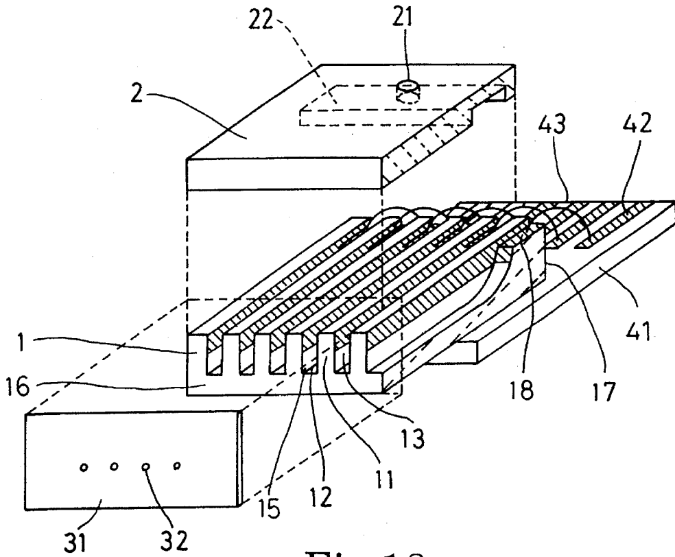
Fig.18 PRIOR ART
