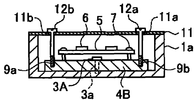
B-B CROSS SECTION
