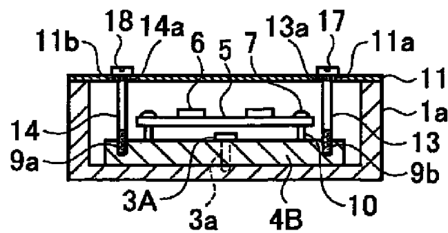
B-B CROSS SECTION
