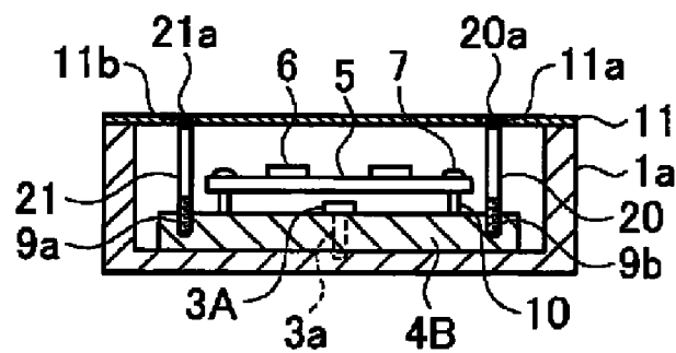
B-B CROSS SECTION
