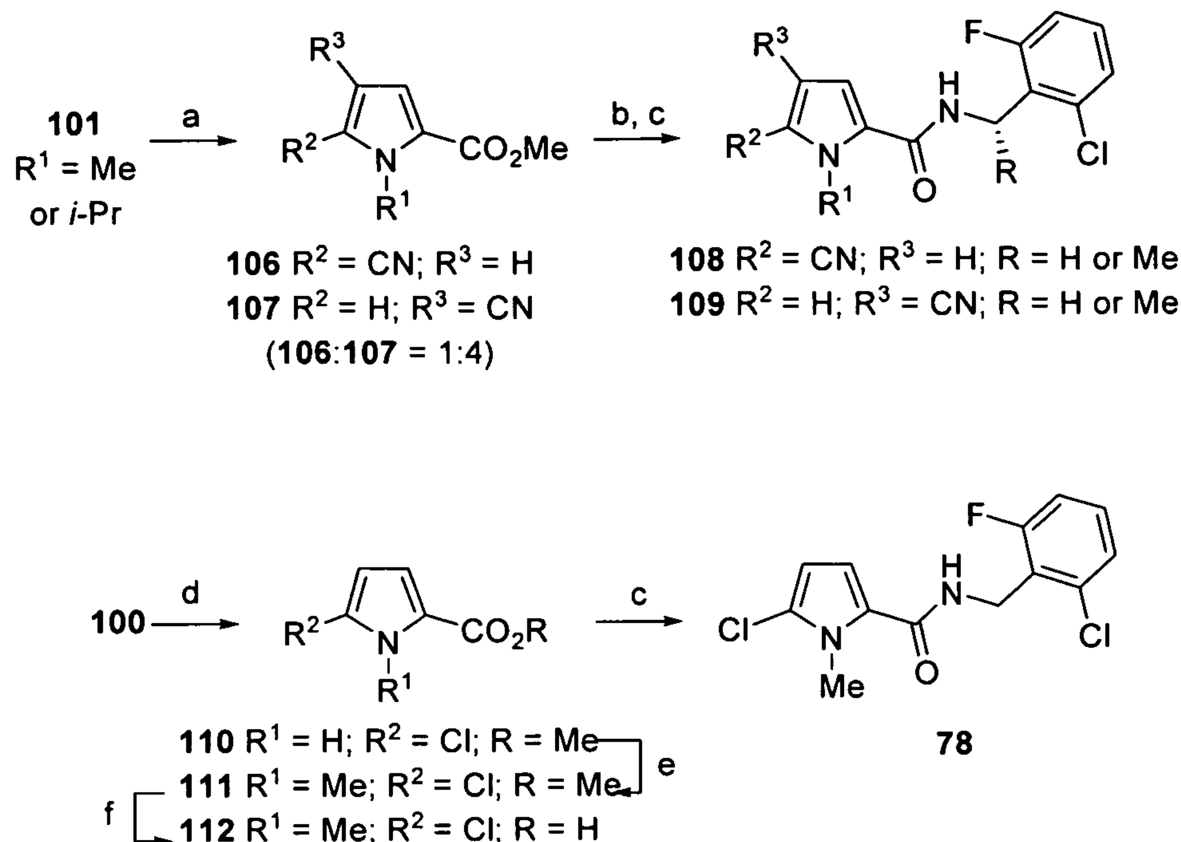
Scheme 6
