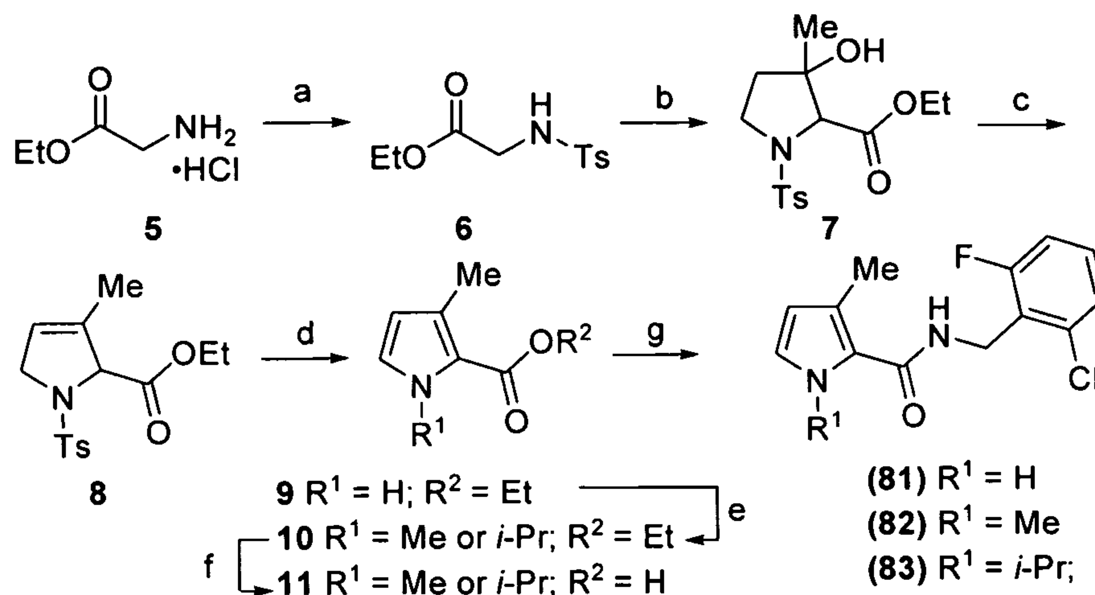
Scheme 4
