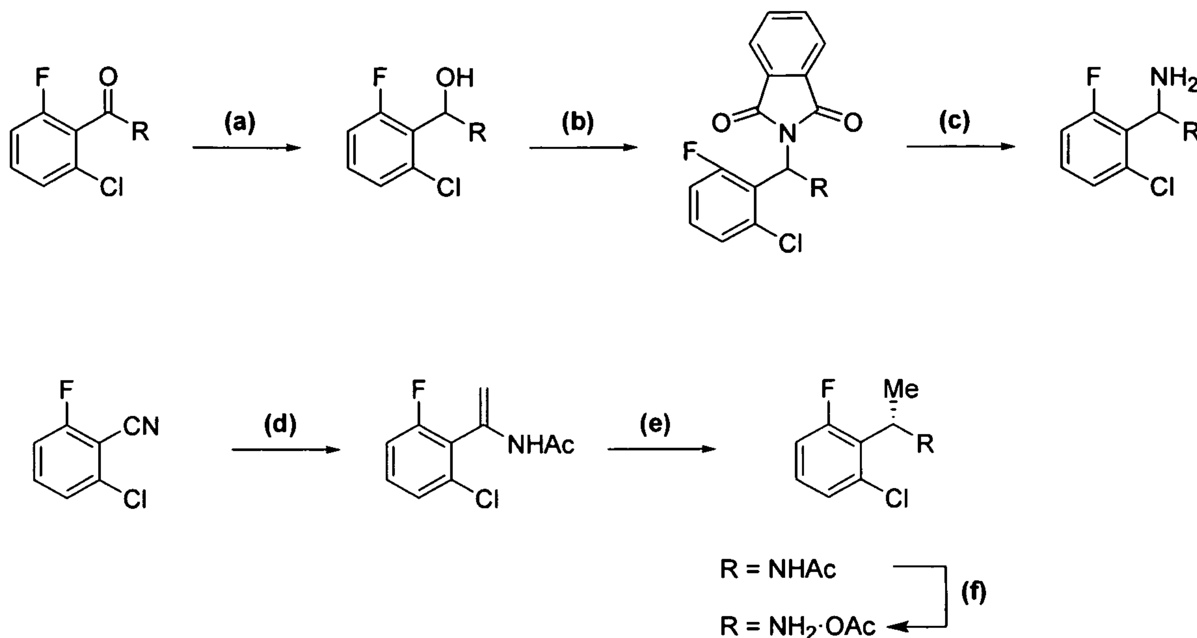
Scheme 3
