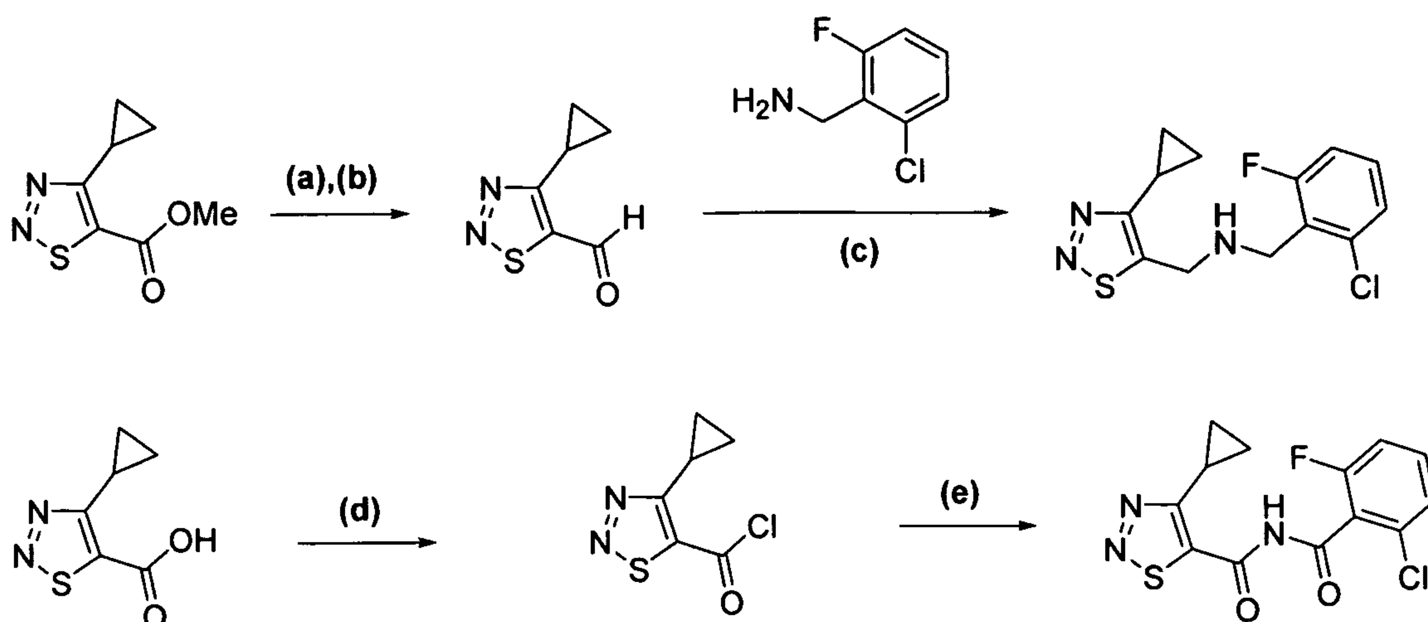
Scheme 2
