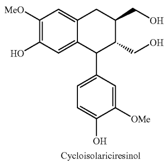
Figure 1 illustrates the different phenolic and polyphenolic compounds contained in the bark of betula pendula (birch tree).
