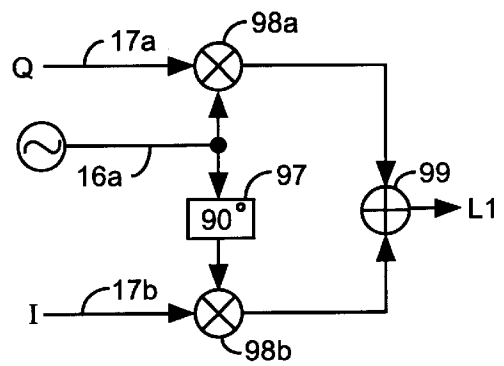
L1 QPSK Modulator (Prior Art)
