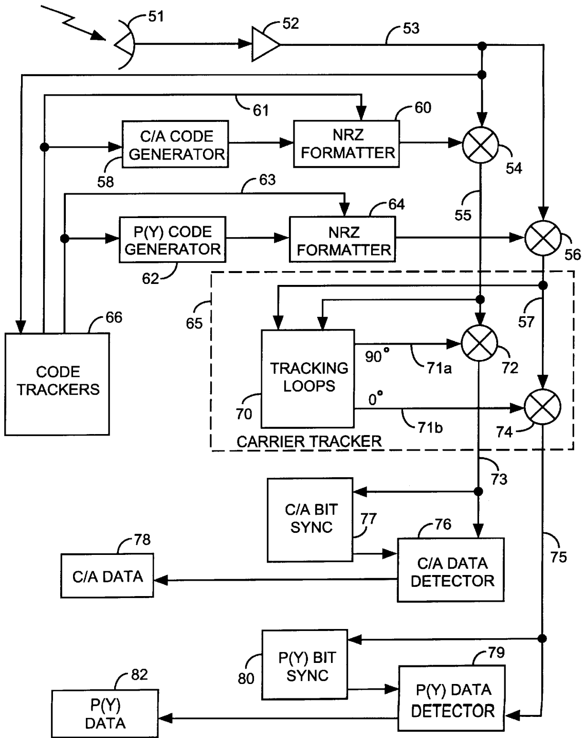
NRZ Formatted Quadrphase Modulated Receiver System (Prior Art)
