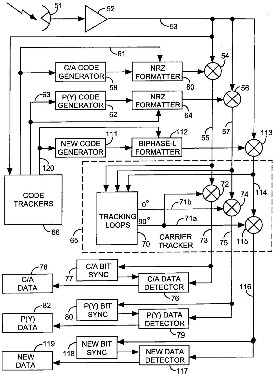
NRZ & Biphase-L Formatted Hexaphase Modulated Receiver System
