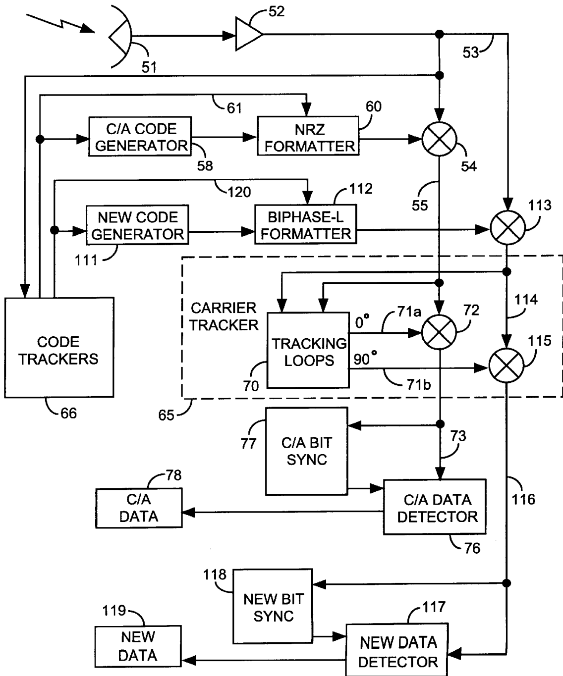
NRZ and Biphase-L Formatted Quadrphase Modulated Receiver System
