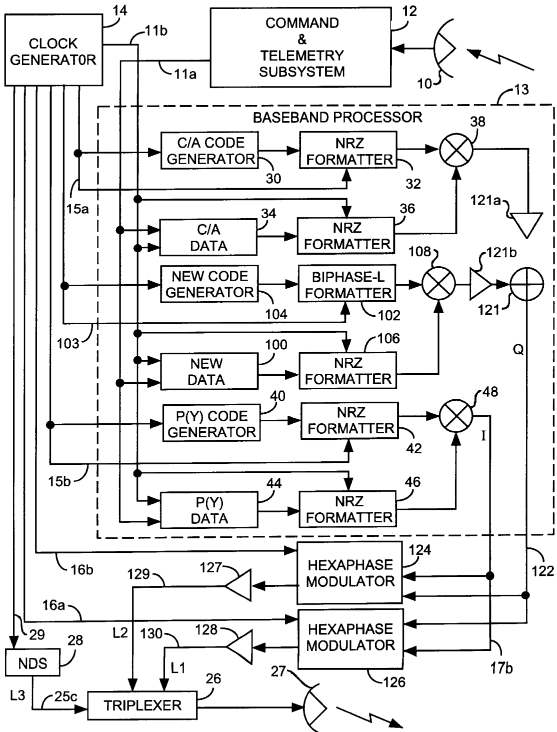
NRZ & Biphase-L Formatted Hexaphase Modulated Transmitter System
