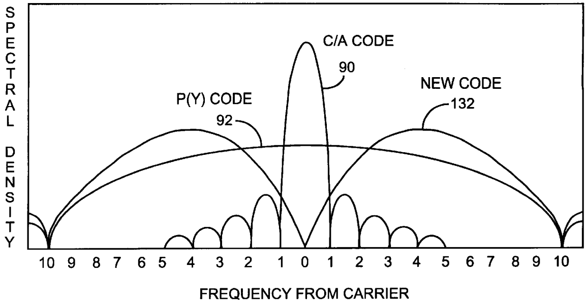
Code Spectral Density
