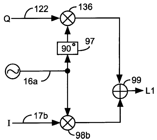
L1 Hexaphase Modulator
