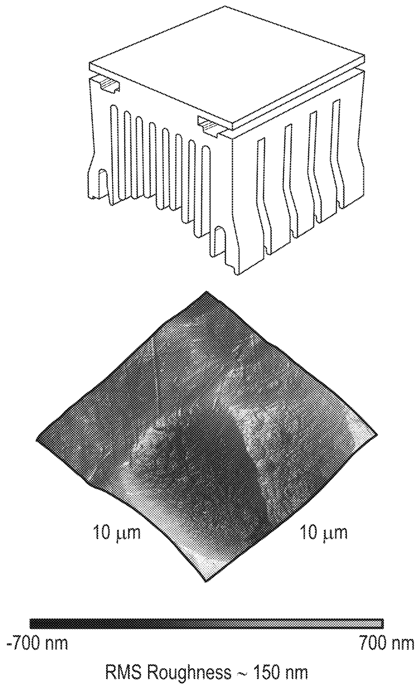
Copper Heat Sink
