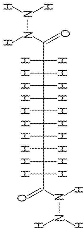
Dodecandioic dihydrazide FIGURE 20D
