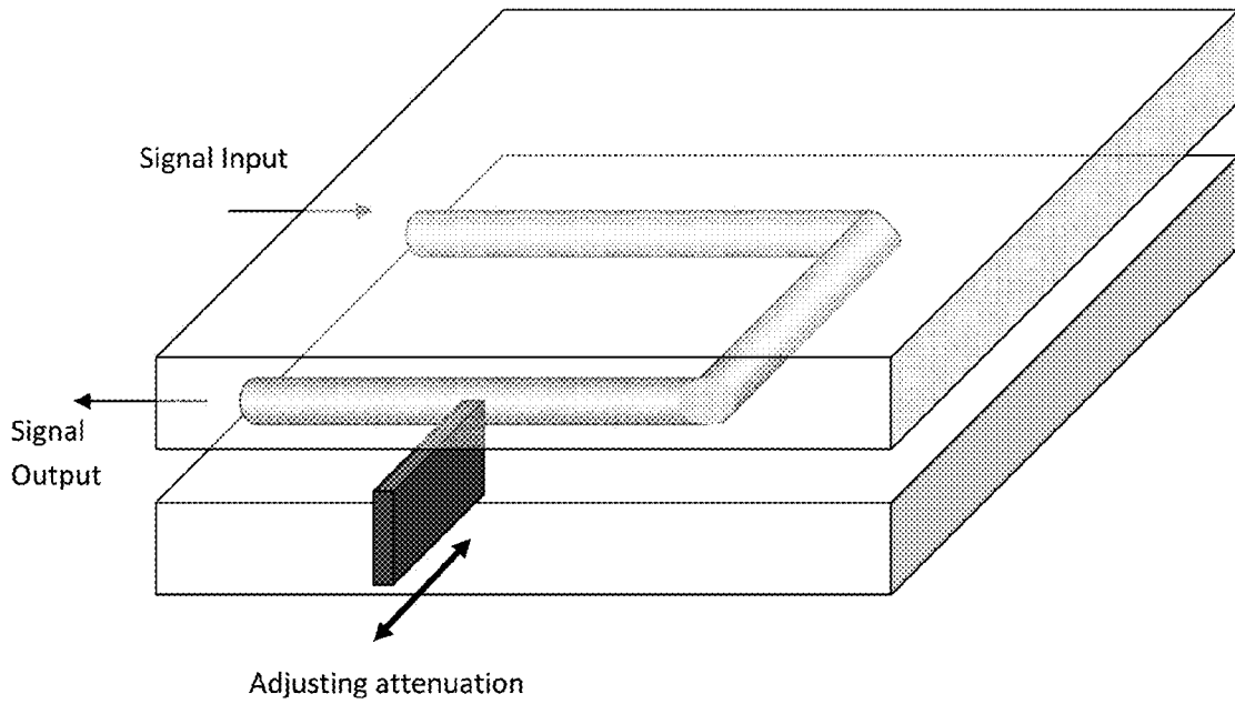
Figure 7: Variable attenuator in a slabline, version 2
