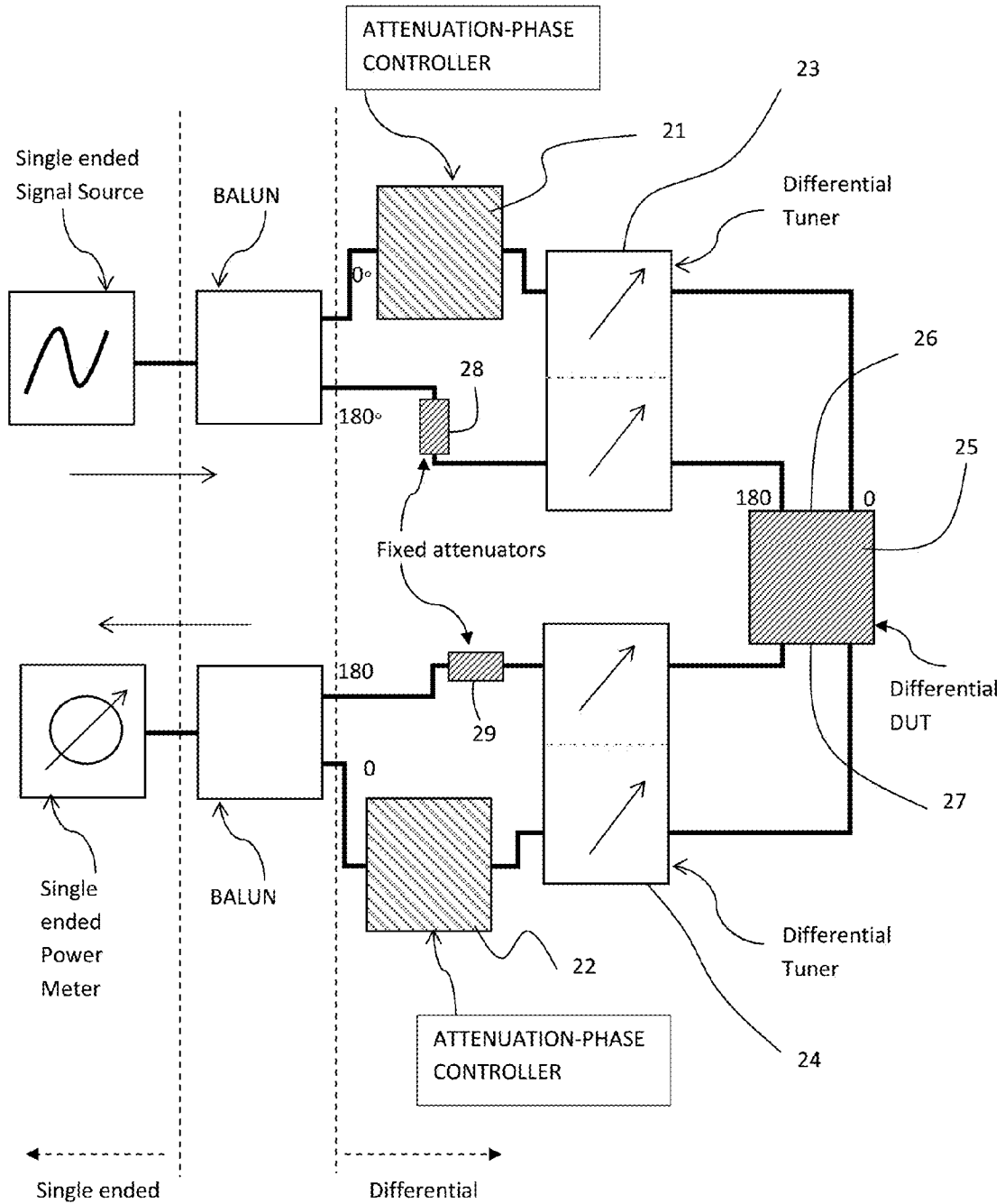
Figure 2: Partly prior art: Differential Load Pull System
