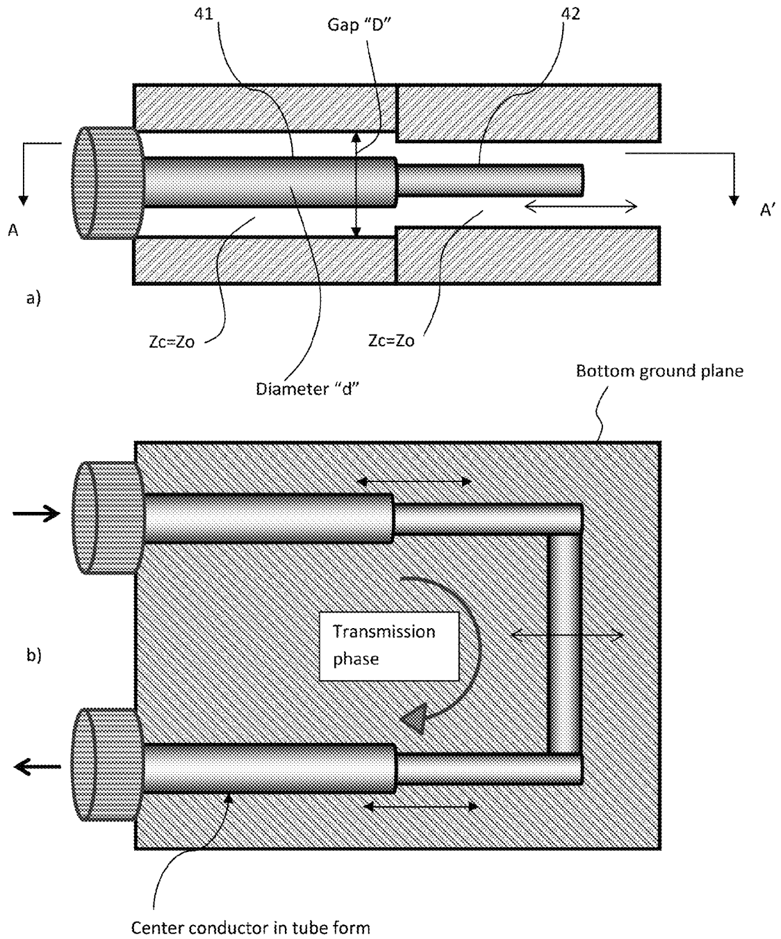
Figure 4: Prior art; linear phase shifter using slabline; a) side view, b) section A-A'
