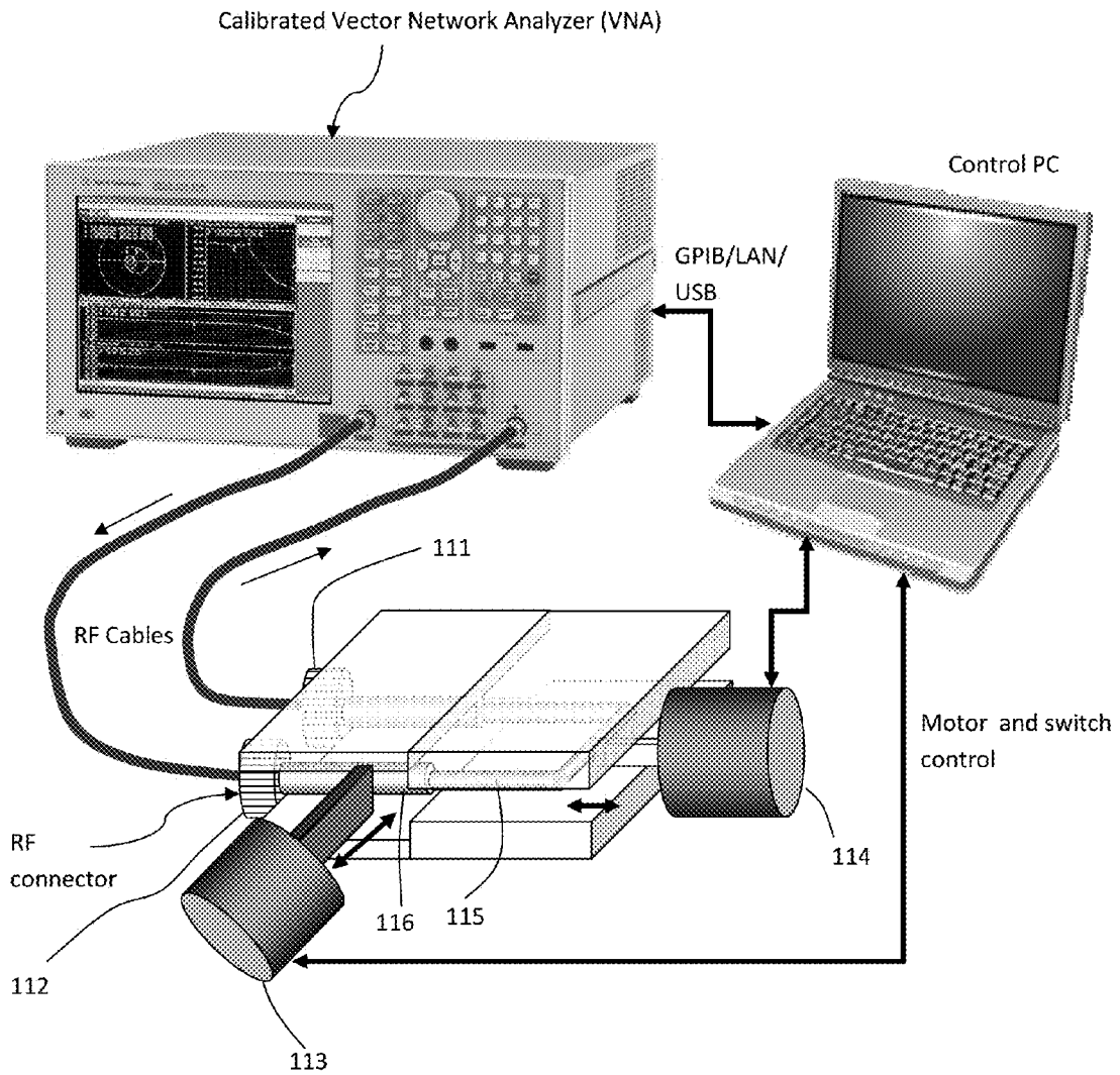
Figure 11: Calibration of VAPS using a pre-calibrated VNA
