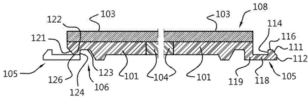
Fig. 17 Prior art
