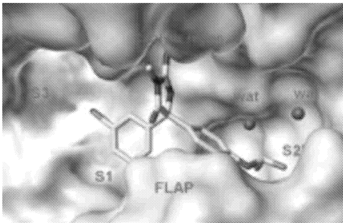
Compound 1A
