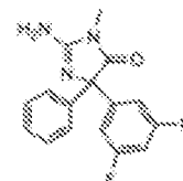
Compound 1B
