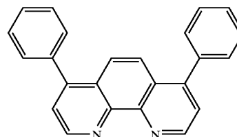
4,7-diphenyl-1,10-phenanthroline (Bphen)
