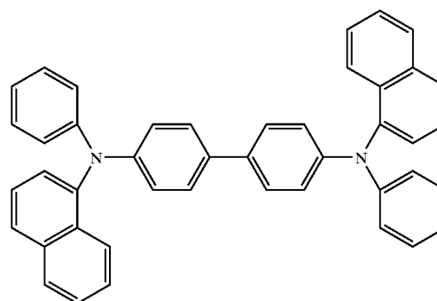
1,4-bis[(1-naphthylphenyl)-amino]biphenyl (NPD)
