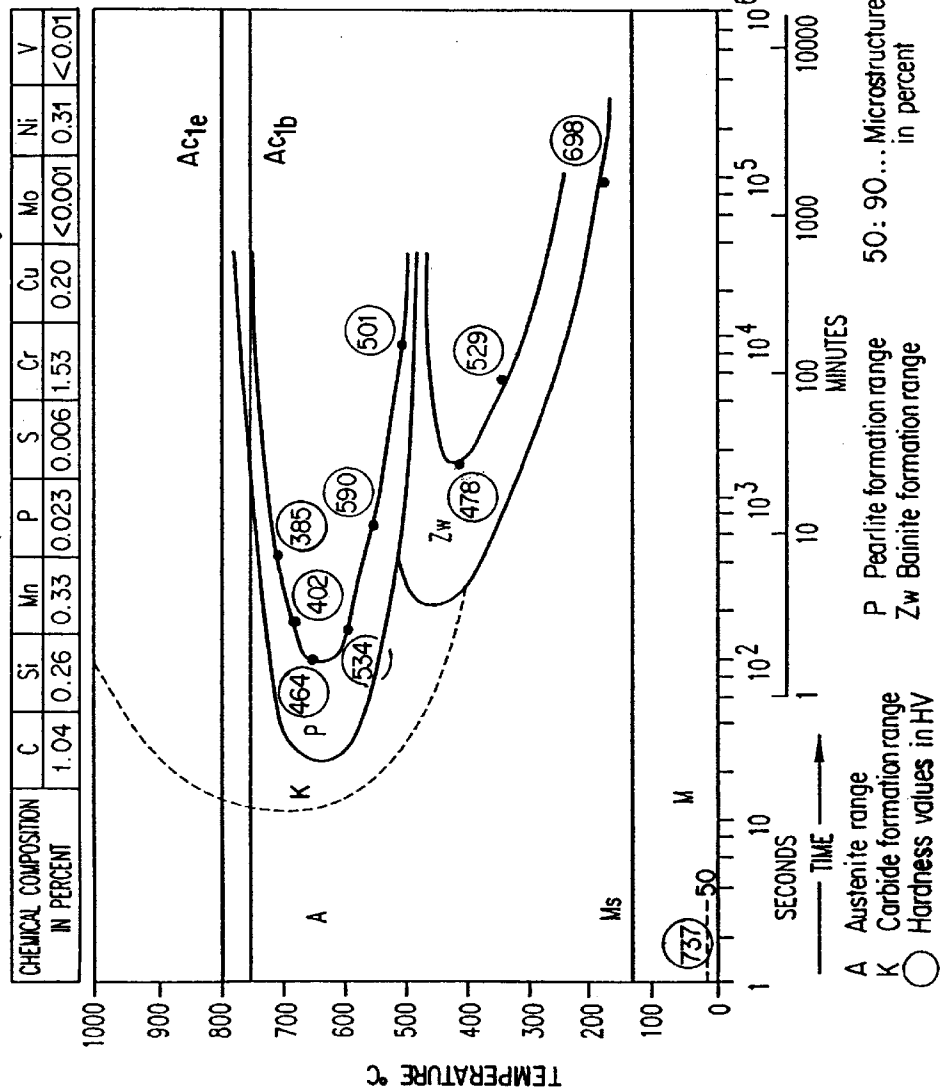
Steel 100 Cr 6 (Melt No 1) Time-Temperature-Transformation Diagram (Isothermic) II-225D
