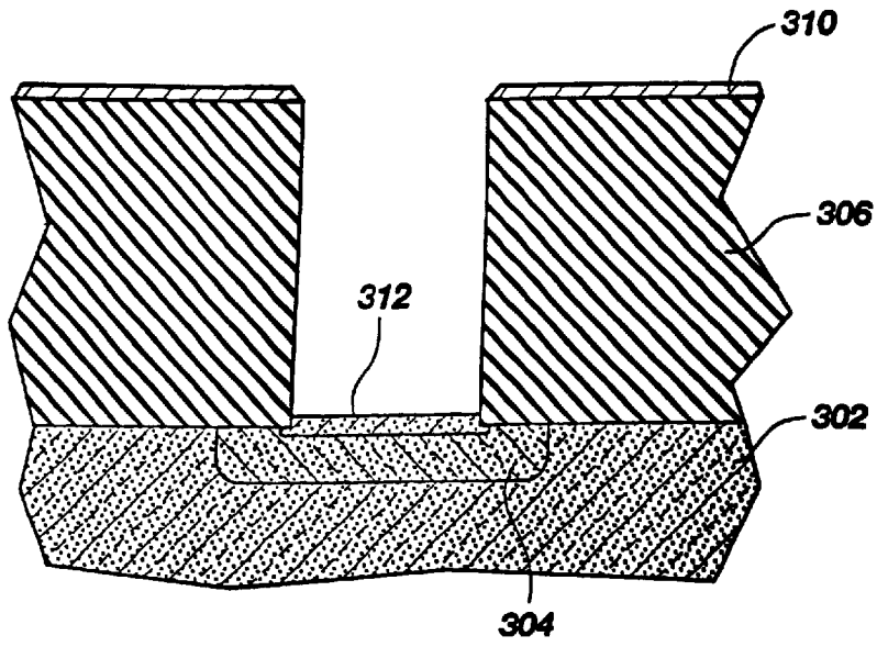
Fig. 17 (Prior Art)
