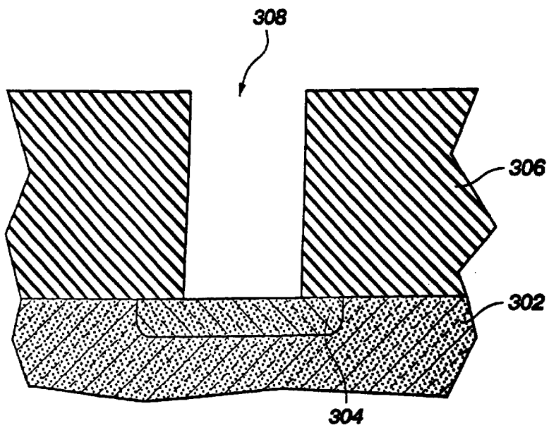
Fig. 15 (Prior Art)
