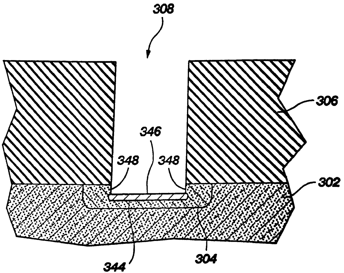
Fig. 21 (Prior Art)
