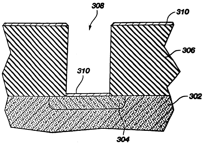
Fig. 16 (Prior Art)
