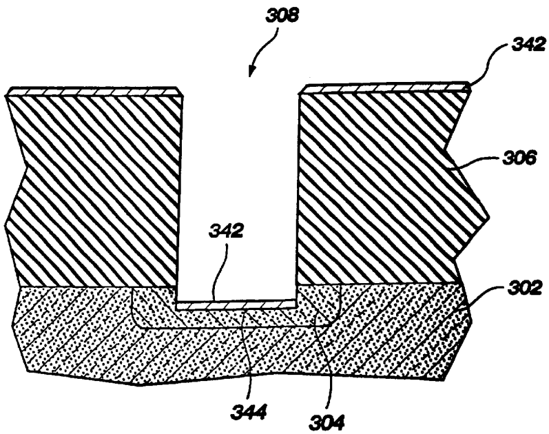
Fig. 20 (Prior Art)
