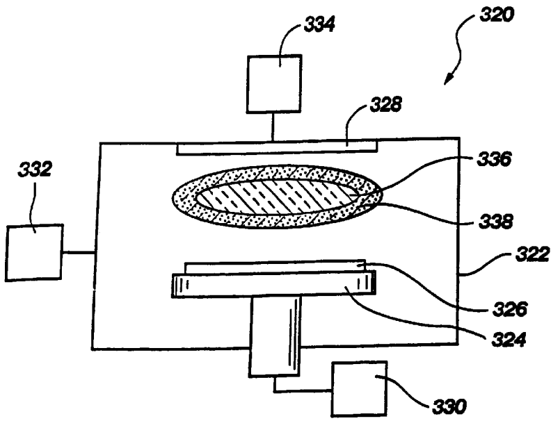
Fig. 19 (Prior Art)
